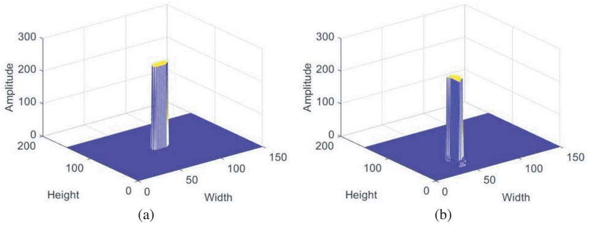
Figure 6. Saliency representation I_G of SAR images. (a) Fig. 2(a). (b) Fig. 2(b).
