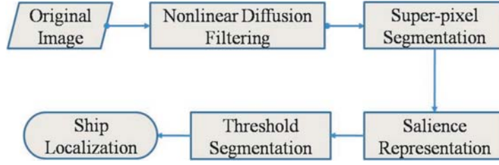
Figure 1. Processing strategy for ship detection in SAR images.
