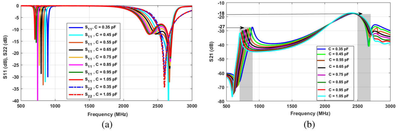
Figure 13. (a) Simulated reflection coefficients of the MIMO system, (b) simulated mutual coupling of the MIMO system.
