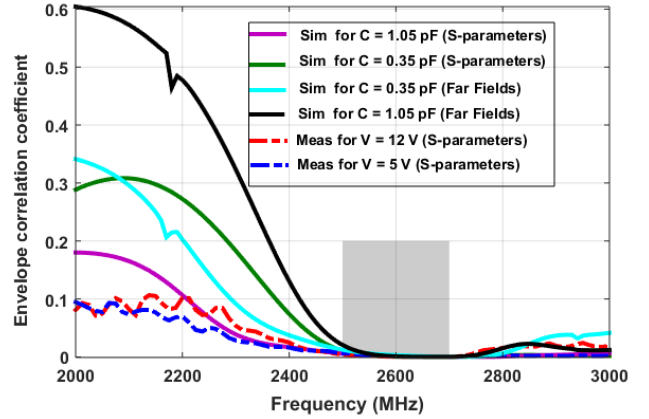
Figure 18. Simulation and measurement of the envelope correlation coefficient.
