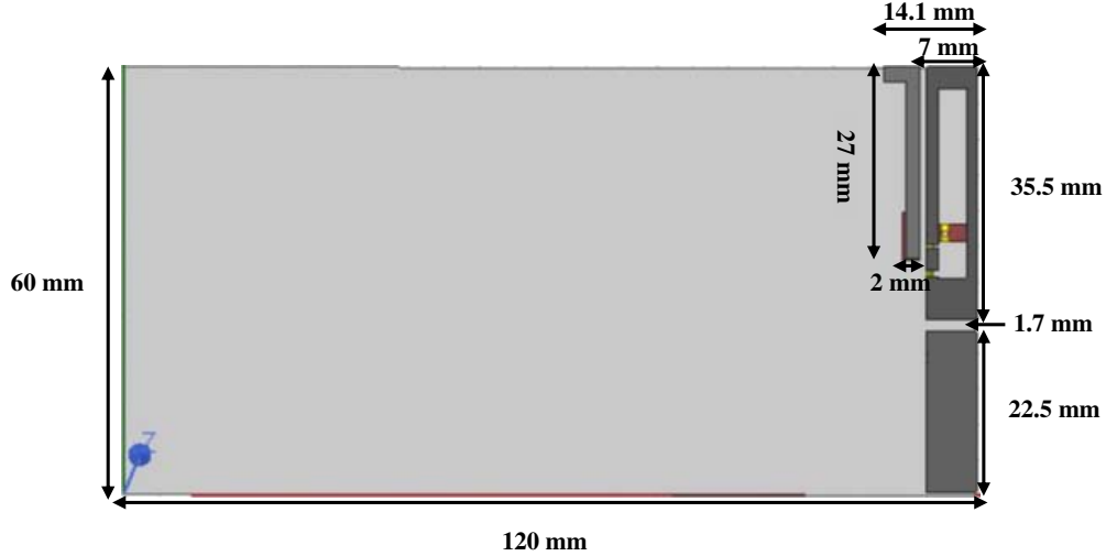
Figure 1. Overall view of the proposed antenna system.
