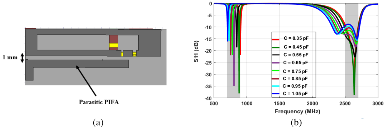
Figure 10. (a) Structure of the active dual-band reconfigurable PIFA, (b) simulation of S_{11} (dB) of the dual-band antenna for C varying from 0.35 pF to 1.05 pF.
