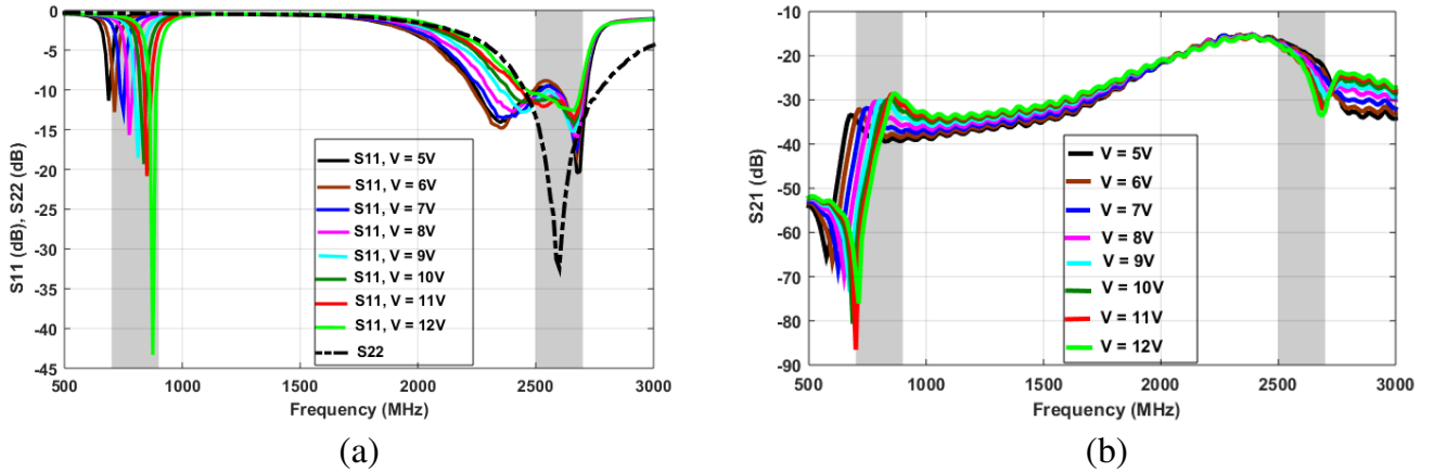
Figure 15. (a) Measured S_{11} and S_{22} of the MIMO system for different DC values, (b) measured S_{21} of the MIMO system for different DC values.
