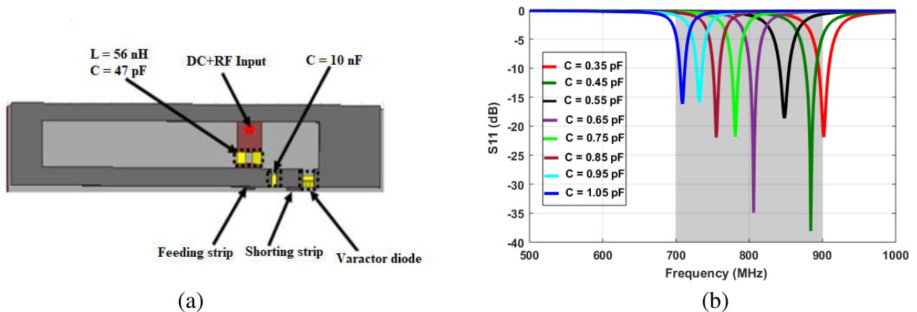
Figure 8. (a) Structure of the active reconfigurable PIFA, (b) simulation of reflection coefficient for C varying from 0.35 pF to 1.05 pF.
