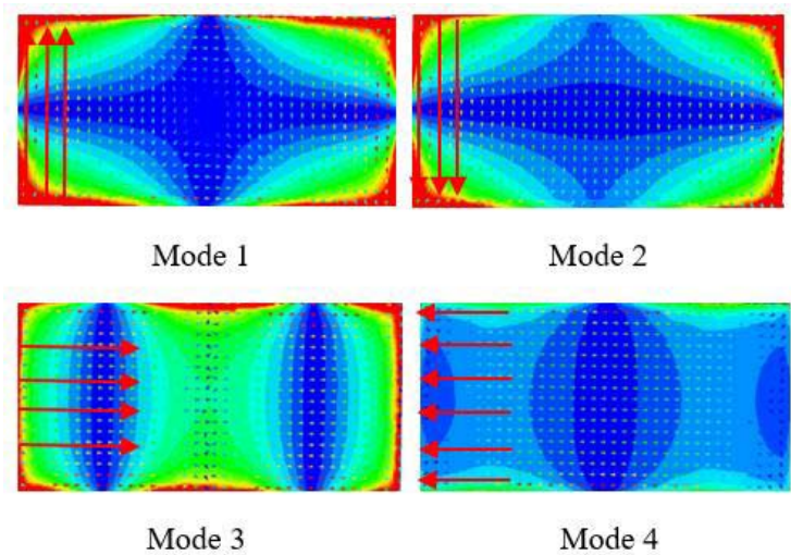
Figure 3. Electric field and surface current vector over the chassis at 2.6 GHz.
