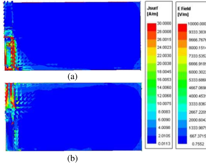
Figure 12. Visualization of the electric field ( E field) and the surface current vector ( J_{surf} ) over the MIMO structure at 2.6 GHz when exciting (a) antenna 1 and (b) antenna 2.
