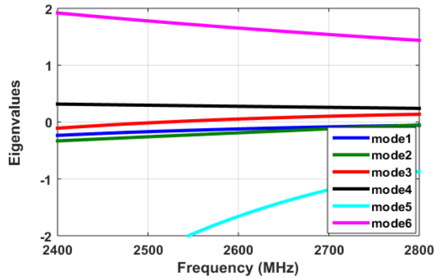
Figure 2. Simulation of the eigenvalues of the mobile phone chassis.
