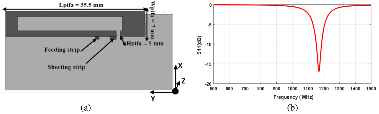
Figure 4. (a) Initial meandered PIFA, (b) simulation of S_{11} of the meandered PIFA.
