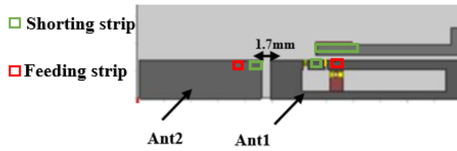
Figure 11. Structure of the MIMO system.
