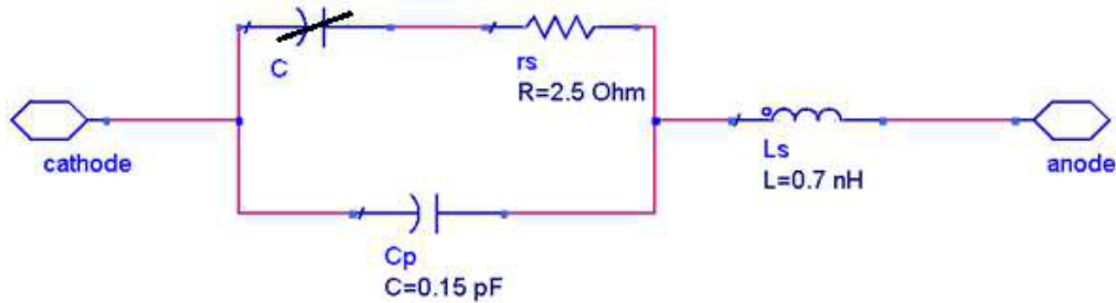
Figure 5. The varactor diode equivalent circuit.
