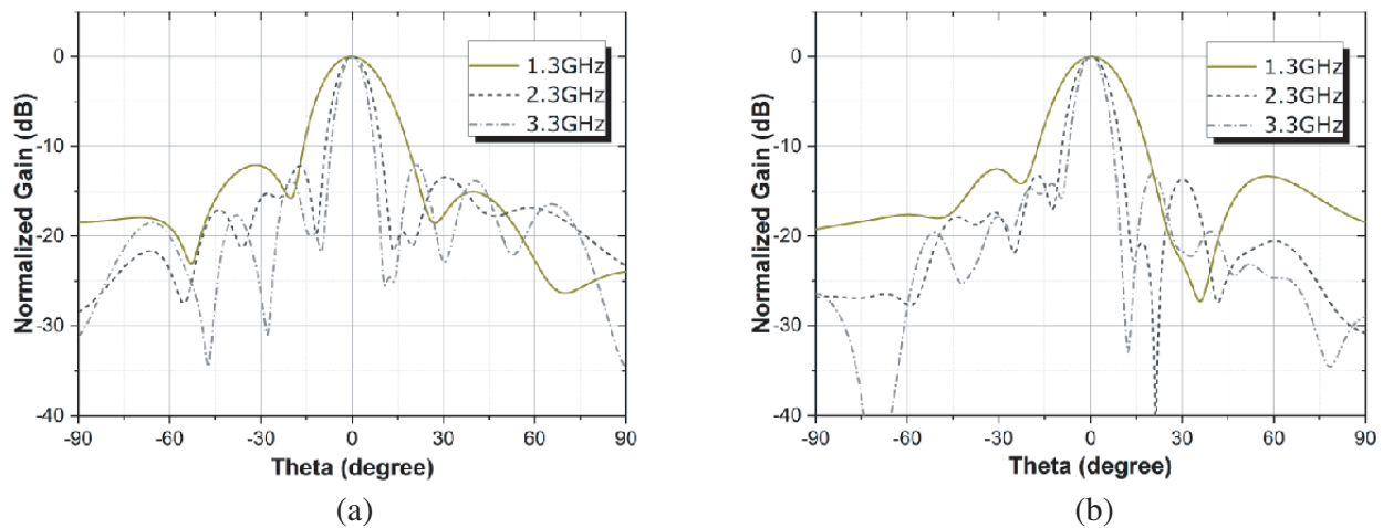
Figure 8. Measured radiation patterns of the array prototype at 1.3, 2.3 and 3.3 GHz in (a) E -plane, and (b) H -plane.
