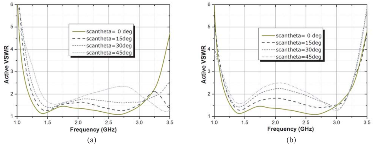
Figure 7. Measured active VSWR when the array antenna scans in (a) E -plane, and (b) H -plane.
