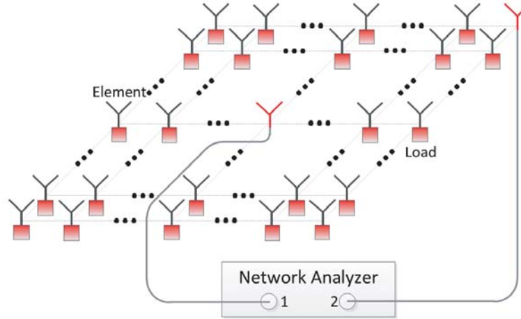
Figure 6. Functional diagram of the measuring method for the active VSWR of the centre element in an array antenna.
