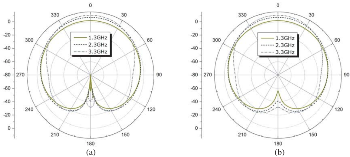
Figure 5. Simulated radiation patterns of the antenna element at 1.3, 2.3, and 3.3 GHz in (a) E -plane, (b) and H -plane.
