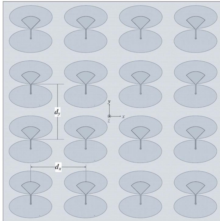
Figure 2. Layout of the 16-element ( 4 \times 4 ) subarray antenna. The element spacing dx = dy = 60 mm.
