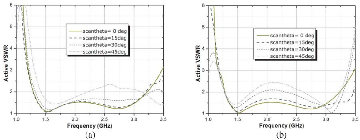
Figure 4. Simulated active VSWR when the array antenna scans in (a) E -plane, and (b) H -plane.
