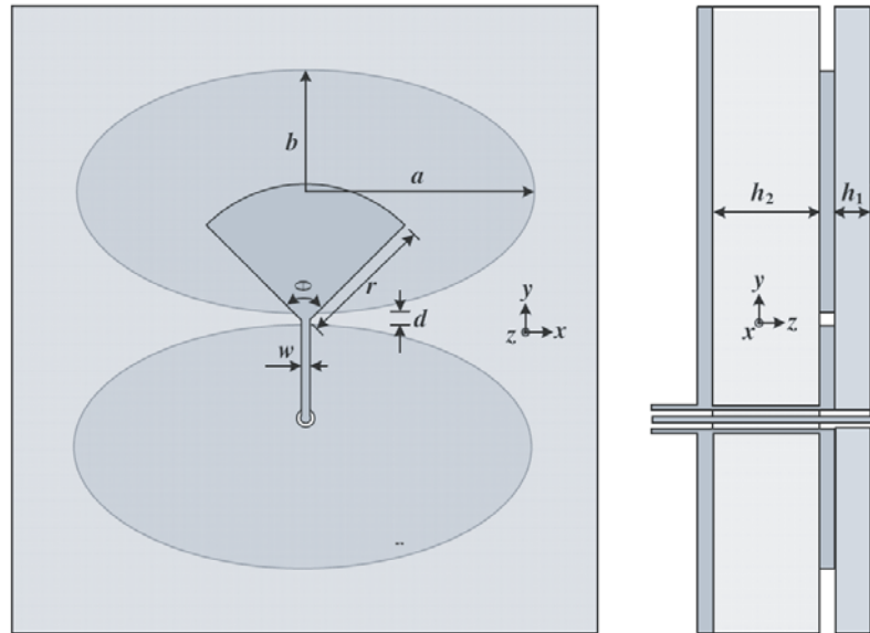
Figure 1. Geometry of the planar dipole antenna which acts as an array element. (a) Front view. (b) Side view.
