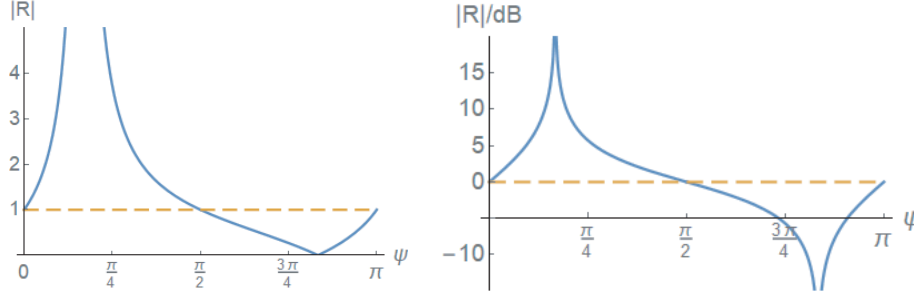
Figure 2. The magnitude of the reflection coefficient |R| (absolute and logarithmic) for a plane wave incident to a planar self-dual EH boundary defined by a real vector \mathbf{a} which forms the angle \pi/3 with the normal of the boundary. Solid blue line: \mathbf{k}^i lies in the plane parallel to the vectors \mathbf{n} and \mathbf{a} and makes the angle \psi with the boundary (see Figure 1). Matched wave conditions appear for \psi = 5\pi/6 (matched incident wave) and for \psi = \pi/6 (matched reflected wave). Dashed orange line: the reflection coefficient is |R| = 1 for all incidence angles in the plane parallel to vectors \mathbf{n} and \mathbf{n} \times \mathbf{a} . The value |R| is independent of the polarization of the wave in both cases.
