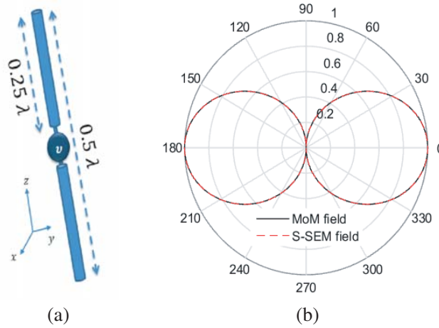
Figure 3. (a) The symmetric half-wavelength wire system that is used in the learning phase and (b) its far-field polar representation in comparison to a MoM computation [22].
