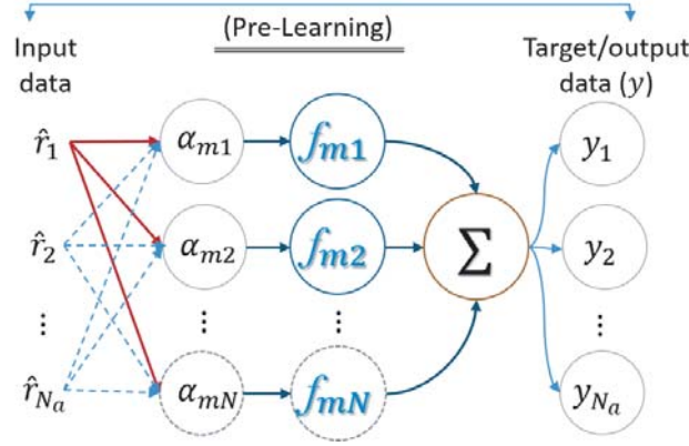
Figure 2. The m th current segment's pre-learning architecture of the S-SEM-NN with N_a nodes, where N_a is the number of field points. The NN accepts input data (angles) and produces target output data (complex far fields.) Here, the S-SEM s_{mn} poles (not shown in the figure but see (2) for details) will be part of the internal training parameters of each activation function f_{mn} of each neuron (nonlinear training parameters), while the corresponding strengths \alpha_{mn} are linear weights post-multiplied by the output of each neuron. The input data points are the measured far-field angles \theta and \phi (features), while the output of the NN is the real and imaginary parts of the fields ( \theta - and \phi -components).
