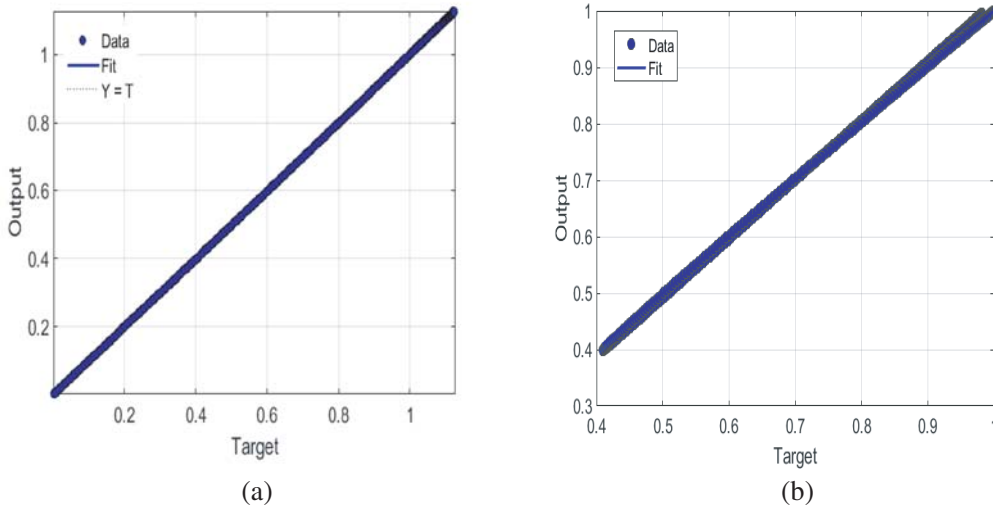
Figure 7. Regression analysis plot (a) symmetric wire (b) L-shape wire.
