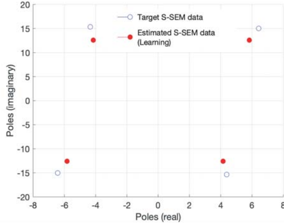
Figure 4. A comparison of the estimated S-SEM data and the actual ones obtained from a direct method (MoM or measurement) of the symmetric wire. Here, the MoM code WIPL-D [22] is used to generate test f_{mn} data.
