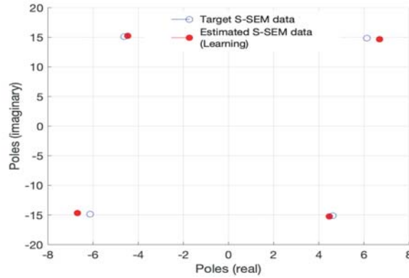
Figure 6. A comparison of the complex plot of the estimated S-SEM data and the actual ones obtained from an EM solver of the L-shaped wire.
