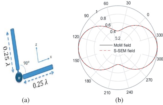
Figure 5. (a) The L-shape wire system used in the learning phase and (b) its far-field polar representation in comparison to an EM solver.
