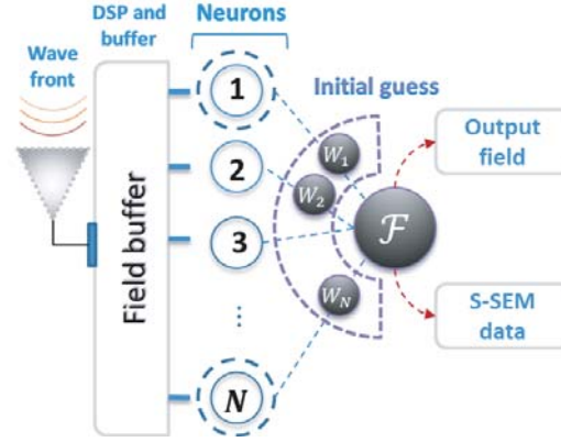
Figure 1. Proposed Inverse Source Modeling System based on the S-SEM neural network.
