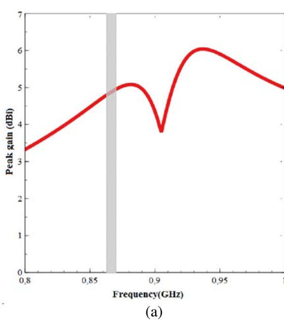
Figure 13. Simulated peak gain of the two-element array: (a) for Z_L = 5.6 pF, (b) for Z_L = 33 nH.
