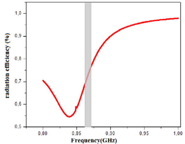
Figure 7. Simulated radiation efficiency of the proposed structure.
