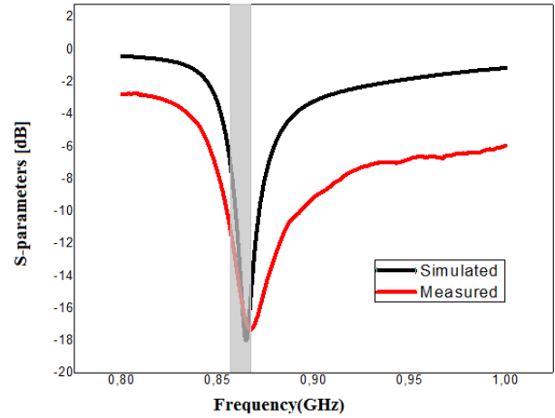
Figure 15. Simulated and measured return loss for Z_L = 5.6 pF.
