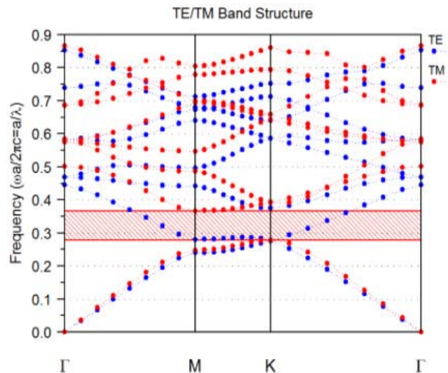
Figure 1. Photonic band gap of the designed sensor.
