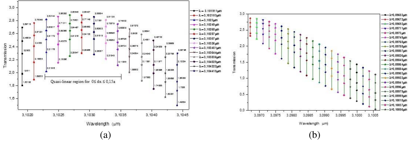
Figure 5. Sensor output spectrum for various displacements with Sx = 0.335D and, (a) for Sy = 0 , (b) for Sy = 0.05D .
