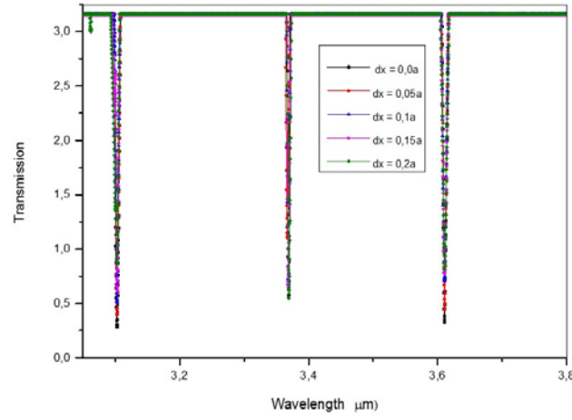
Figure 3. Response of the micro displacement sensor as a function of wavelength for various displacements \Delta x ( dx in Figure 3).
