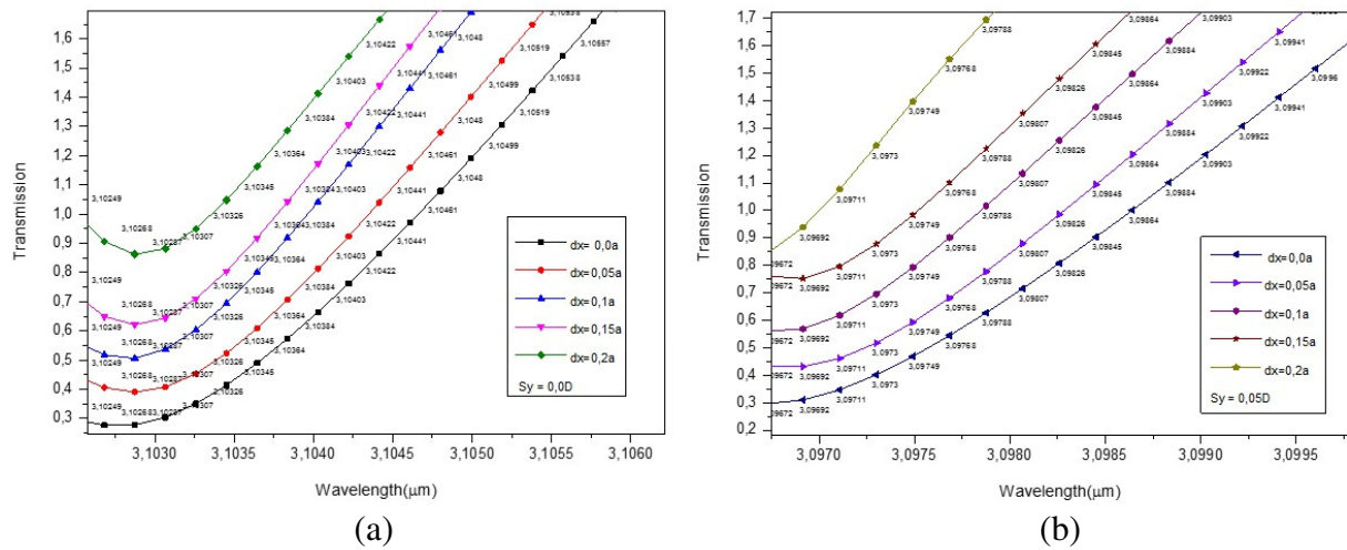
Figure 4. Sensor response for various displacements with S_x = 0.335D and: (a) For S_y = 0 and (b) for S_y = 0.05D .
