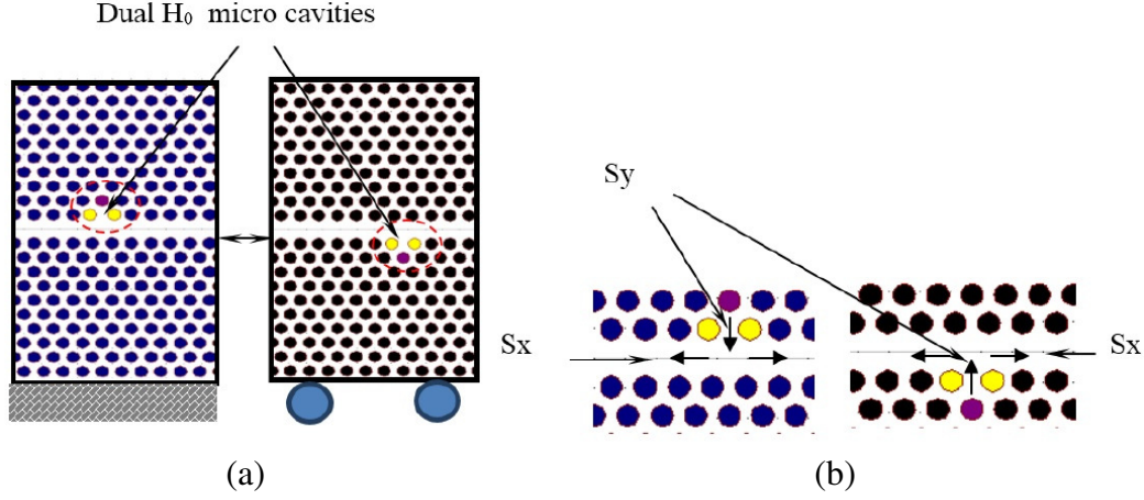
Figure 2. (a) Proposed design for the micro displacement sensor, (b) optimizations process.
