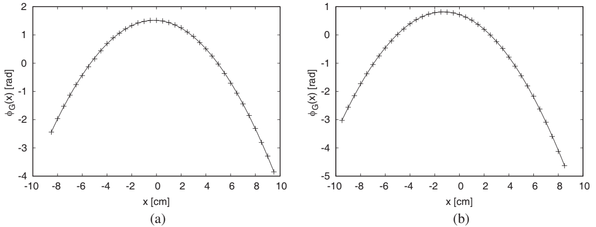
Figure 5. Phase profiles of the radiation beam on axis ((a) y = 0 ) and at y_0 = 35 mm from the propagation axis (b) measured after removing the SPP. Black solid lines are the curves fitted to data.
