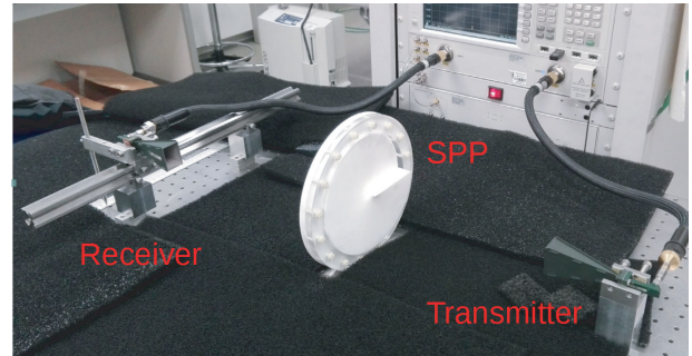
Figure 2. (a) Geometry of the experimental setup. The scan has been performed in the horizontal x direction through a linear translation stage positioned at two different vertical positions from the singularity. (b) Picture of the experimental setup.
