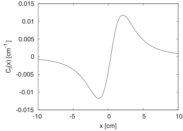
Figure 7. Transverse curvature of the helicoidal wavefront C_I(x) calculated from the fit function of data in Fig. 6(b).
