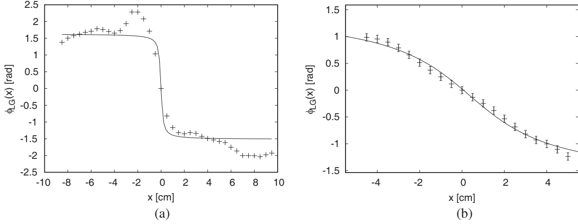
Figure 6. Phase profiles of the phase difference \phi_{LG} = \phi - \phi_G on axis ((a) y = 0 ) and at y_0 = 35 mm from the singularity (b). Here \phi is the dataset in Fig. 4 and \phi_G is the best fit in Fig. 5. Black solid lines are the curves fitted to data.
