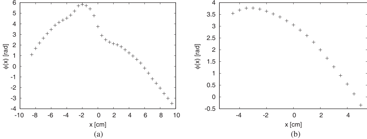
Figure 4. Phase profiles of the radiation beam with screw phase dislocation ( l = 1 ) generated with the SPP and measured on axis ((a) y = 0 ) and at y_0 = 35 mm from the singularity (b).
