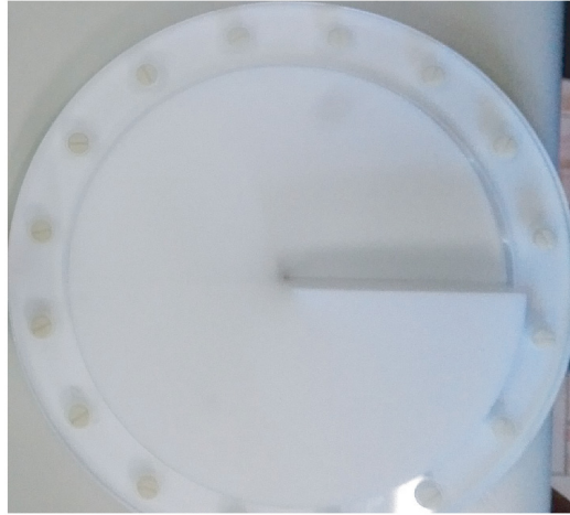
Figure 1. Picture of the SPP used to generate the radio-vortex.
