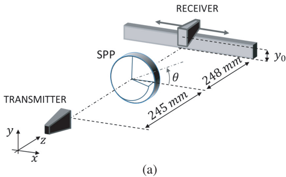
Figure 2. (a) Geometry of the experimental setup. The scan has been performed in the horizontal x direction through a linear translation stage positioned at two different vertical positions from the singularity. (b) Picture of the experimental setup.
