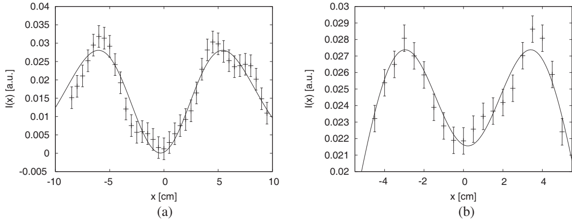
Figure 3. Intensity profiles of the Gaussian beam with screw phase dislocation on axis ((a) y = 0 ) and at y_0 = 35 mm from the singularity (b). Black solid line indicates the theoretical fit of a l = 1 Laguerre-Gauss mode. Error bars are the statistical errors extracted from the theoretical fits.
