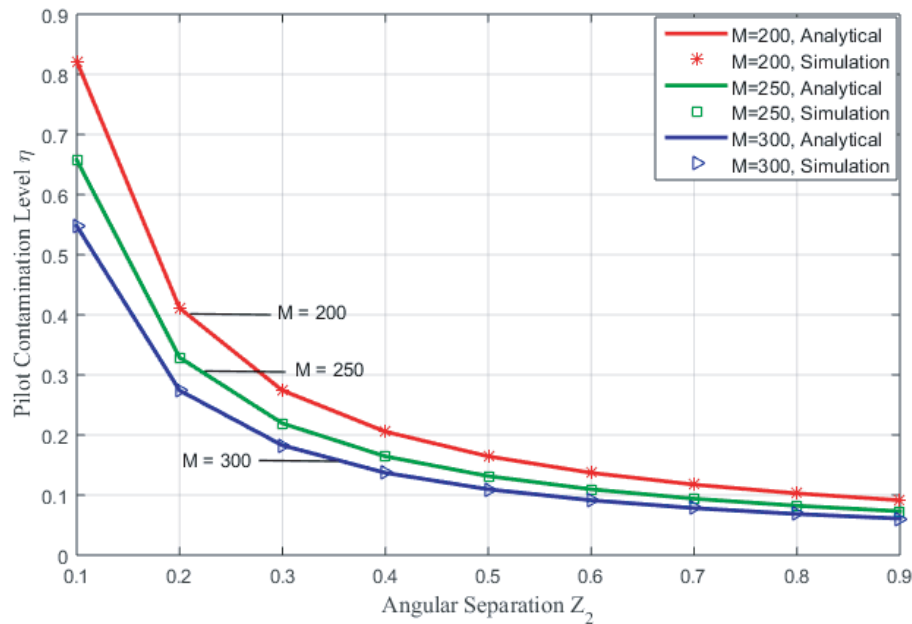
Figure 4. Pilot contamination versus angular separation Z_2 .
