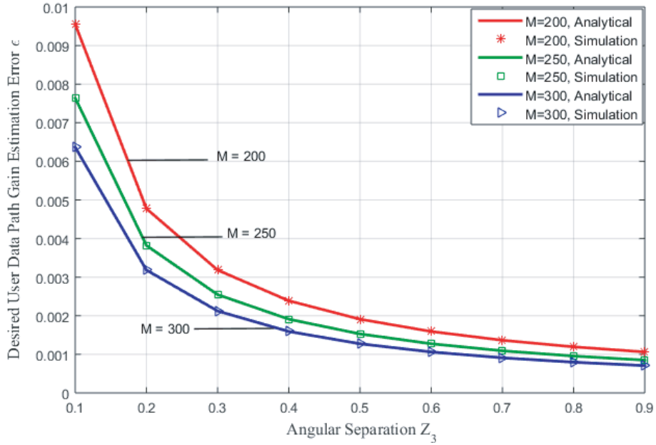
Figure 5. Desired user's data path gain estimation error versus angular separation Z_3 .
