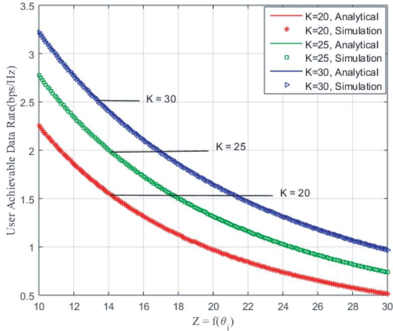
Figure 6. User's achievable data rate versus angular separation function Z = f(\theta_i) .
