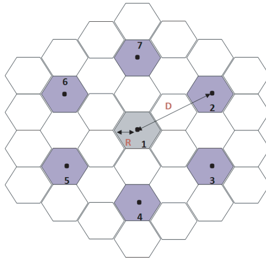
Figure 1. Illustration of first tier of copilot cells.
