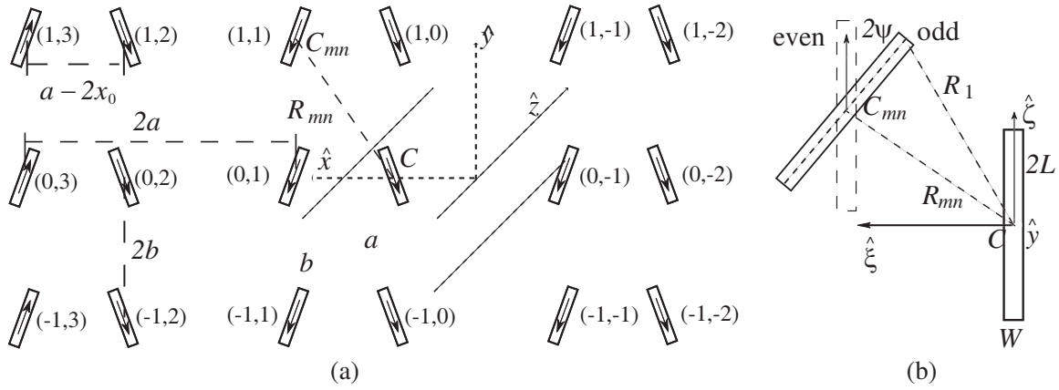
Figure 2. Image representation of a waveguide fed compound slot and geometry for mutual admittance evaluation. (a) Equivalent image representation of the slot. (b) Geometry for the evaluation of mutual admittance between the reference and image slot in an n = \text{even} column (dotted) and n = \text{odd} column (solid).
