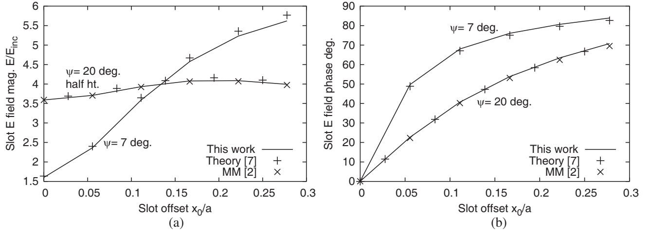
Figure 6. Variation of slot aperture electric field with slot offset. Comparison with modified analytical method [7] and mode method (MM) results [2]. (a) Aperture electric field magnitude with slot offset. (b) Aperture electric field phase with slot offset.
