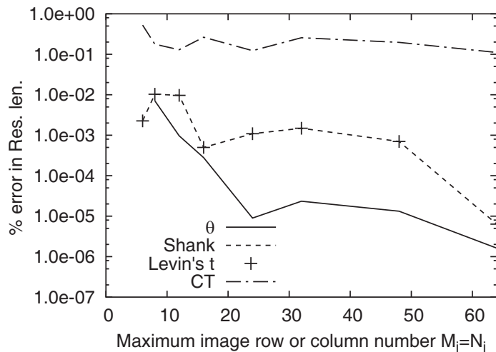
Figure 3. % error in resonant length with the maximum number of image row or column for various convergence acceleration algorithms.
