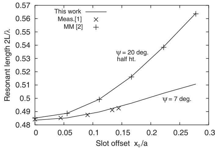
Figure 4. Resonant length with slot offset compared with measured [1] and mode method (MM) results [2].
