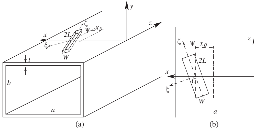
Figure 1. Geometry of the problem. (a) Waveguide fed compound slot. (b) Top view of the waveguide with compound slot.
