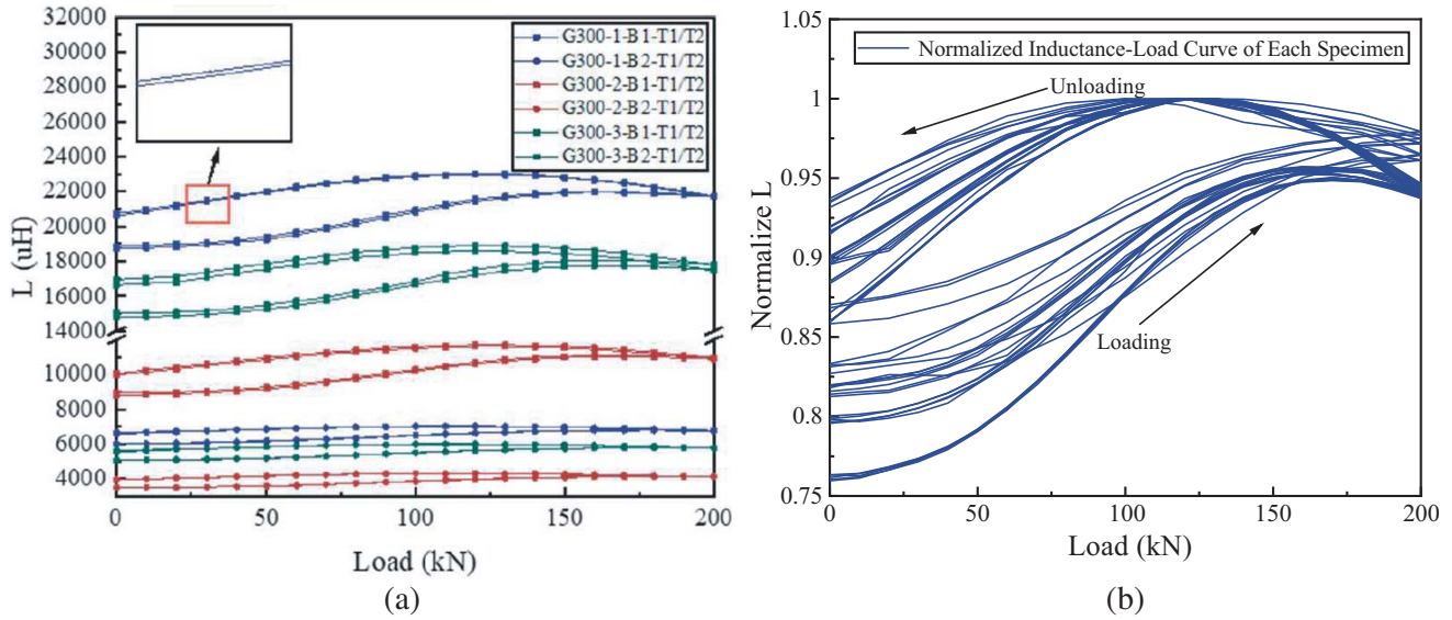
Figure 6. Inductance changed with load: (a) Inductance collected at different load levels; (b) Normalized inductance-load curves.
