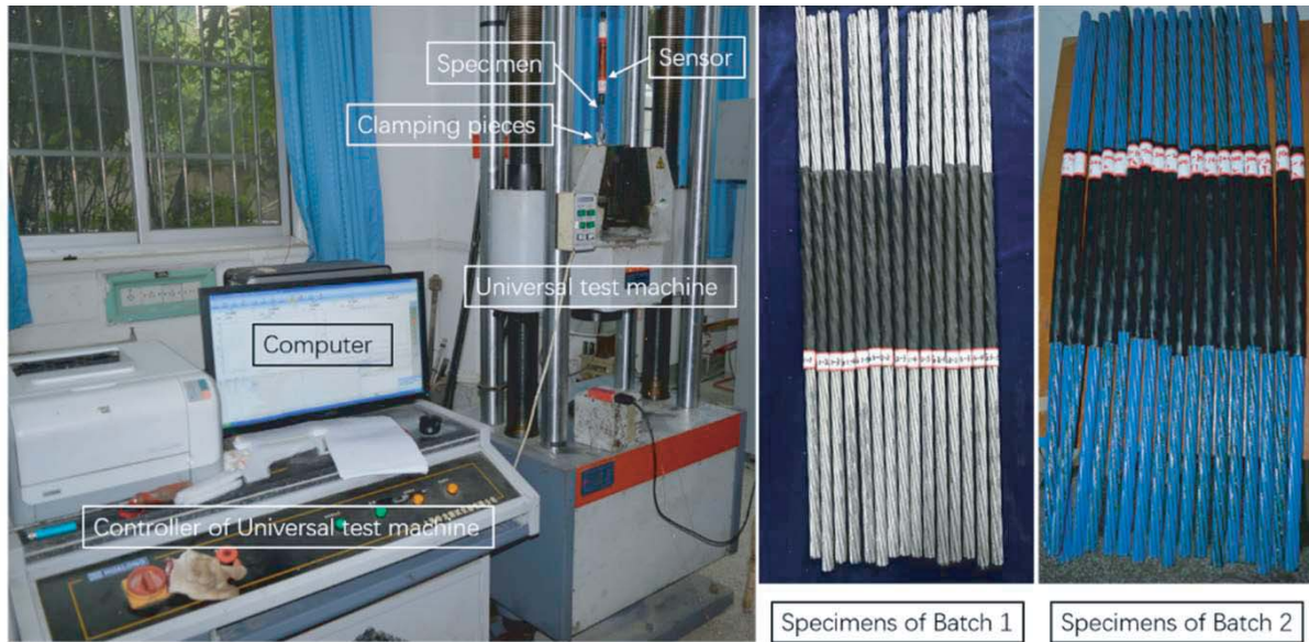
Figure 3. Experimental system and specimens.
