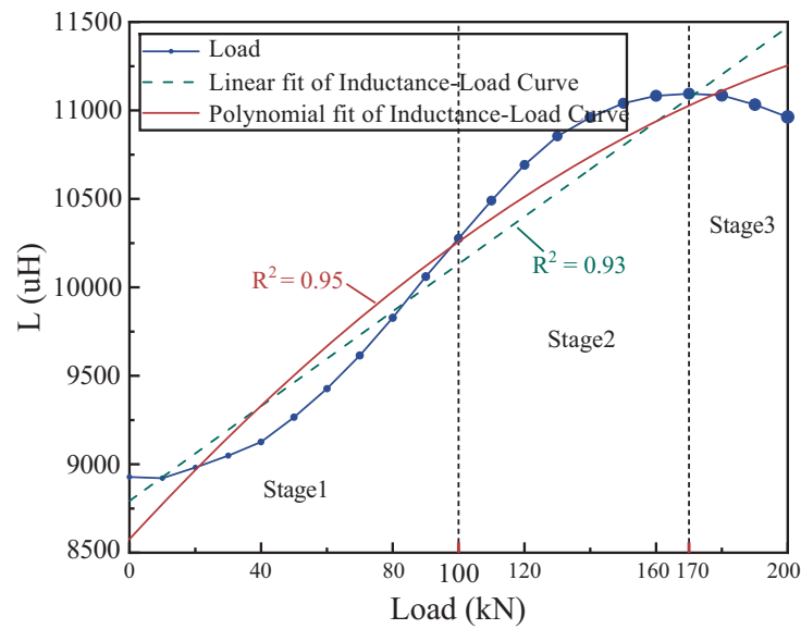
Figure 7. Inductance collected during the loading phase of specimen G300-1-B1-T1.
