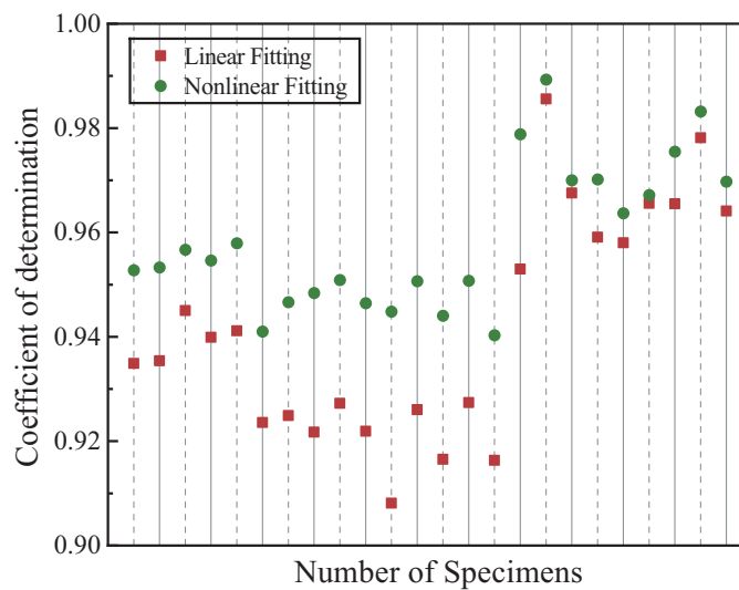
Figure 8. Coefficient of determination of each specimen obtained by linear fit and nonlinear fit during the loading phase.
