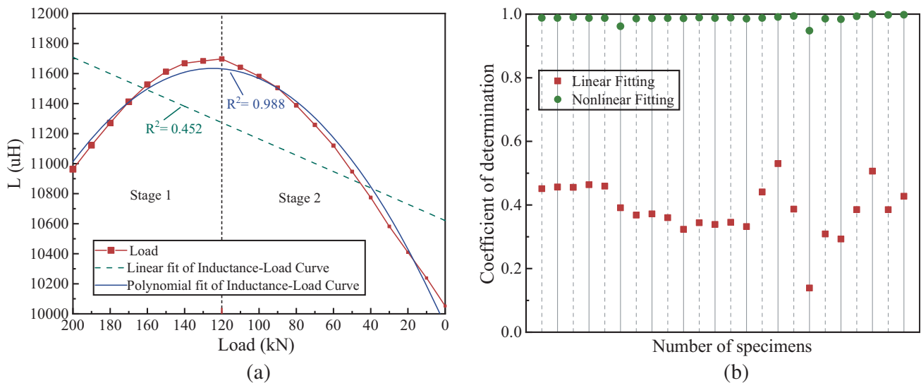
Figure 9. Analysis of the unloading stage: (a) Inductance collected during the unloading phase of specimen G300-1-B1-T1; (b) Coefficient of determination of each specimen obtained by linear fit and nonlinear fit during the unloading phase.
