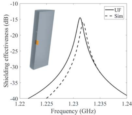
Figure 6. Shielding effectiveness versus frequency for the TM_{012} mode for a slotted cavity with a slot located at z = h/6 with an absorber at z = 0 . The absorber location within the cavity is reported as inset.
