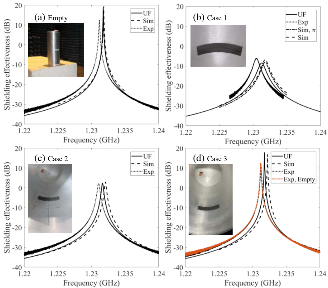
Figure 3. Shielding effectiveness versus frequency for the TM_{012} mode for (a) an empty cavity, and a loaded cavity as in (b) Case 1, (c) Case 2, and (d) Case 3. Photos of experiments are reported as insets. The unmatched formulation (UF) results using the short circuit current density for a finite cylinder are reported as solid curves. Full-wave simulation (Sim) and experimental (Exp) results are reported as dashed and dotted curves, respectively. The x -axis scale is narrow (1.22 to 1.24 GHz) around the TM_{012} mode to capture the exhibited large quality factors.
