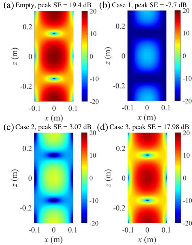
Figure 4. Electric field magnitude maps for the TM_{012} mode for (a) an empty cavity, and a loaded cavity as in (b) Case 1, (c) Case 2, and (d) Case 3. in the x - z plane for y = 0 . SE is the abbreviation used for shielding effectiveness.
