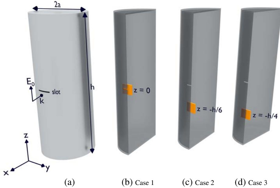
Figure 1. (a) Schematic of a slotted cylindrical enclosure excited by a plane-wave incident field as depicted to probe TM modes. The cavity is loaded with a microwave absorber material (orange box) at three different positions as outlined in panels (b)–(d) to dampen the EM fields. The origin of the reference system is at the center of the cylinder.
