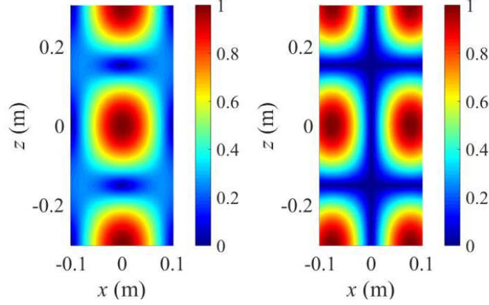
Figure 2. Normalized electric and magnetic field magnitude maps for the \text{TM}_{012} mode in an empty cavity in the x - z plane for y = 0 from Eqs. (1) and (5).
