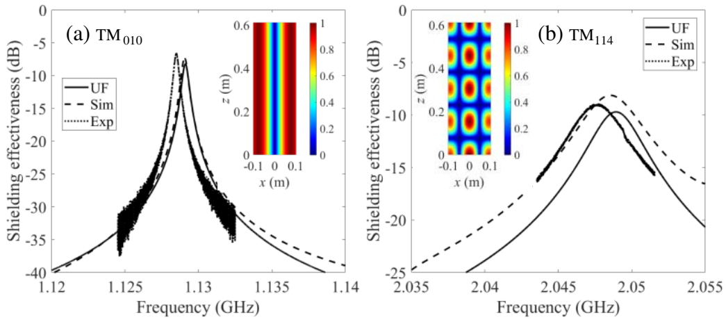
Figure 5. Shielding effectiveness versus frequency for the (a) TM_{010} and (b) TM_{114} modes for a loaded cavity with an absorber located at a magnetic field peak. Normalized magnetic field magnitude distribution within the cavity in the x - z plane for y = 0 from Eq. (1) for the two cases are reported as insets.
