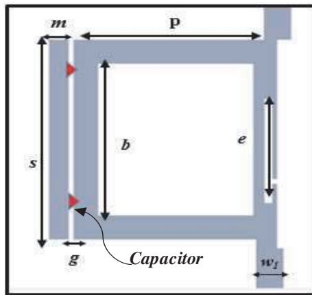
Figure 3. The proposed filter.
