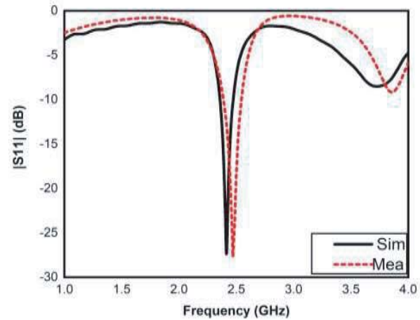
Figure 4. S_{11} simulation and measurement results for the filter.
