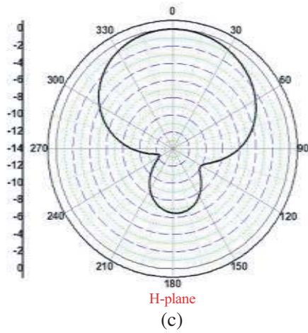
Figure 15. Simulated E - and H -planes patterns at 2.4 GHz (a) and (b) conventional antenna and (c) and (d) filtenna.
