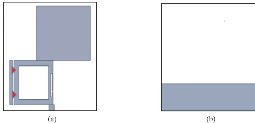
Figure 10. The structure of the proposed filtenna (a) top view, (b) bottom view.
