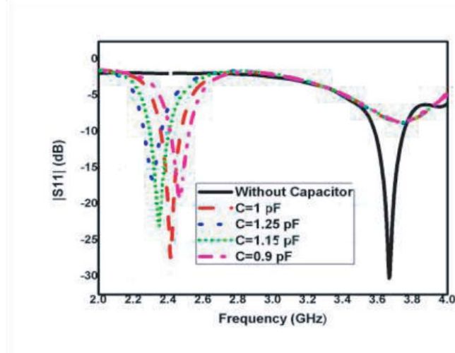
Figure 6. The return loss at various capacitor values for the suggested filter.
