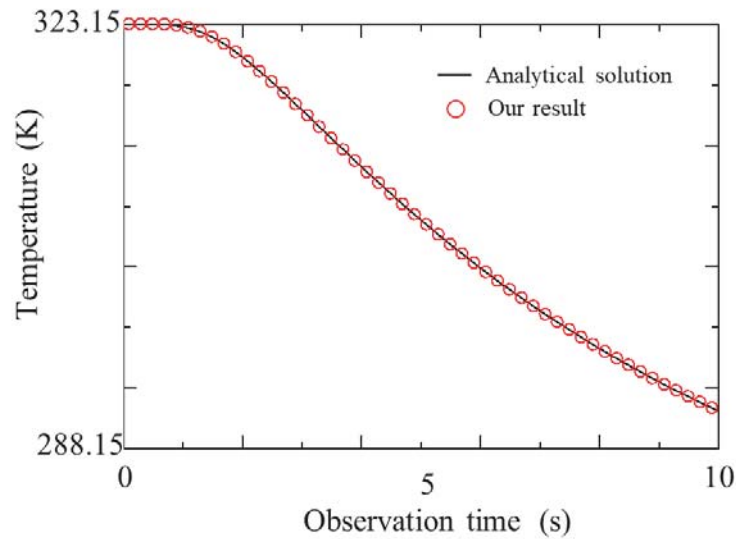
Figure 4. Temperature-time response at the observation plane. The results from the proposed method are in good agreement with the analytical solution at all observation times.
