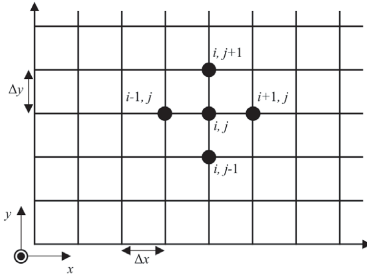
Figure 1. Space discretization for the finite difference scheme, i and j indicate the discretized points for the x and y directions, respectively. \Delta x and \Delta y represent the size of the unit cell.
