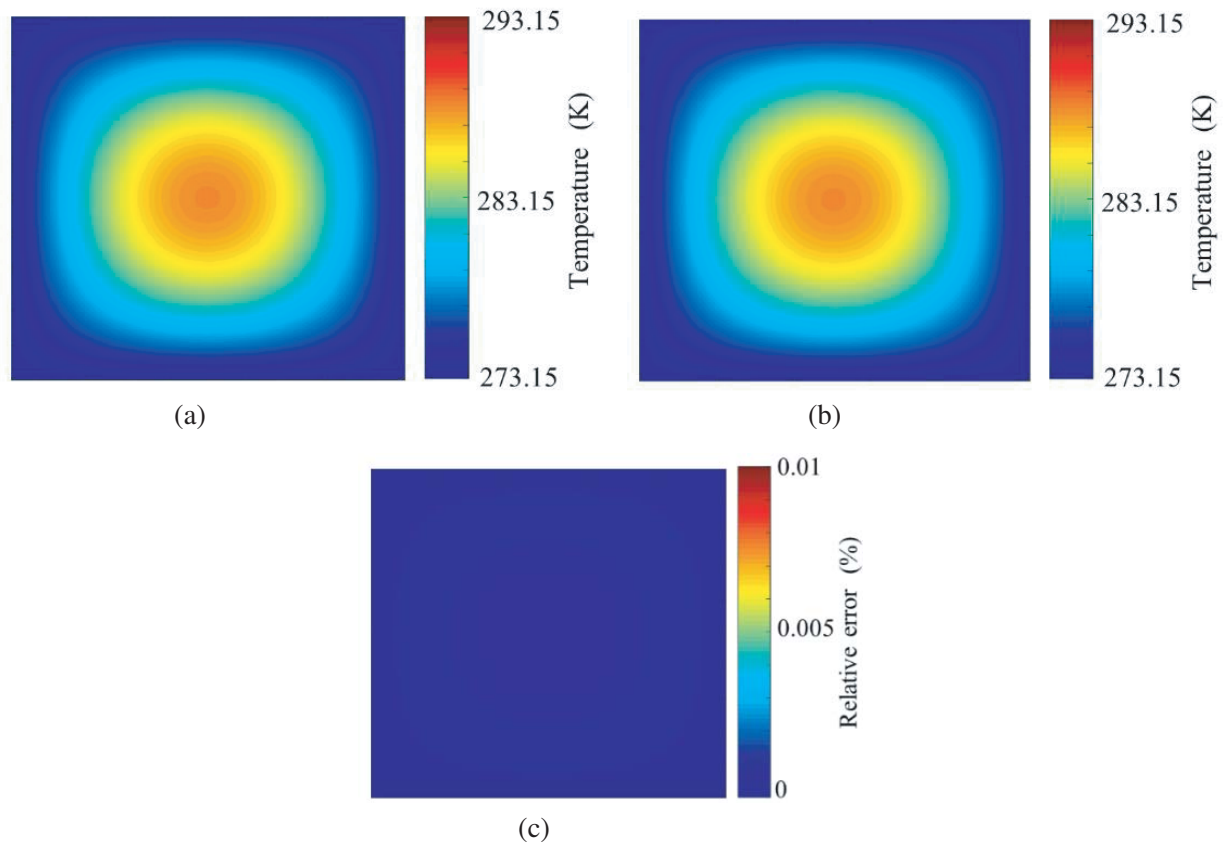
Figure 7. Temperature distribution at t = 6 s obtained using (a) the proposed method and (b) conventional FDM. (c) Relative error between the proposed method and conventional FDM. The computational error is less than 0.005% for the complete computational area.
