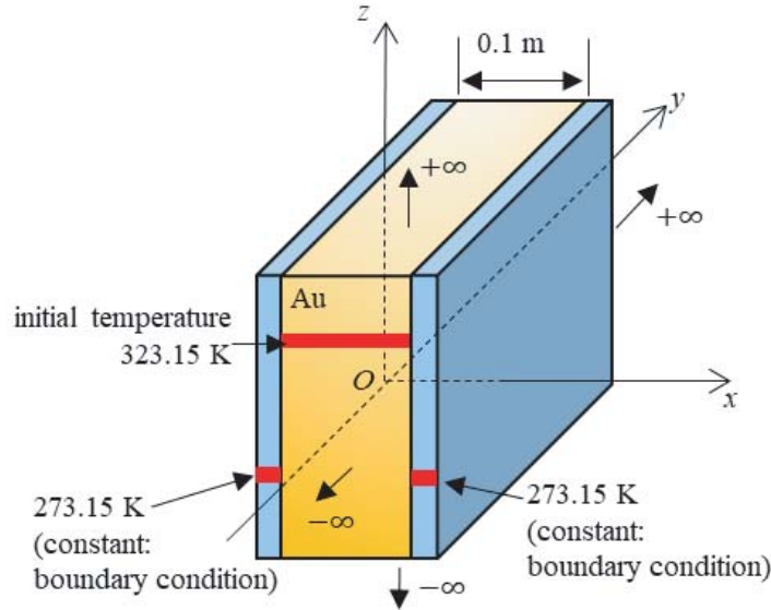
Figure 3. Computational model of a two-dimensional object for validating the proposed heat transfer computational method.
