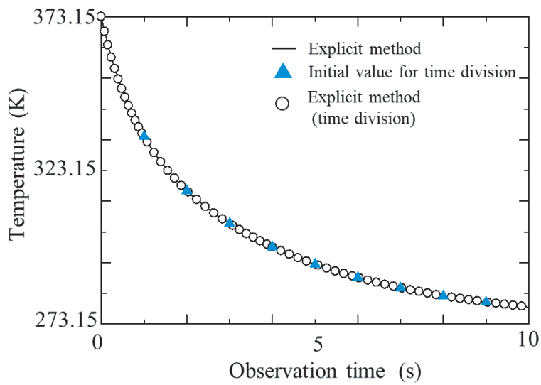
Figure 8. Temperature-time response at the center of an object. Parallel computing can be performed by the proposed method.
