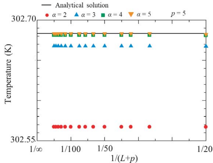
Figure 5. Convergence test for various truncation numbers, L . The result converges as the truncation number increases. The accuracy of the result increases with the truncation number.
