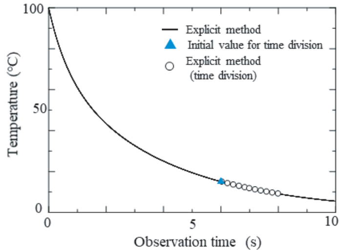
Figure 9. Temperature-time response at the desired observation period by the proposed method and TD-FDM.
