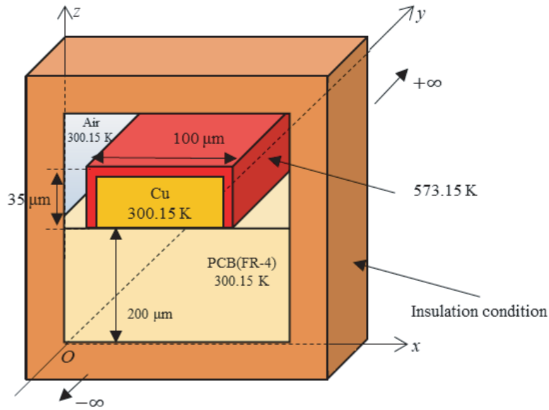
Figure 10. Computational model of heat transfer problem of PCB.
