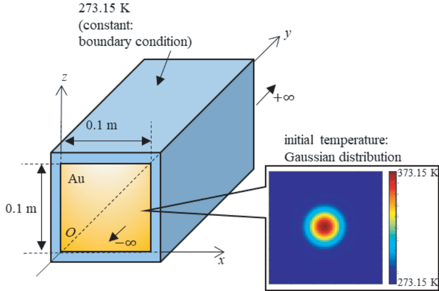
Figure 6. Computational model of a two-dimensional object made of gold for validating the proposed heat transfer computation method.
