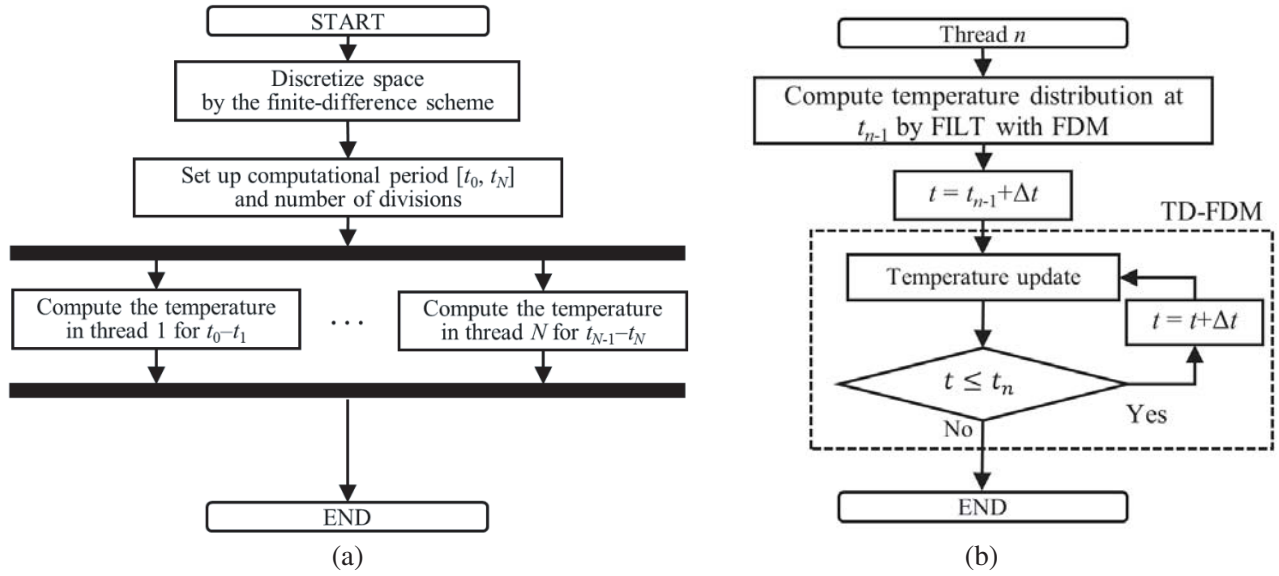
Figure 2. Flowchart for the time-division parallel computing method. (a) Distributing observation time to threads. (b) Computing the temperature distribution in each thread. The initial temperature distribution can be obtained by FILT with FDM expanded in the complex frequency domain.
