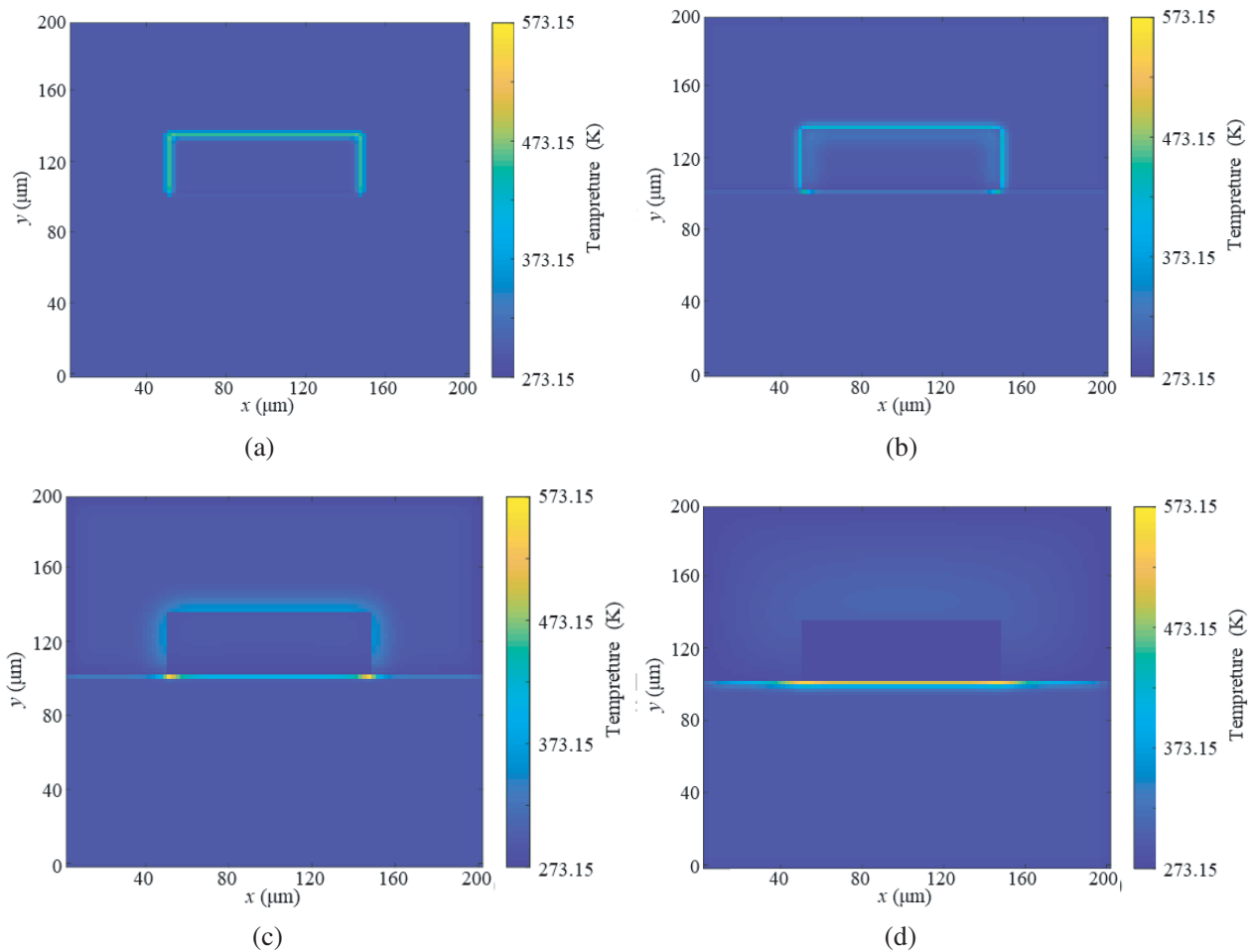
Figure 11. Temperature distributions at a specific observation time t computed by our method. (a) t = 10 ns, (b) t = 100 ns, (c) t = 1000 ns, and (d) t = 10000 ns.
