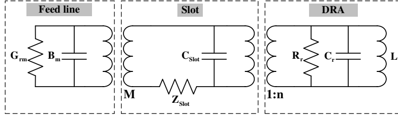
Figure 6. Equivalent circuit model diagram of DRA fed by aperture.
