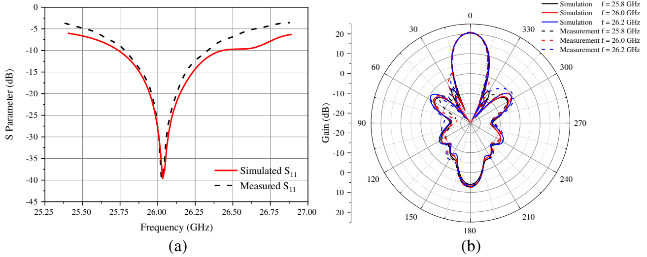
Figure 20. Measured and simulated results of planar antenna array fed by series-parallel hybrid feed. (a) S parameters S_{11} . (b) Radiation patterns.
