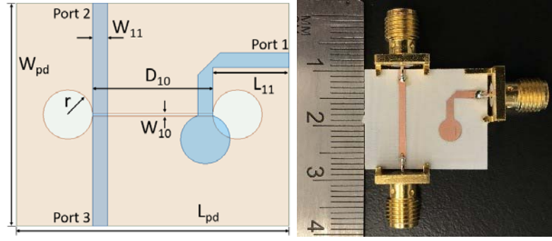
Figure 2. The top-view of the wideband power divider.
