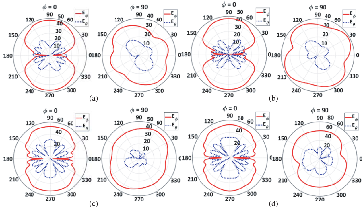
Figure 8. Radiation pattern of transmit mode with \Phi = 0^\circ and \Phi = 90^\circ at (a) 8 GHz, (b) 9 GHz, (c) 10 GHz, (d) 11 GHz.
