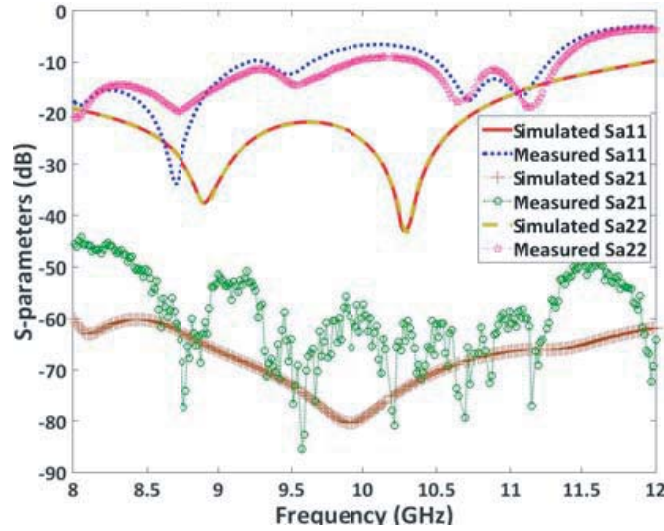
Figure 4. Simulated and measured S -parameters using first method.
