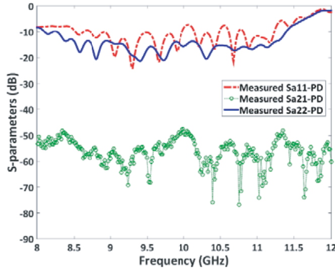
Figure 6. Measured S -parameters with power divider.
