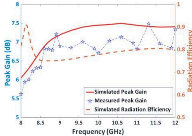
Figure 7. Simulated and measured gain of the antenna system.
