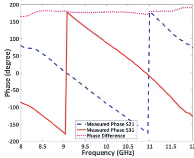
Figure 3. Measured phase of output ports for the modified power divider.
