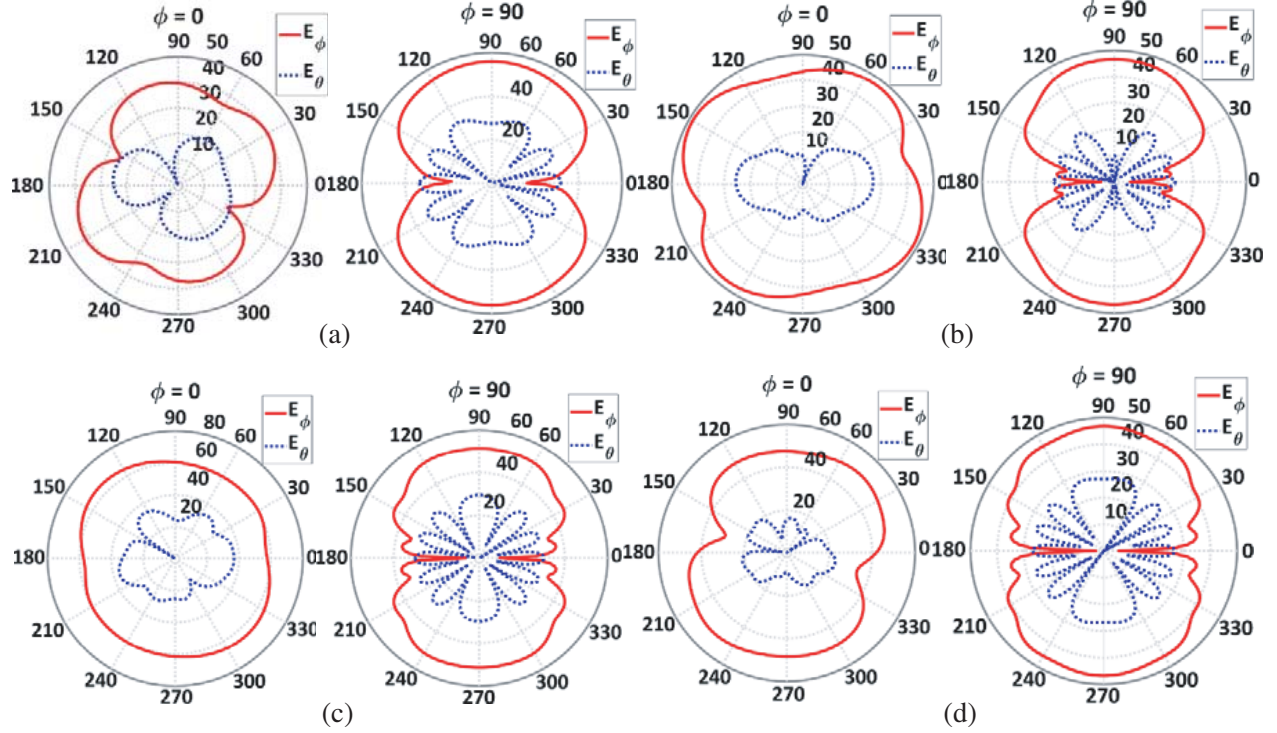
Figure 9. Radiation pattern of receive mode with \Phi = 0^\circ and \Phi = 90^\circ at (a) 8 GHz, (b) 9 GHz, (c) 10 GHz, (d) 11 GHz.
