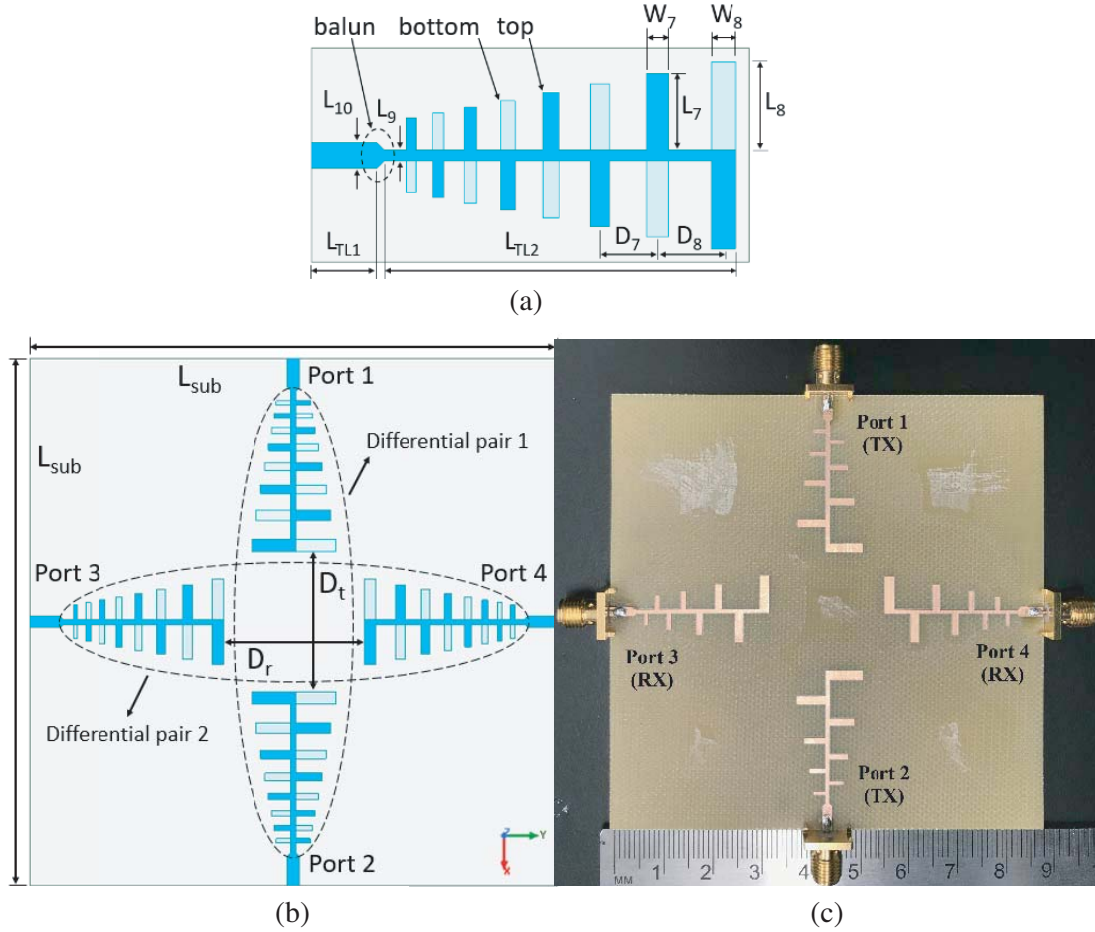
Figure 1. (a) The geometry of a single LPDA; (b) The geometry of LPDA antenna system; (c) The top view of the fabricated system.
