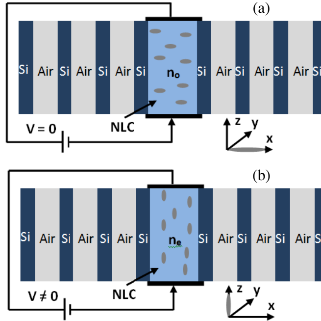
Figure 2. Working principle diagram of the N-CL. At the (a) \emptyset = 0^\circ and (b) \emptyset = 90^\circ of the 1D PhC microcavity structure.
