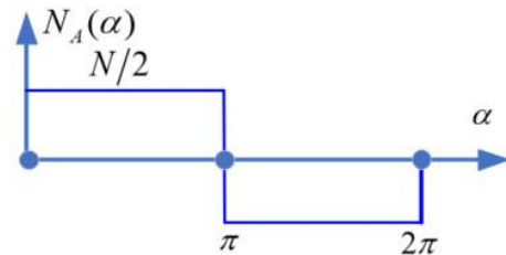
Figure 5. Winding function of phase A for star winding.
