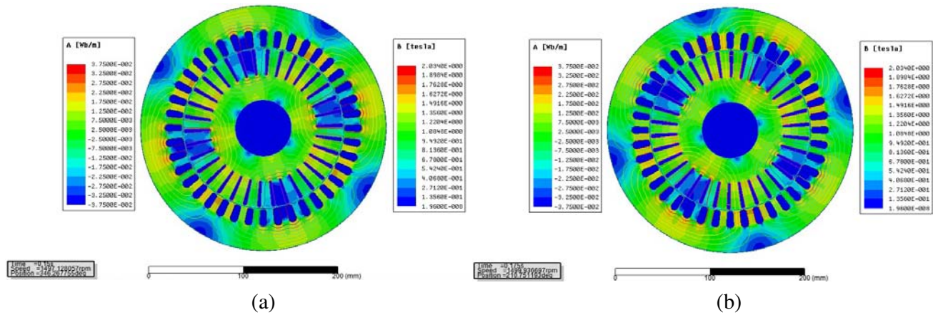
Figure 7. The magnetic field density of pentacle-star winding five-phase motor, (a) when t = 0.15 s, (b) when t = 0.175 s.
