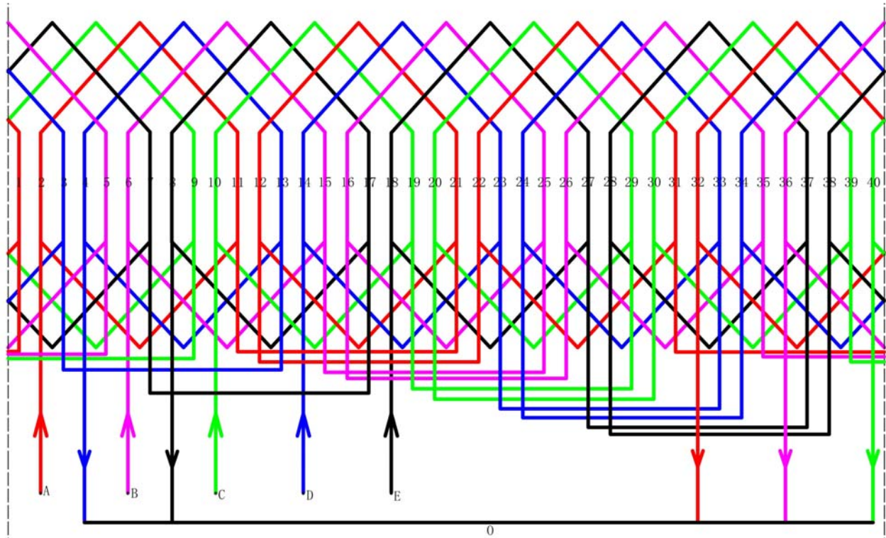
Figure 2. Star winding diagram.
