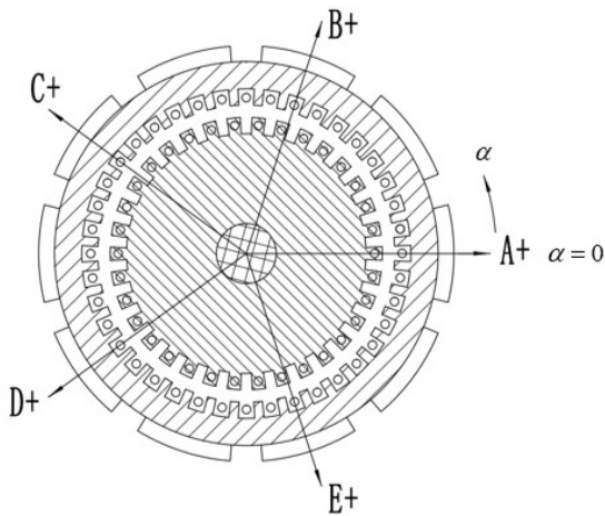
Figure 4. Star winding co-ordinate system diagram.
