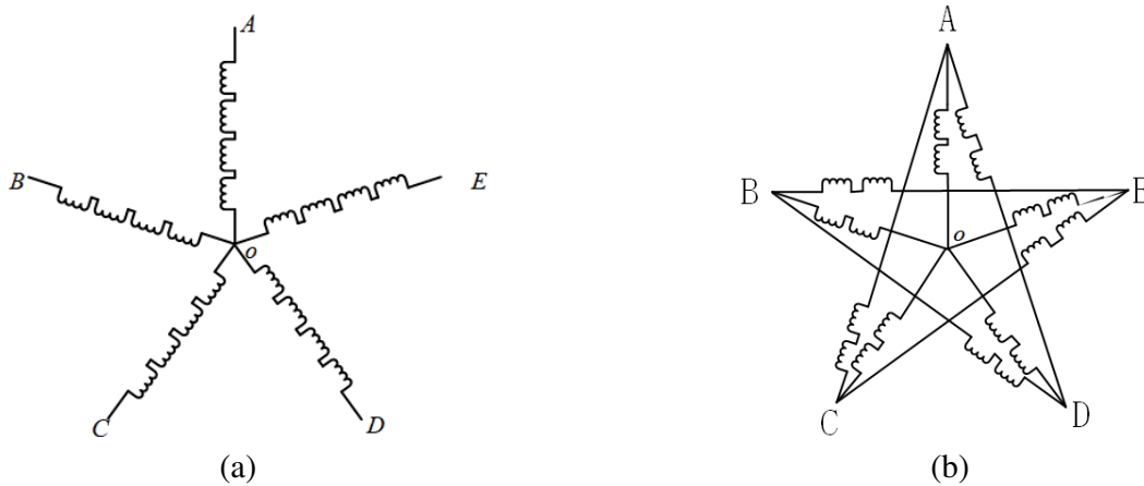
Figure 1. Star and novel pentacle-star winding configuration for a five-phase motor. (a) Star winding. (b) Pentacle-star winding.
