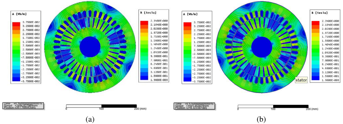
Figure 6. The magnetic field density of star winding five-phase motor, (a) when t = 0.15 s, (b) when t = 0.175 s.
