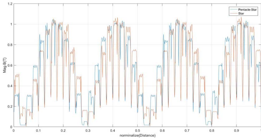
Figure 8. Air gap flux density for five-phase motor: star winding and pentacle-star winding.
