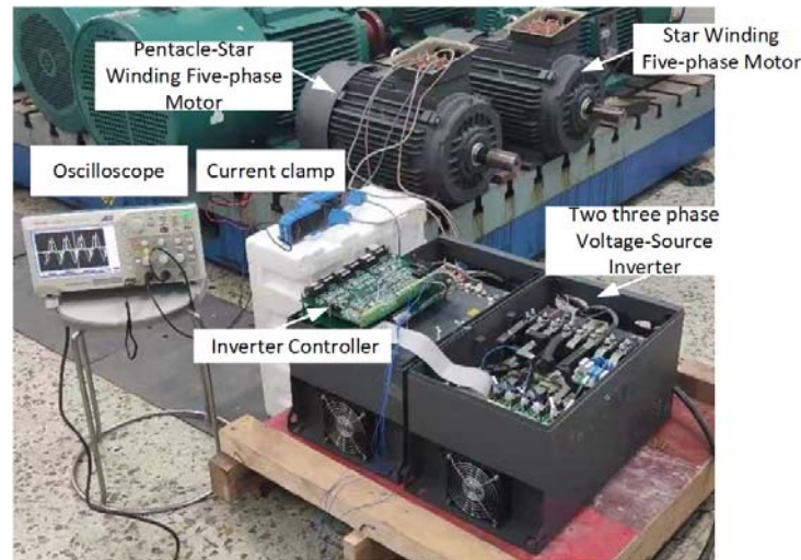
Figure 9. Pentacle-star and star five-phase prototype motor based on Y160L-4.
