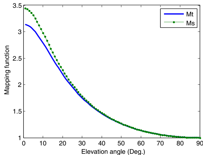
Figure 2. Comparison of thin and thick shell mapping functions.
