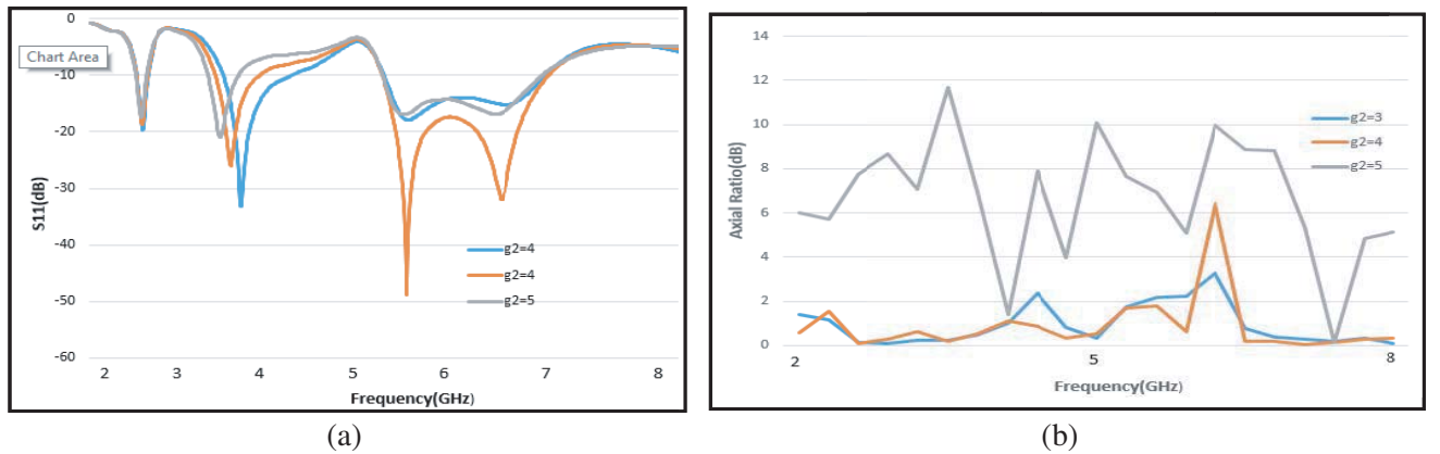
Figure 7. Effects of g_2 on antenna performances. (a) S_{11} and (b) axial ratio.
