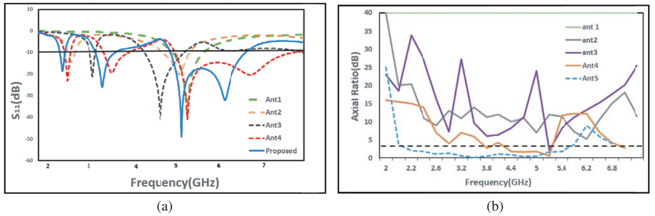
Figure 3. Simulated results of antenna different steps. (a) S_{11} . (b) Axial ratio.
