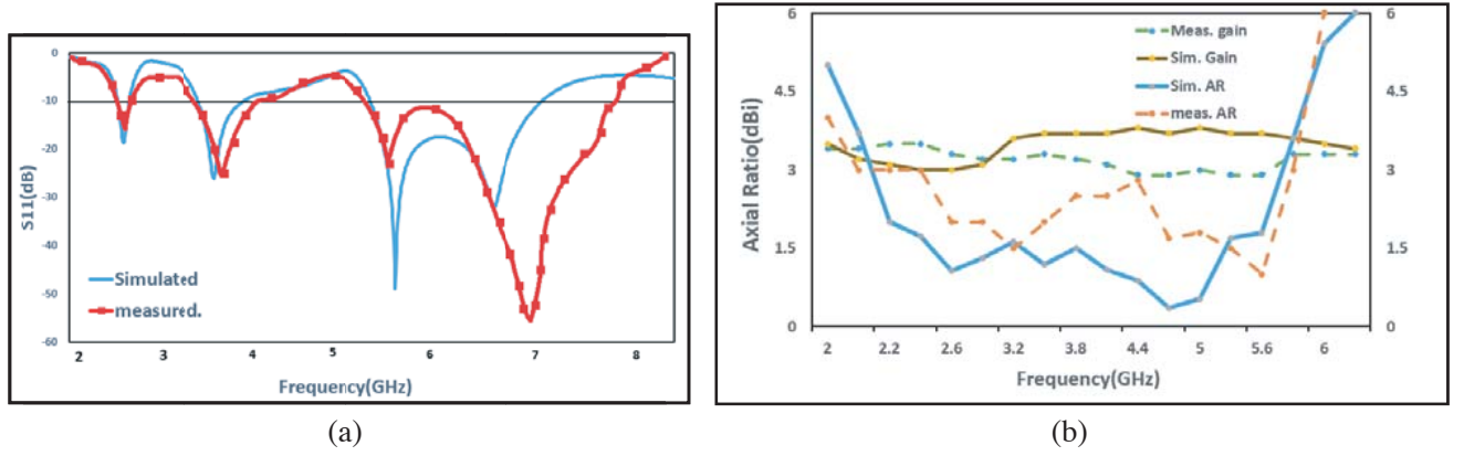
Figure 10. Simulated and measured results. (a) |S_{11}| . (b) AR and realized gain at \theta = \phi = 0^\circ .
