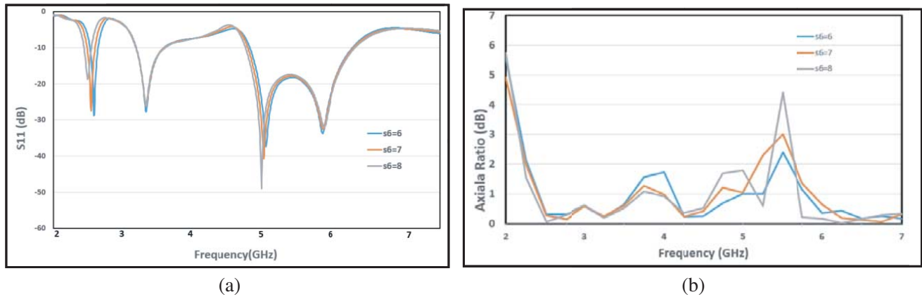
Figure 8. Effect of s6 on (a) S_{11} , (b) axial ratio.
