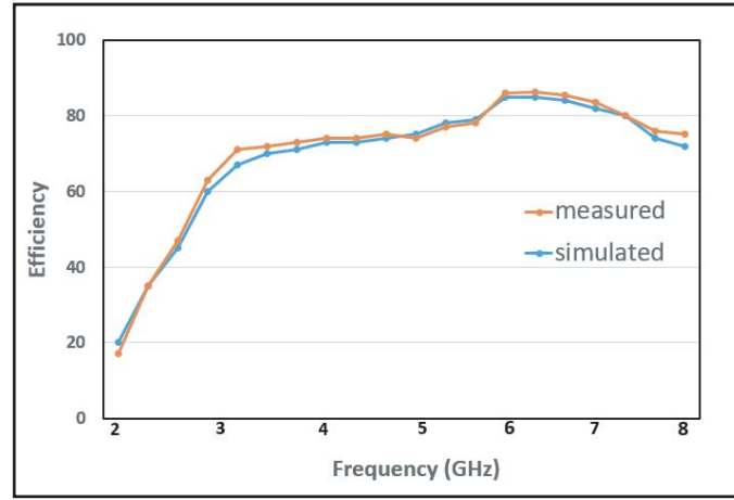
Figure 11. Radiated efficiency of proposed antenna.
