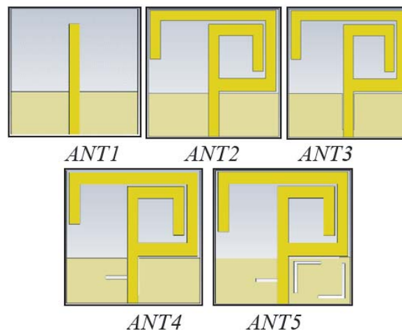
Figure 2. Improvement procedure for designed antenna.
