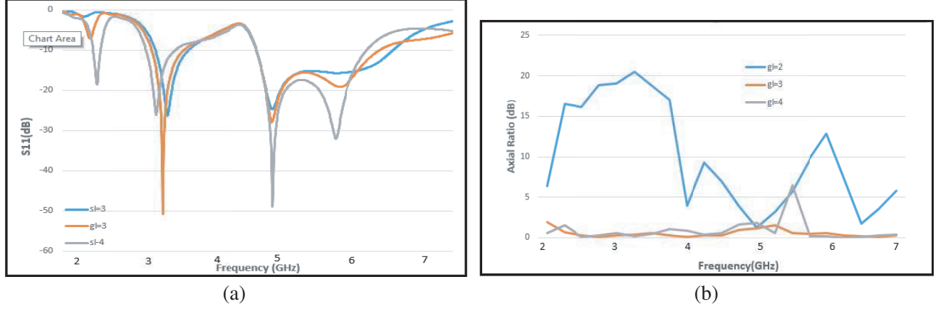
Figure 6. Effects of g_1 on antenna performances. (a) S_{11} and (b) axial ratio.
