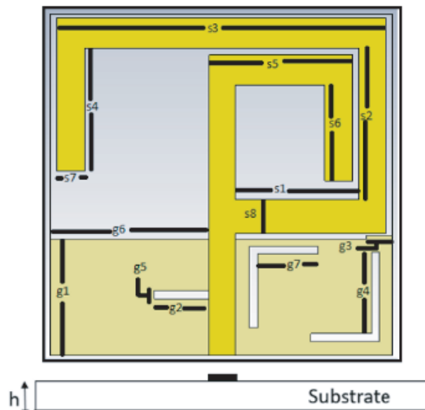
Figure 1. Schematic diagram of proposed antenna.
