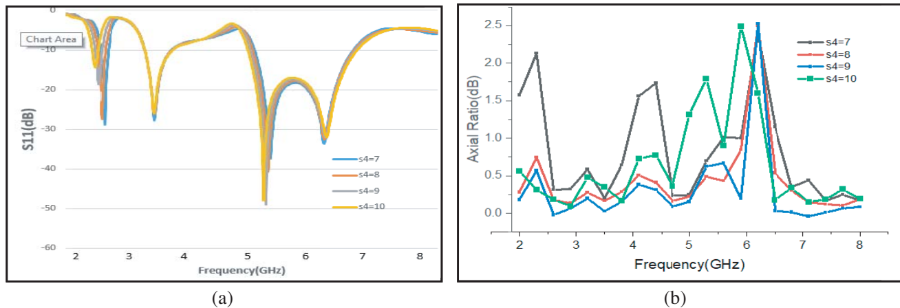
Figure 5. Effects of s_4 on antenna performances. (a) S_{11} and (b) axial ratio.
