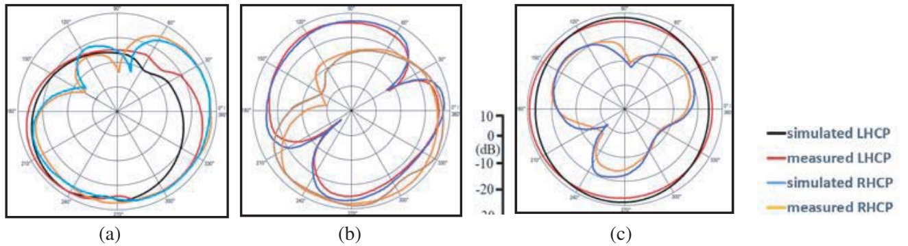
Figure 12. Radiation Pattern at (a) at 2.45 GHz, (b) at 3.8 GHz, (c) at 5.8 GHz.
