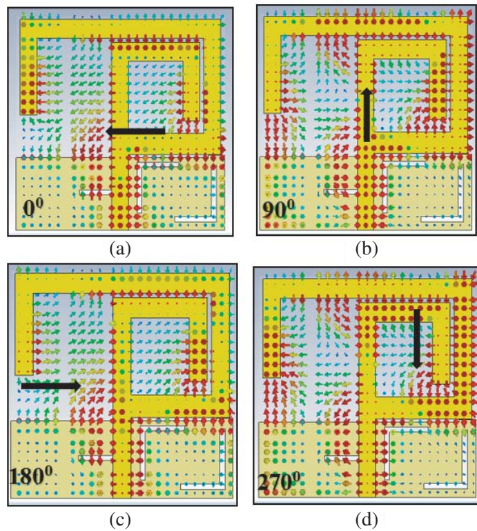
Figure 4. Surface current density over the proposed antenna at 5.2 GHz with the phase of 0^\circ , 90^\circ , 180^\circ and 270^\circ .
