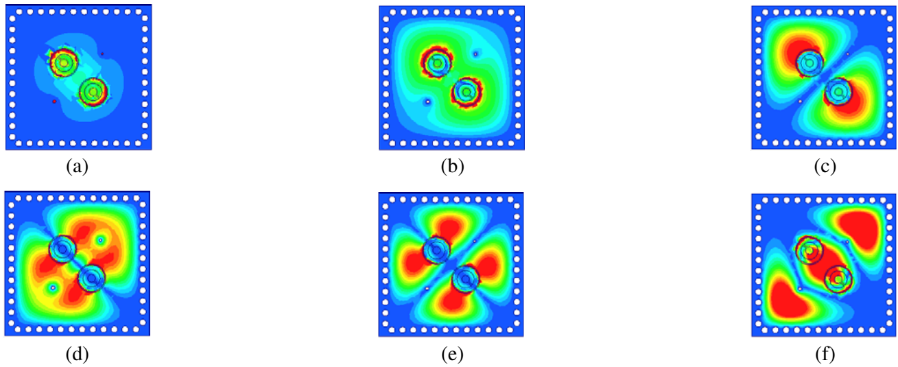
Figure 2. Electric field distributions of the first six modes in the proposed resonator. (a) CSRRs mode, (b) TE_{101} , (c) TE_{102} , (d) TE_{201} , (e) TE_{202} , (f) TE_{301} .
