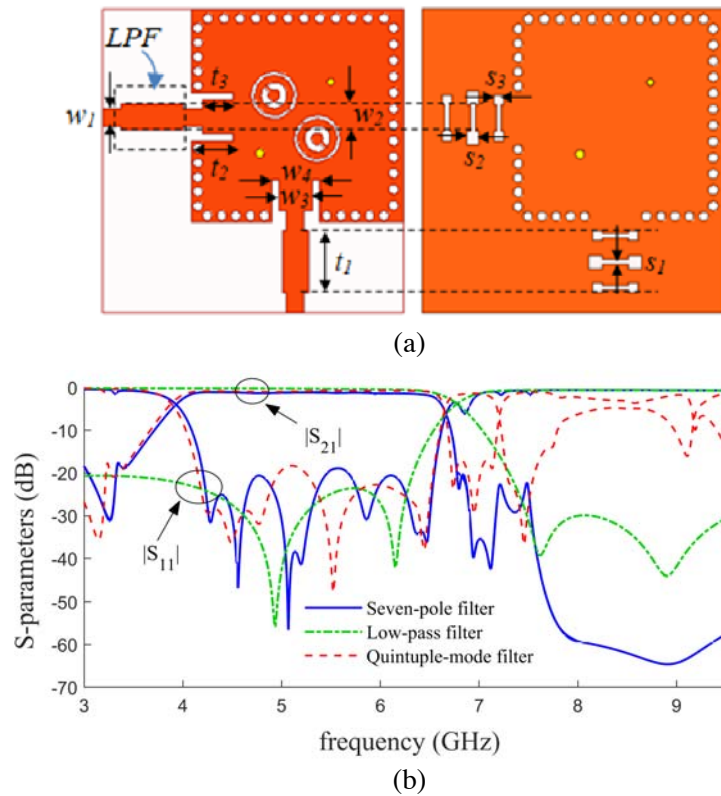
Figure 4. (a) Basic structure of the proposed multi-mode filter. (b) Quintuple-mode filter, DGS-LPF, and the seven-pole filter responses.
