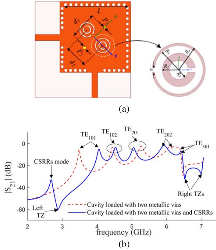
Figure 1. (a) Quintuple-mode SIW resonator and the CSRRs configuration. (b) Simulated |S_{21}| of the quintuple-mode resonator-with and without CSRRs under weak coupling.
