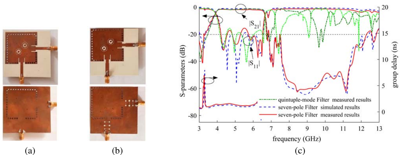
Figure 5. (a) Photography of the fabricated quintuple-mode filter. (b) Photography of the fabricated seven-pole filter. (c) S -parameters of the proposed filters and group delay of the seven-pole filter.
