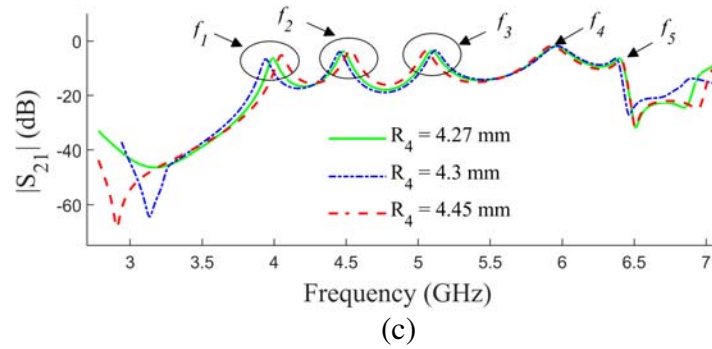
Figure 3. Resonant frequencies variation versus (a) the length d_1 , (b) the radius R_1 , (c) the radius R_4 under weak coupling.
