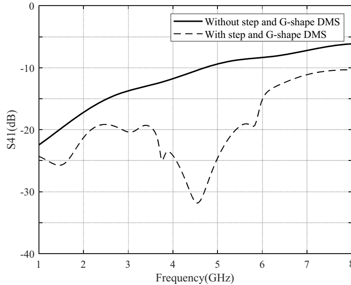
Figure 7. Comparison of the simulation results of microstrip lines S_{41} before and after the combination of G-shaped DMS and step-shaped transmission line.
