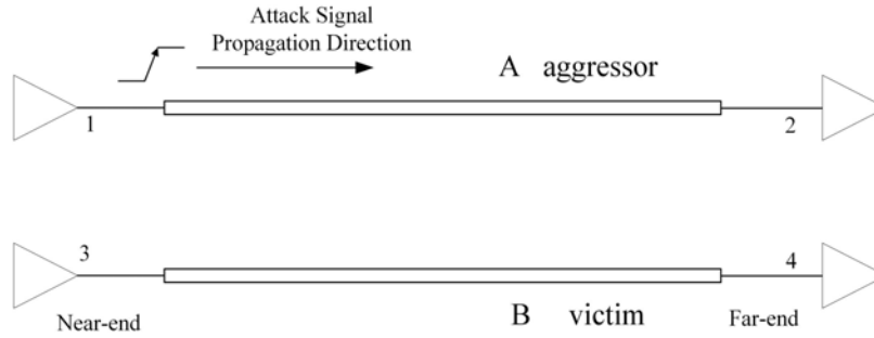
Figure 1. Coupling microstrip lines signal transmission model.
