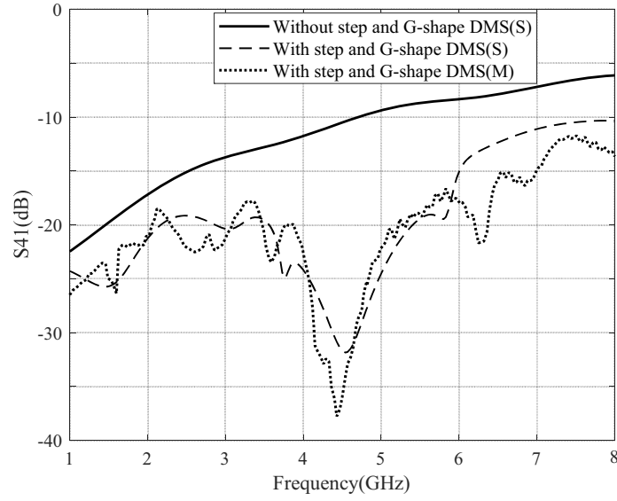
Figure 11. Comparison of the simulation and measured results of microstrip lines S_{41} before and after the combination of G-shaped DMS and step-shaped transmission line.
