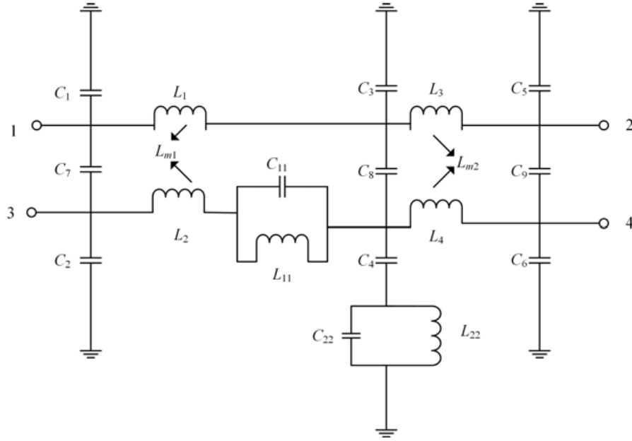
Figure 4. Equivalent circuit of the coupled microstrip lines with etched G-shaped DMS.
