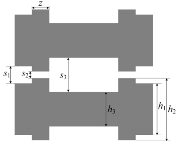
Figure 2. Geometric structure of step-shaped transmission line.
