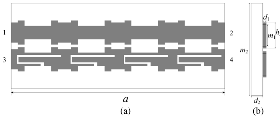
Figure 6. Coupled microstrip lines combining G-shaped DMS and step-shaped transmission line. (a) Top view. (b) Side view.
