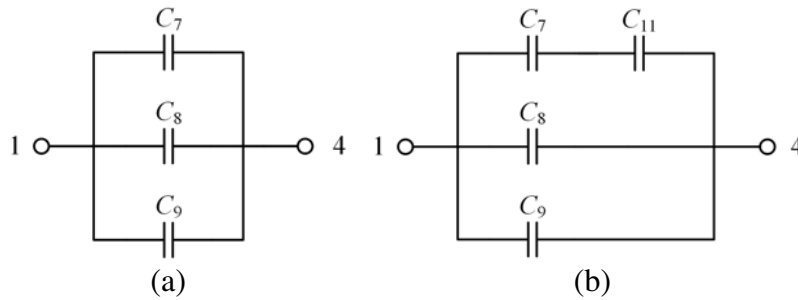
Figure 5. Total capacitive coupling from port 1 to port 4. (a) Without G-shaped DMS. (b) With G-shaped DMS.
