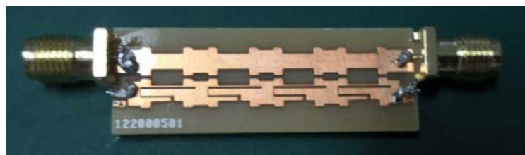
Figure 10. Actual production diagram of measuring insertion loss S_{21} .
