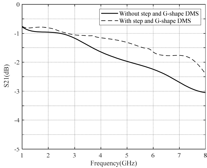
Figure 8. Comparison of the simulation results of microstrip lines S_{21} before and after the combination of G-shaped DMS and step-shaped transmission line.
