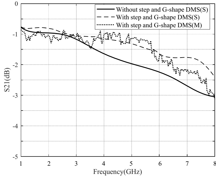
Figure 12. Comparison of the simulation and measured results of microstrip lines S_{21} before and after the combination of G-shaped DMS and step-shaped transmission line.
