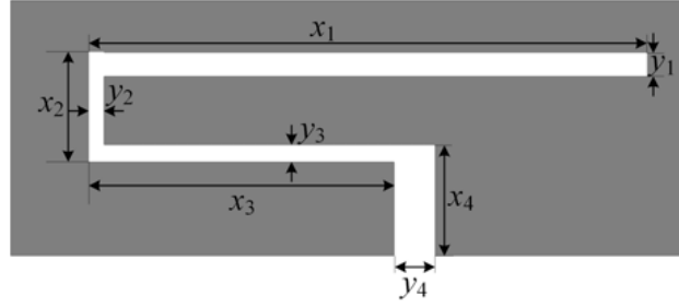
Figure 3. Geometric structure of G-shaped DMS.
