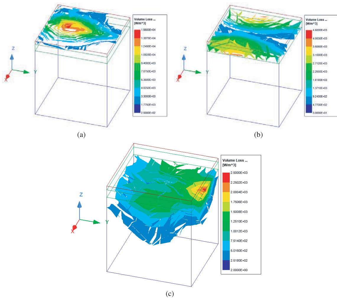
Figure 6. Simulated volume loss density for 1 V of input voltage at the antenna port, (a) skin, (b) fat, and (c) muscle.
