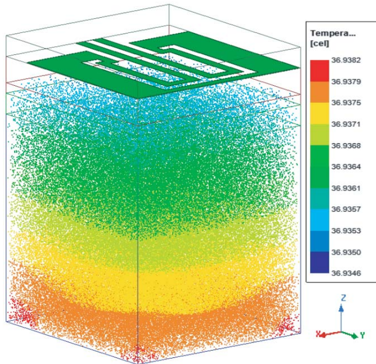
Figure 7. 3D thermal emission visualization at 1.4 GHz.
