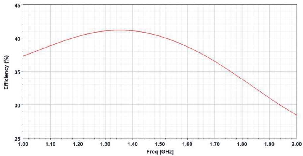
Figure 5. Antenna radiation efficiency.
