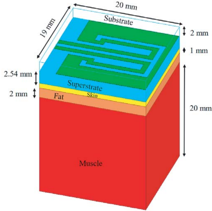
Figure 2. Antenna configuration and dimensions with three-layer tissue structure.
