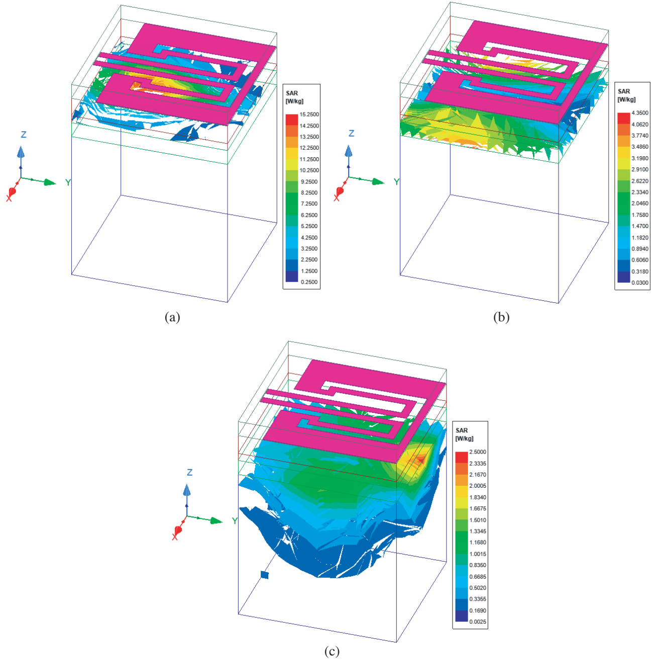
Figure 4. Simulated SAR at frequency of 1.4 GHz for (a) skin, (b) fat, and (c) muscle.
