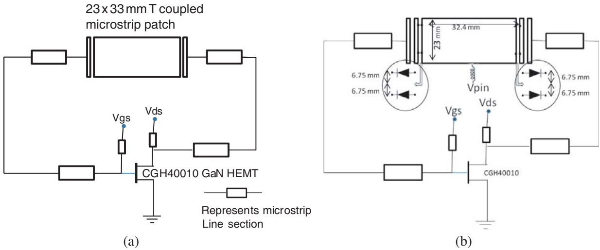
Figure 1. Schematic of (a) fixed frequency high power AIA, (b) frequency reconfigurable high power AIA.
