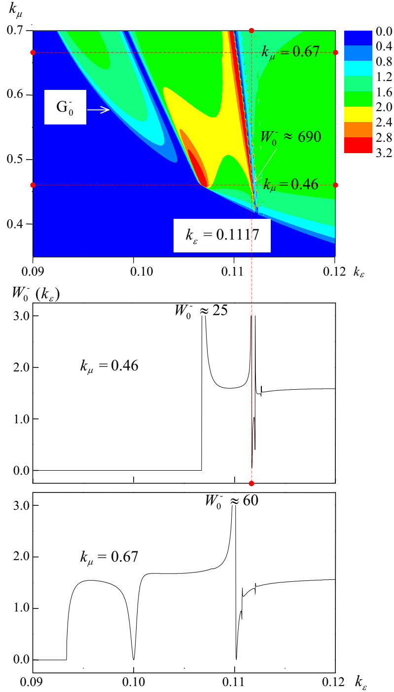
Figure 5. Efficiency W_0^-(k_\varepsilon, k_\mu) of VChR in a half-space occupied by a binegative plasma-like medium, and a section of the surface W_0^-(k_\varepsilon, k_\mu) by planes k_\mu = 0.46 , k_\mu = 0.67 : h = 0.4 , \beta = 0.2 , and k = 0.08 .
