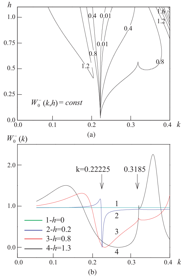
Figure 1. (a) Lines W_0^-(k, h) = \text{const} , characterizing the intensity of diffraction radiation into the half-space y < f(z) , and (b) curve W_0^-(k) for various values of h : \mu(k) = -4.84 , \varepsilon(k) = -0.84 , and \beta = 0.89 .
