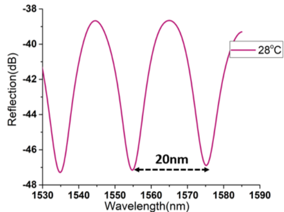
Figure 7. Spectrum of the temperature sensor sample (S2).
