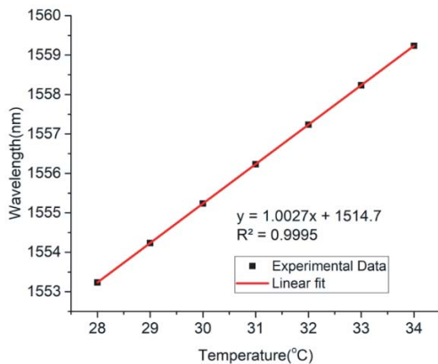
Figure 6. Linear fitting line for wavelength versus temperature (S1).
