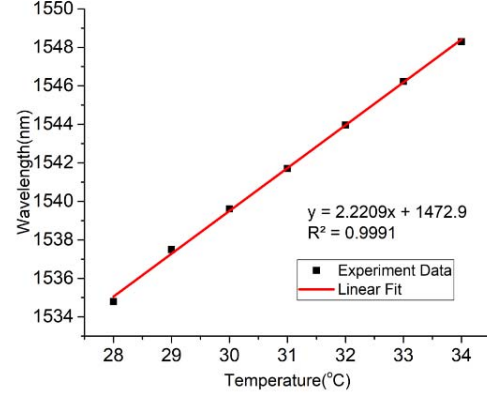
Figure 9. Linear fitting line for wavelength versus temperature (S2).
