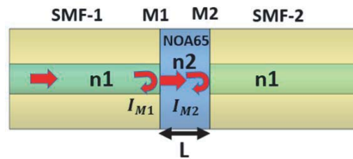
Figure 1. Schematic diagram of the FPI temperature sensor.
