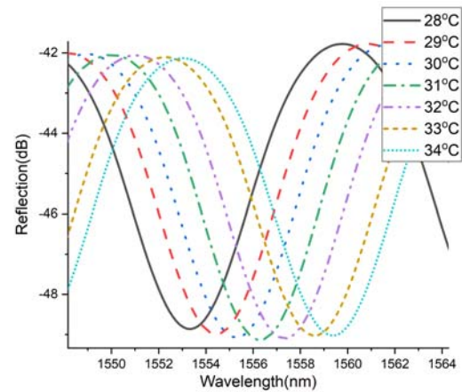
Figure 5. Reflection spectral evolution of FPI sensor (S1) under different temperature measurements.
