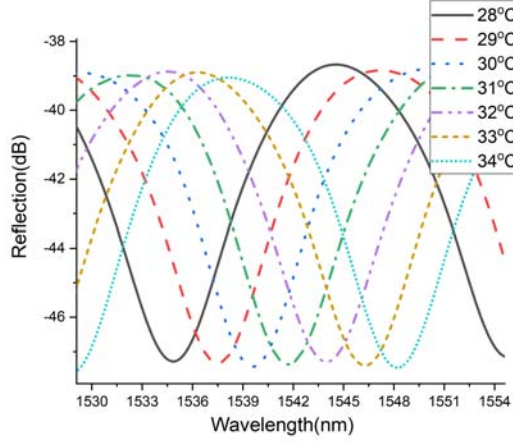
Figure 8. Reflection spectral evolution of FPI sensor (S2) under different temperature measurements.
