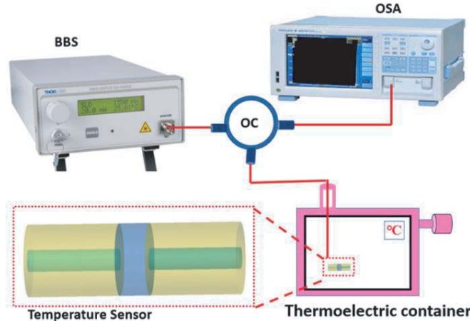
Figure 3. Temperature measurement setup for FPI sensor.
