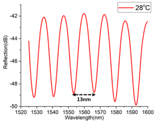
Figure 4. Spectrum of the temperature sensor sample (S1).
