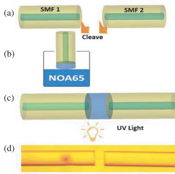
Figure 2. Fabrication steps of the proposed polymer based on FPI cavity temperature sensor.
