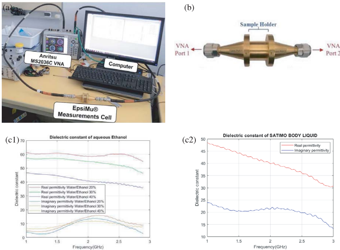
Figure 4. (a) Dielectric property measurements setup using EpsiMu ® Tool [48,50], and Anritsu MS2036C Vector Network Analyzer. (b) Photograph of the coaxial cell for the dielectric measurements. EpsiMu ® toolbox consists of a coaxial cell based on the two-port transmission line technique and a related software to monitor a calibrated Vector Network Analyzer. (c1) Comparison between the measured dielectric properties of the mimicking mixtures of human blood (Water-Ethanol). (c2) Measured dielectric properties of the SATIMO Body Liquid, mimicking tissue of muscle, in 1–3 GHz band.
