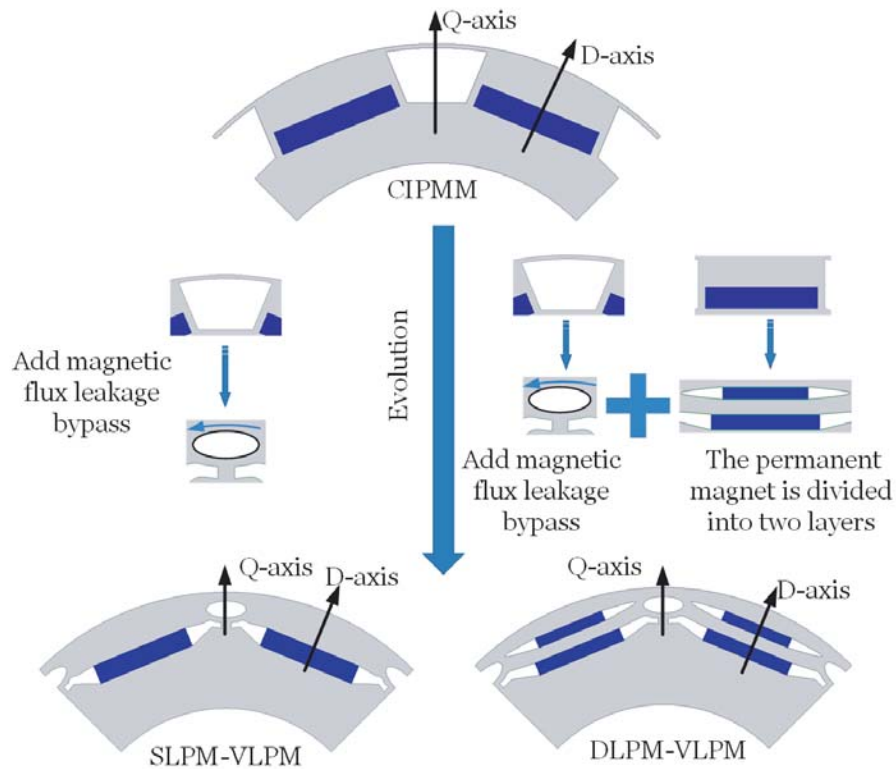
Figure 1. Rotor evolution from the conventional interior PM motor to the SLPM-VLPM and the DLPM-VLPM.
