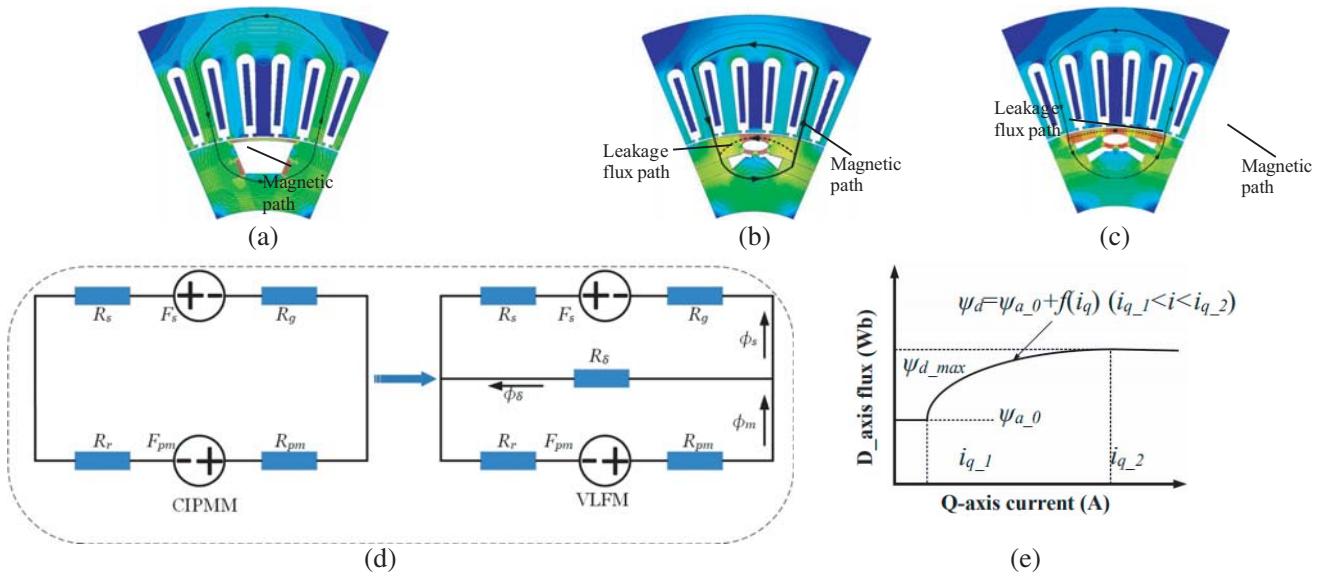
Figure 2. Theoretical analysis for variable leakage flux. (a) Magnetic path of CIPMM. (b) Magnetic path of SLPM-VLFM. (c) Magnetic path of DLPM-VLFM. (d) Magnetic equivalent circuit. (e) Variable flux property.
