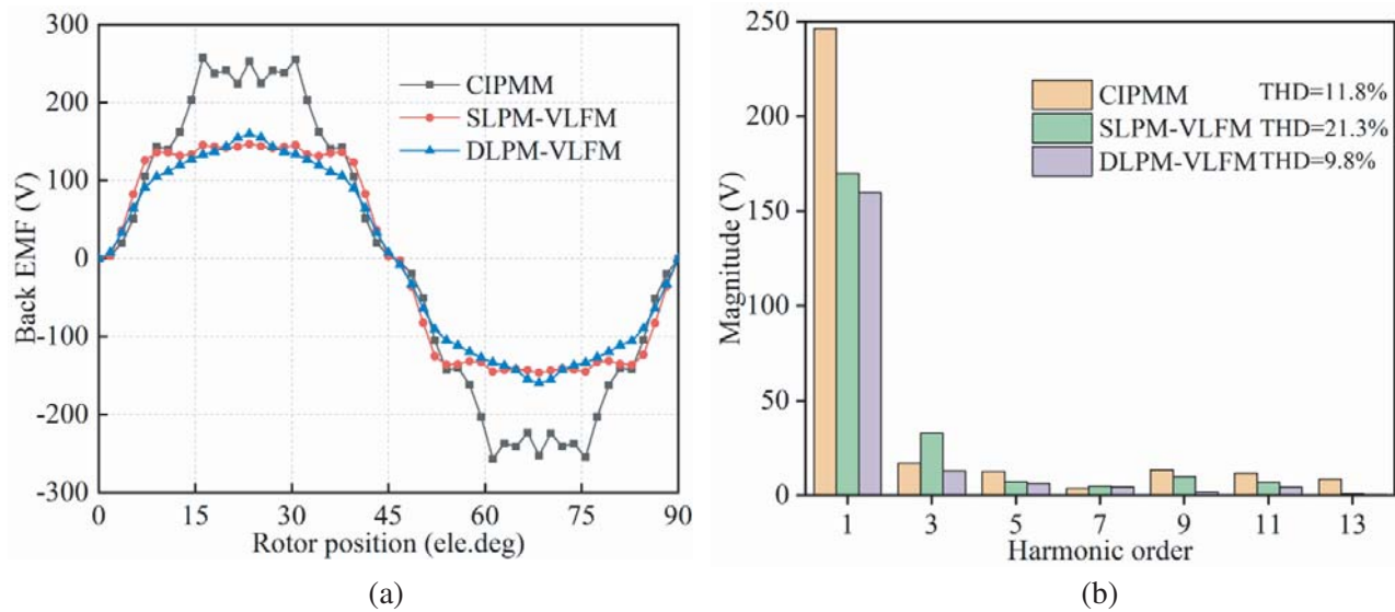
Figure 7. No-load back-EMF of the three motors. (a) Waveforms. (b) Harmonic component.
