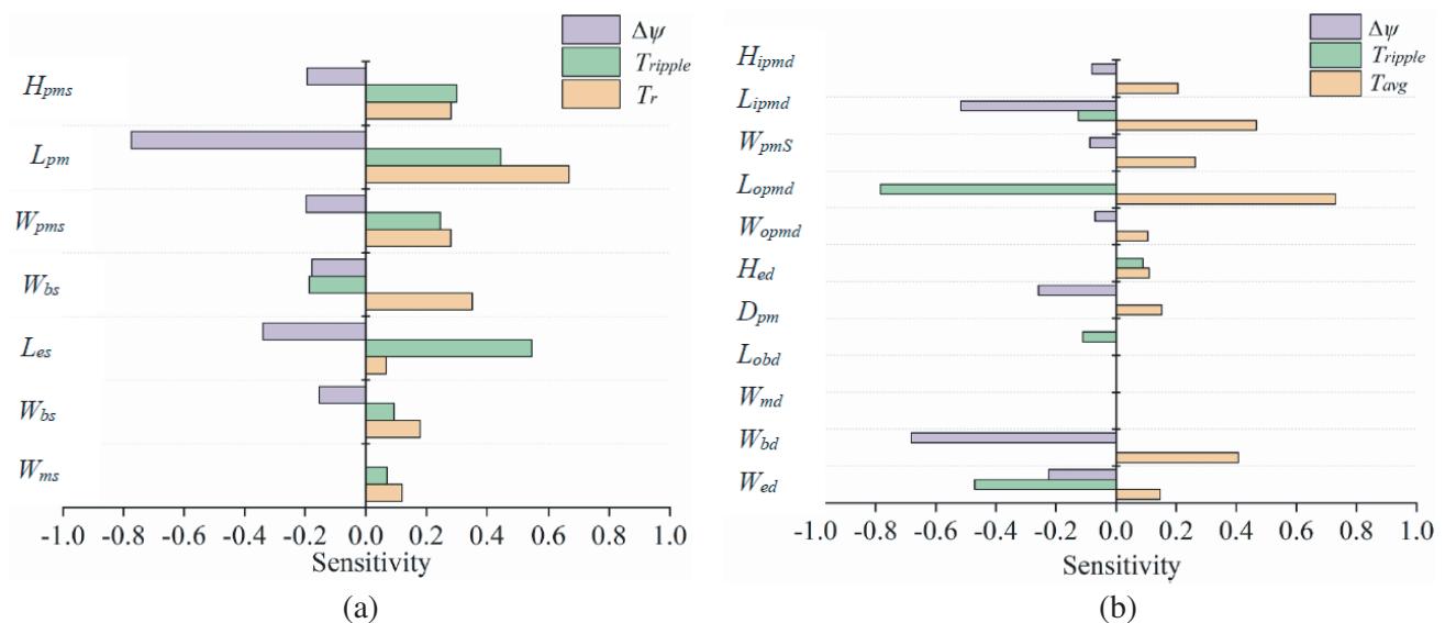
Figure 5. Sensitivity analysis. (a) SLPM-VLFM. (b) DLPM-VLFM.
