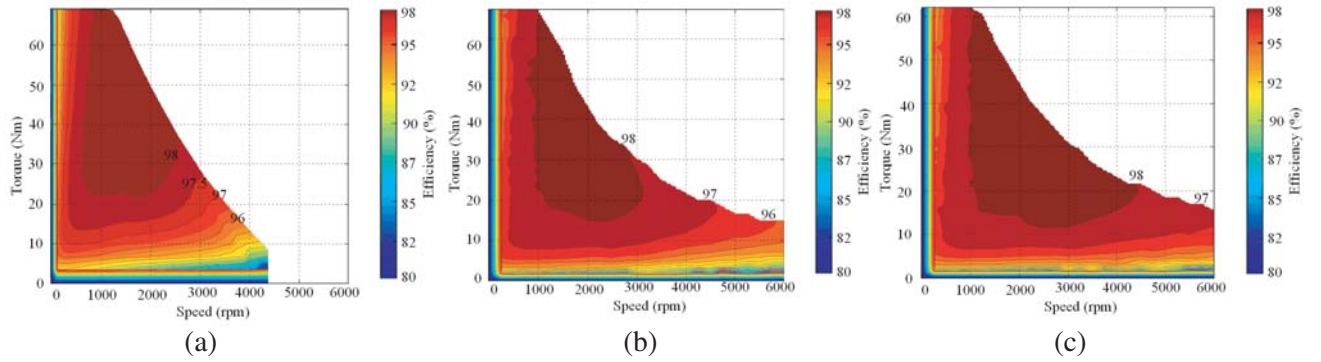
Figure 11. Efficiency maps of the three motors. (a) CIPMM. (b) SLPM-VLFM. (c) DLPM-VLFM.
