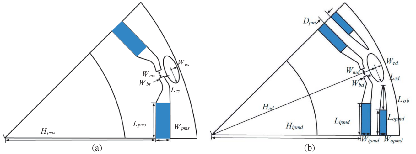
Figure 4. Parametric model. (a) SLPM-VLFM. (b) DLPM-VLFM.
