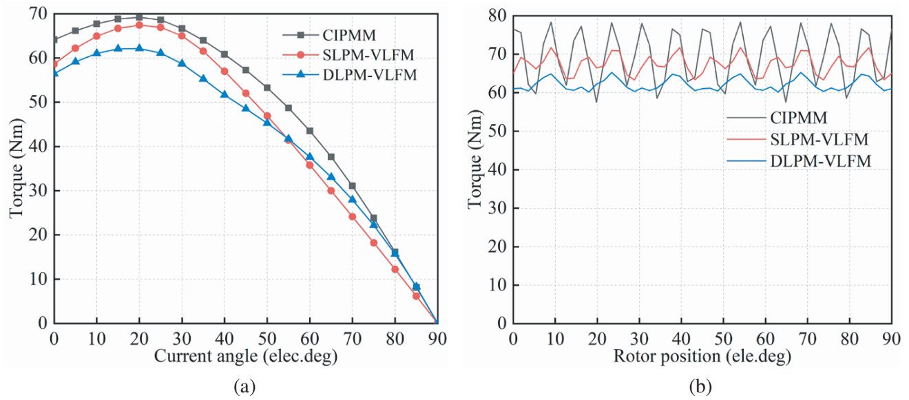
Figure 9. Torque characteristics of the three motors. (a) Torque versus current angles. (b) Output torque versus rotor position.
