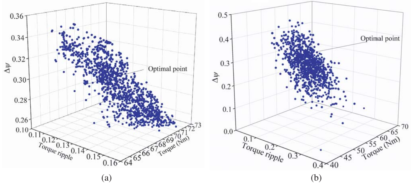
Figure 6. Optimization results of the two proposed motors. (a) SLPM-VLFM. (b) DLPM-VLFM.
