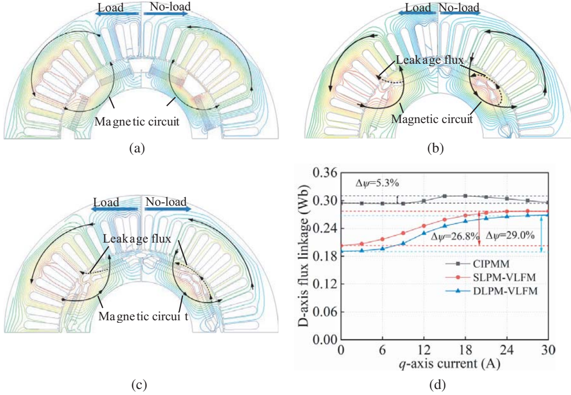
Figure 8. Flux characteristics. (a) Flux characteristics of CIPMM. (b) Flux characteristics of SLPM-VLFM. (c) Flux characteristics of DLPM-VLFM. (d) Relationship between q -axis current and d -axis flux linkage.
