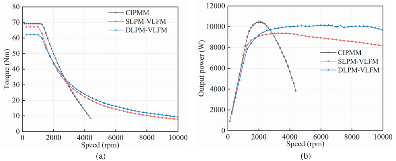
Figure 10. Performance comparisons of the three motors. (a) Torque-speed envelopes. (b) Output power-speed envelopes.
