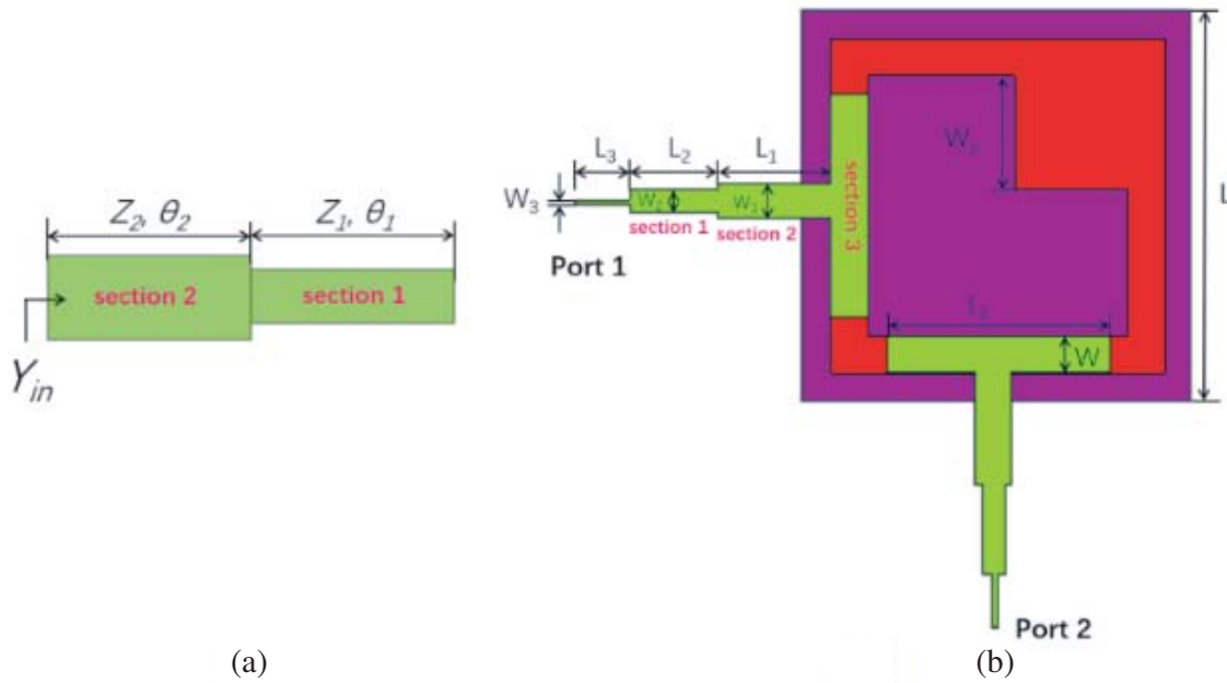
Figure 3. (a) Two section cascaded SIVFL for analyzing and (b) planar view with SIVFLs unfolding.
