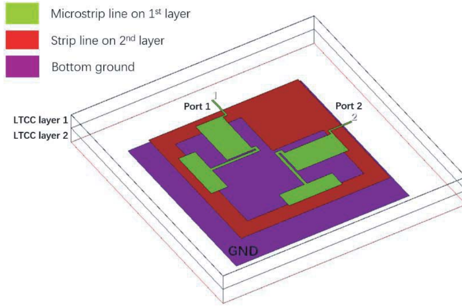
Figure 1. 3D structure of the proposed dual-mode BPF.
