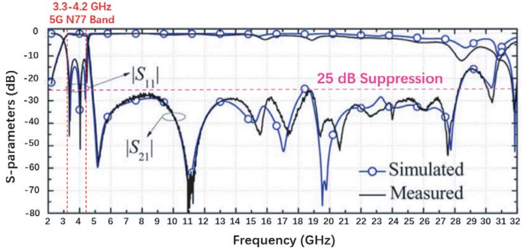
Figure 5. Simulated and measured results of proposed BPF.
