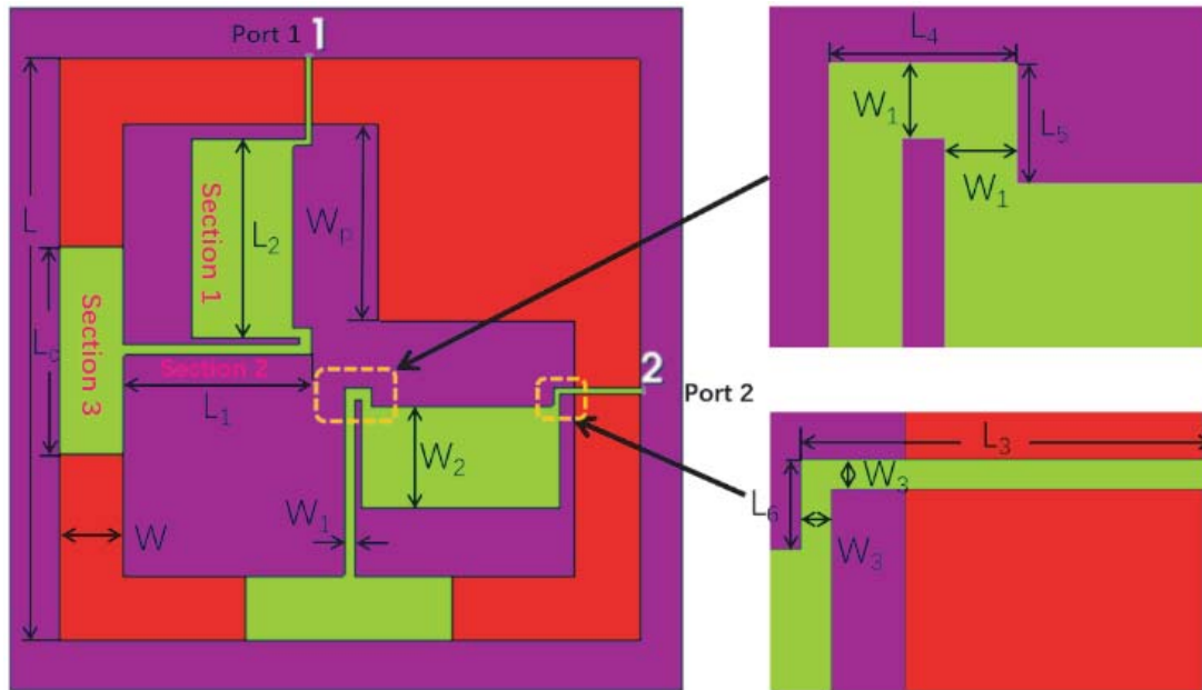
Figure 2. Planar view with parameters definitions.
