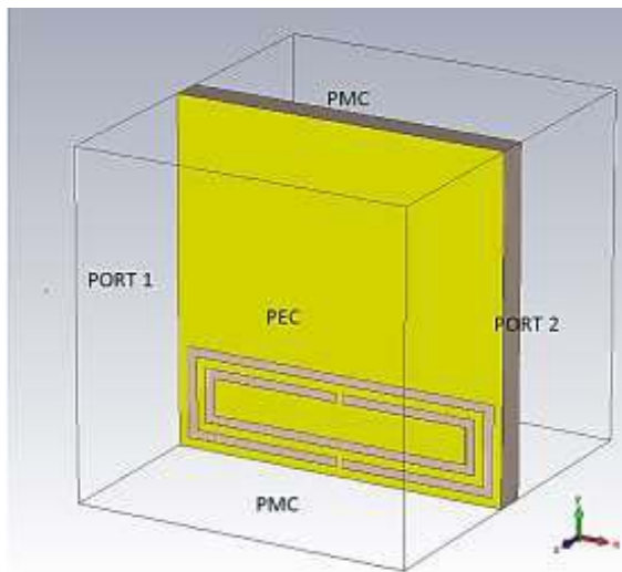
Figure 10. S parameter extraction set up.
