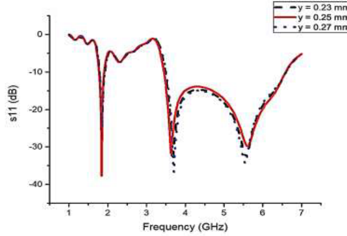
Figure 8. s_{11} evaluation for various values of y .
