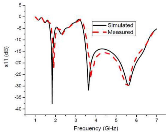
Figure 17. Simulated vs. measured s_{11} .
