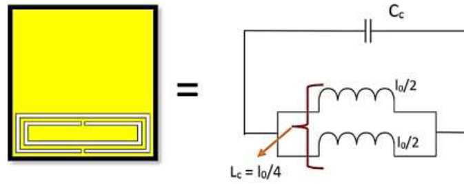
Figure 9. Equivalent circuit of CSRR.
