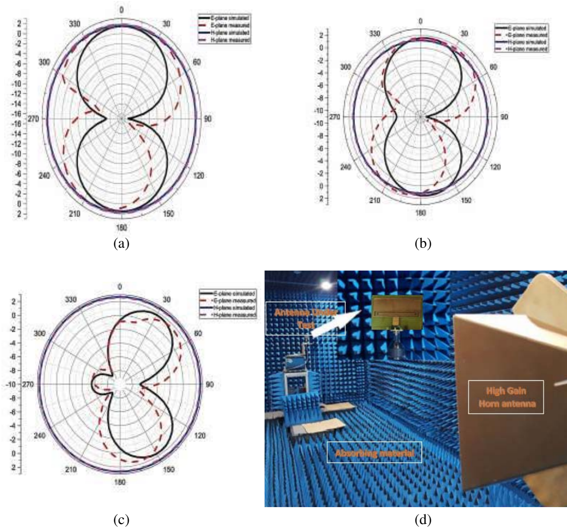
Figure 15. E plane and H plane (measured vs simulated) at the various resonating frequency and measurement setup. (a) 1.83 GHz, (b) 3.65 GHz, (c) 5.59 GHz, (d) chamber set up.
