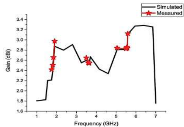
Figure 18. Measured and simulated gain comparison.
