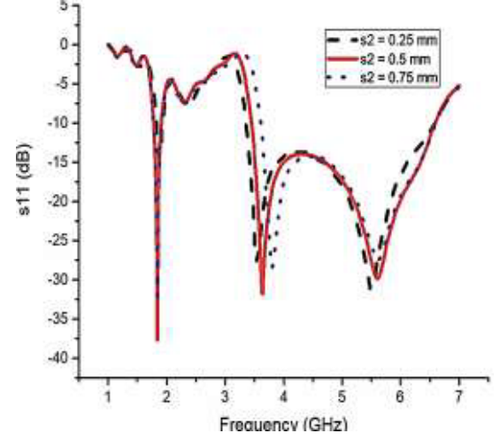
Figure 7. s_{11} evaluation for various values of s_2 .
