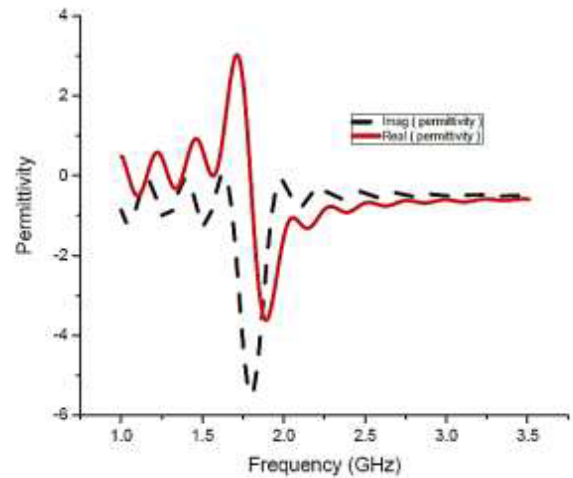
Figure 11. Negative permittivity of the proposed CSR.
