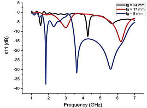
Figure 4. Ground length analysis.
