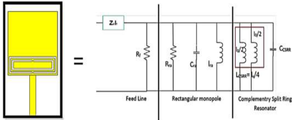
Figure 13. Equivalent circuit of the proposed antenna.
