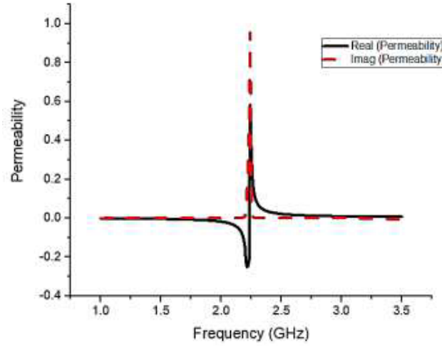
Figure 12. Negative permeability of the proposed CSRR.
