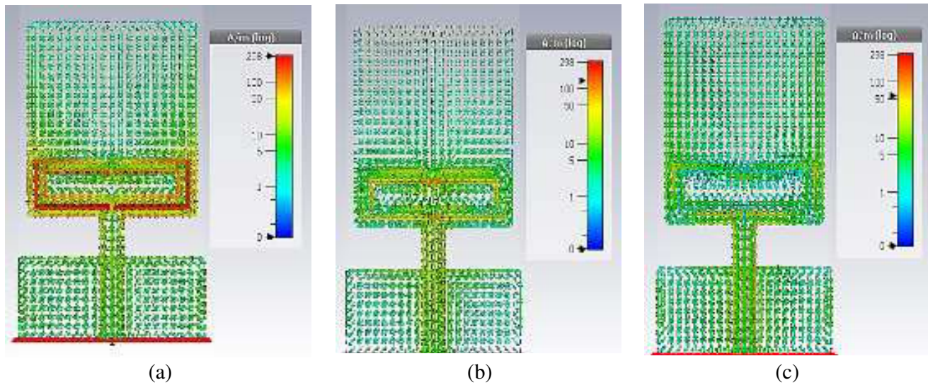
Figure 14. Surface current distribution at the various resonating frequency. (a) 1.83 GHz, (b) 3.65 GHz, (c) 5.59 GHz.
