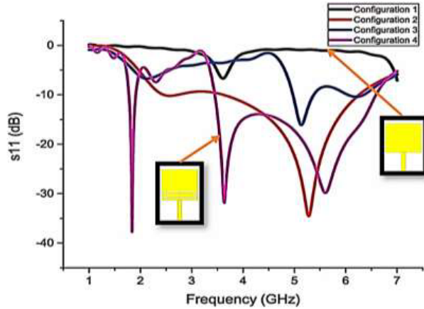
Figure 3. S_{11} comparison (Configuration 1 to 4).
