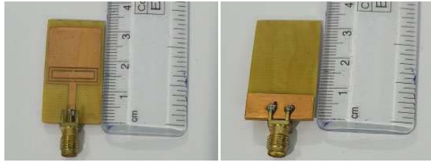
Figure 16. Fabricated prototype.
