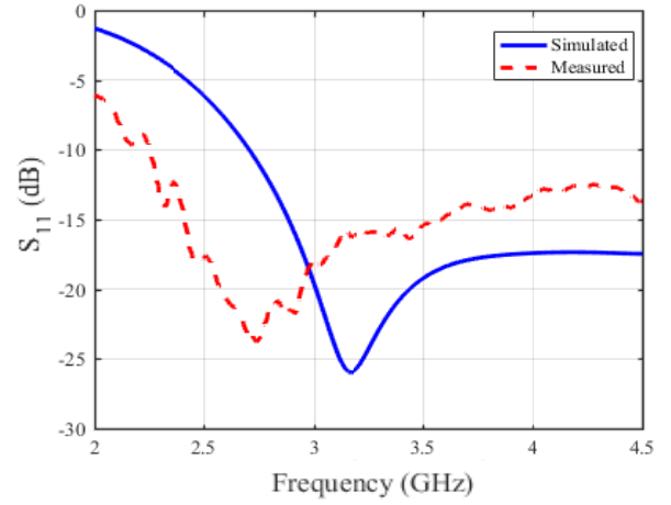
Figure 4. Simulated and measured S_{11} of the reader antenna.
