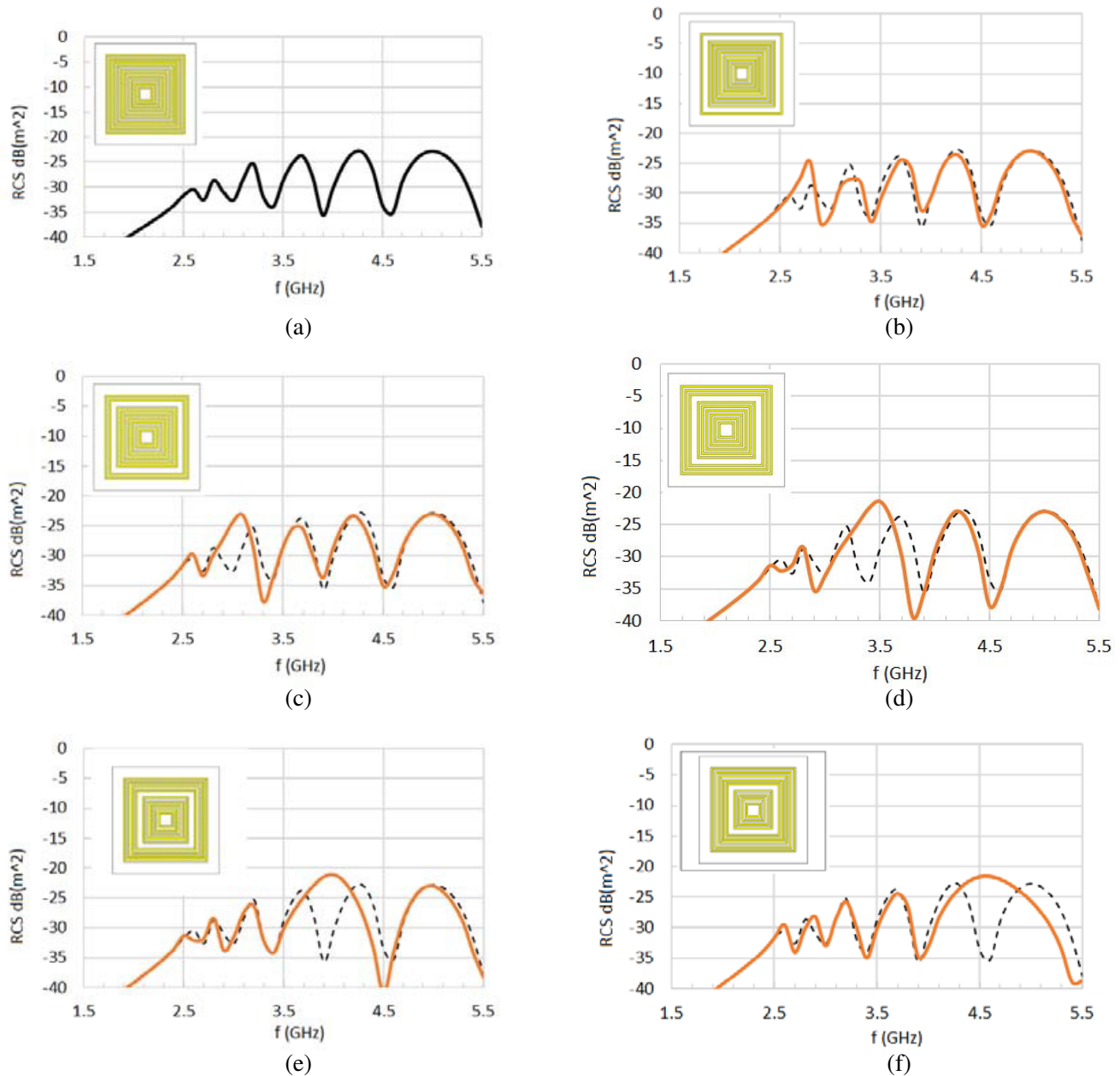
Figure 2. Monostatic RCS with normal incidence of the proposed RFID tag for different six configurations. Dashed line corresponds to the performance of the RFID tag with all rings.
