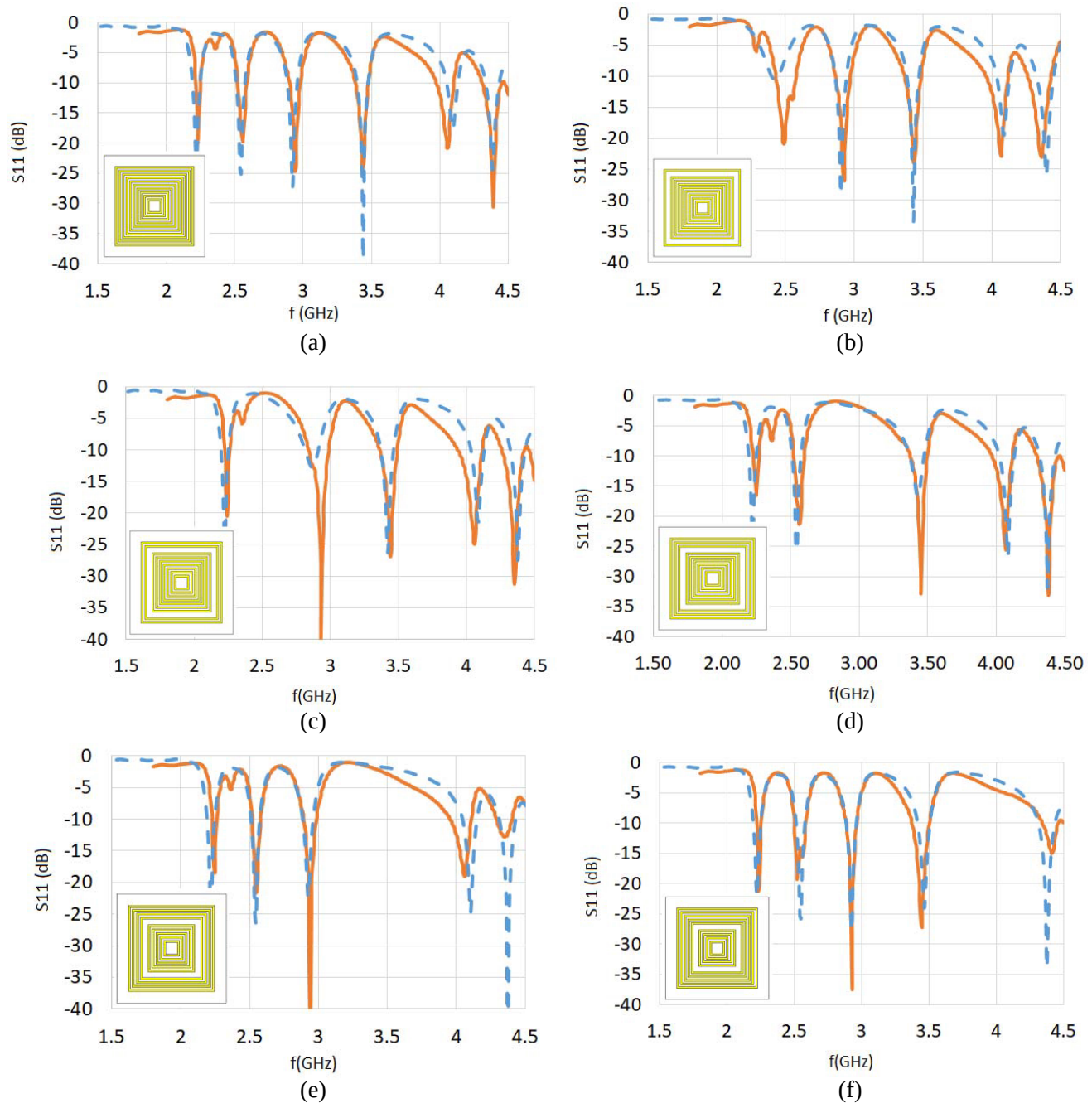
Figure 6. Measured and simulated reflection coefficients of the reader antenna for different RFID tag configurations. Dashed lines corresponds to the simulation results and solid lines corresponds to the measured results.
