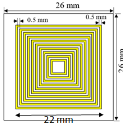
Figure 1. Geometry of the proposed RFID tag composed on concentric square rings on a dielectric slab.
