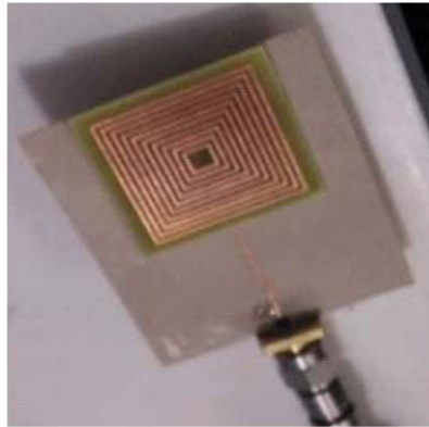
Figure 5. The proposed near field RFID tag identification configuration consisting of a wideband antenna in proximity of the RFID tag.
