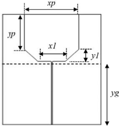
Figure 3. Geometry of the reader antenna.
