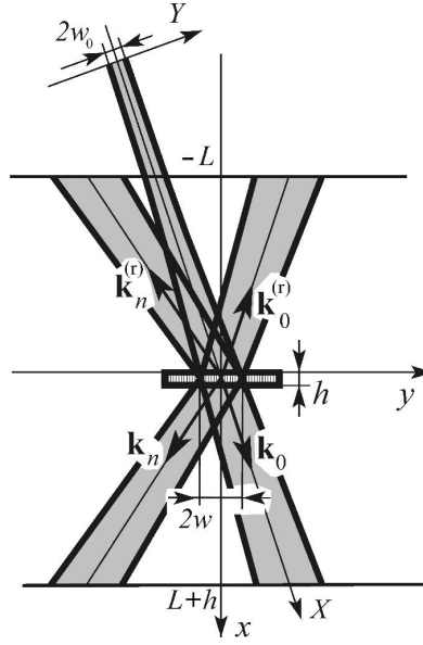
Figure 6. Diffraction of a Gaussian beam by a transmission dielectric grating. \mathbf{k}_n is the wave vectors of n th diffraction order, determining its direction of propagation.
