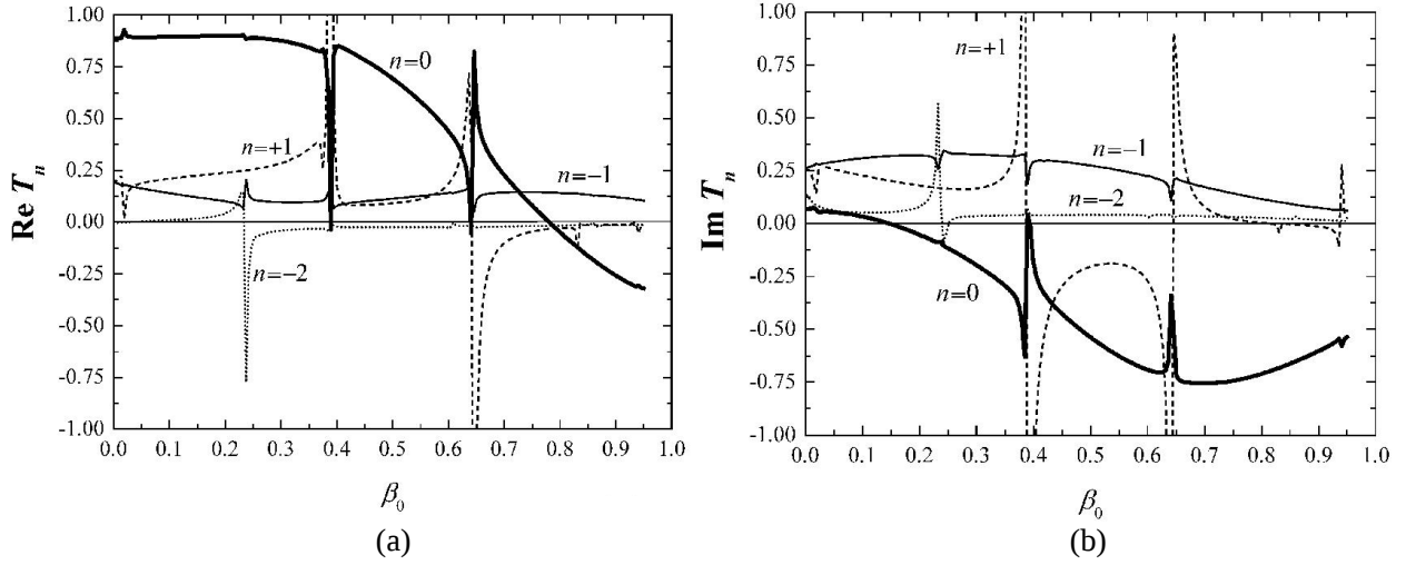
Figure 7. (a) Real and (b) imaginary parts of the complex amplitude transmission coefficient T_n of a planar sinusoidal grating for 4 diffraction orders as functions of the parameter \beta_0 of tangential propagation of the TE polarized plane incident wave.
