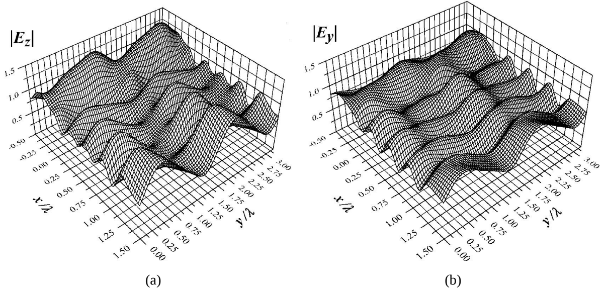
Figure 3. Spatial distribution pattern for the electric field amplitudes E_z and E_y of the TE and TM polarizations, respectively, in a planar sinusoidal grating without a substrate in the case of a plane diffracting wave.
