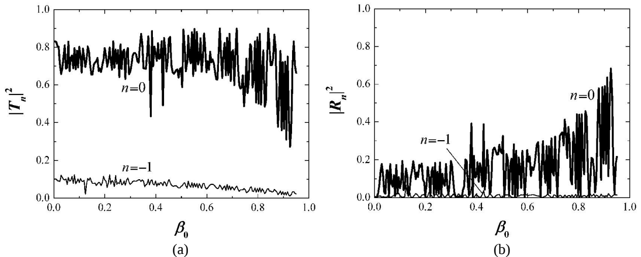
Figure 11. Intensities of the TE polarized (a) two transmitted |T_n|^2 and (b) two reflected |R_n|^2 radiation diffraction orders on the output of a planar sinusoidal grating located on a substrate of the thickness 10^3\lambda , in dependence of the parameter \beta_0 of incident plane wave tangential propagation.
