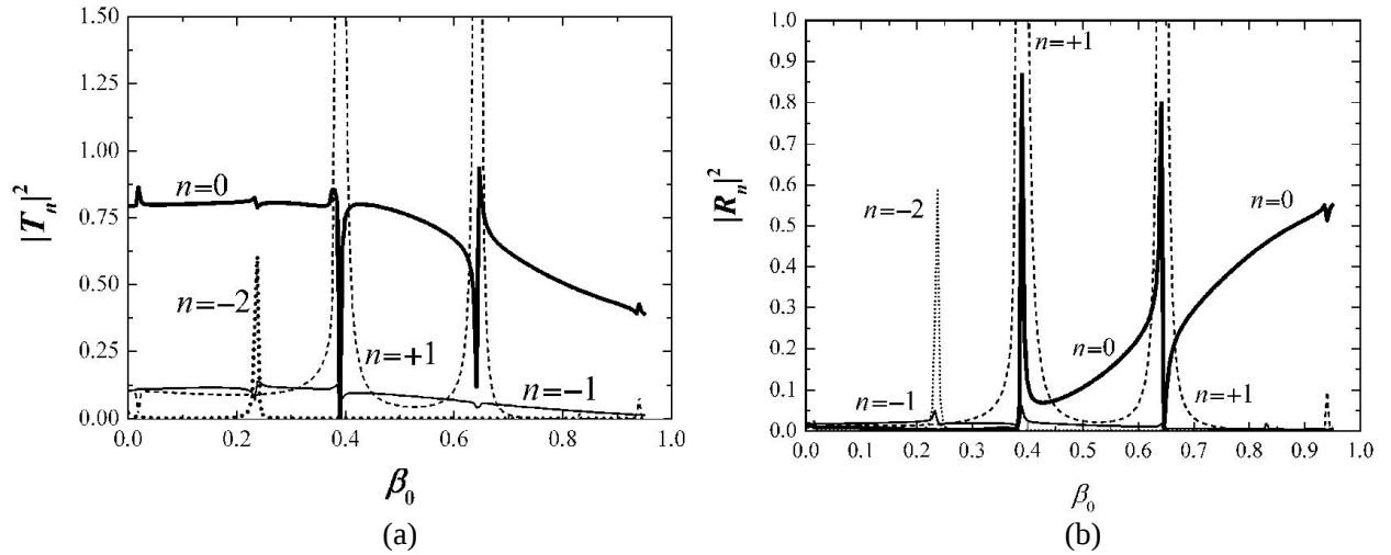
Figure 4. Intensities of the TE polarized (a) 4 transmitted |T_n|^2 and (b) 4 reflected |R_n|^2 radiation diffraction orders on the output of a planar sinusoidal grating without a substrate as functions of the parameter \beta_0 of incident wave tangential propagation.
