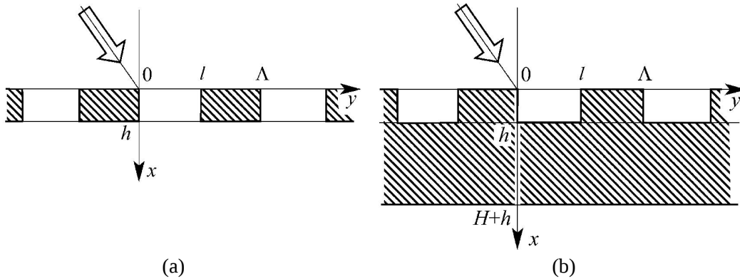
Figure 1. Simple binary relief grating (a) without and (b) with a substrate. h is the thickness of a grating, \Lambda is its spatial period, l is the length of an air groove between two neighbour rulings, H is the thickness of a substrate.
