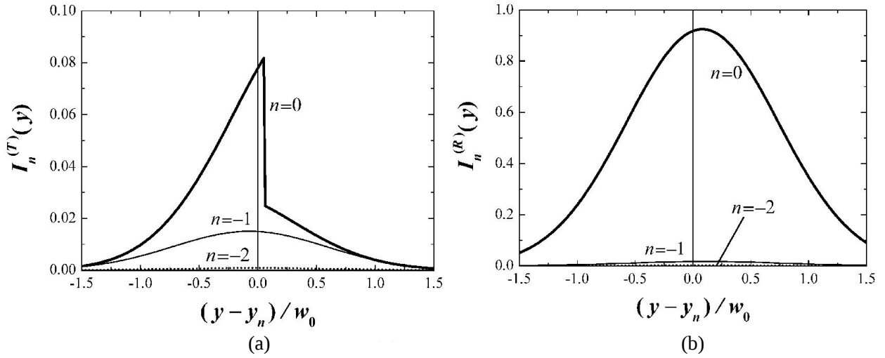
Figure 9. Transverse intensity structure of (a) transmitted I_n^{(T)}(y) and (b) reflected I_n^{(R)}(y) beams of various diffraction orders in the planes x = h + L and x = -L , respectively, computed relative to the middle of every beam y_n at the diffraction of the TE polarized beam with the parameter of tangential propagation \beta_0 = 0.64275 by a planar sinusoidal grating without a substrate.
