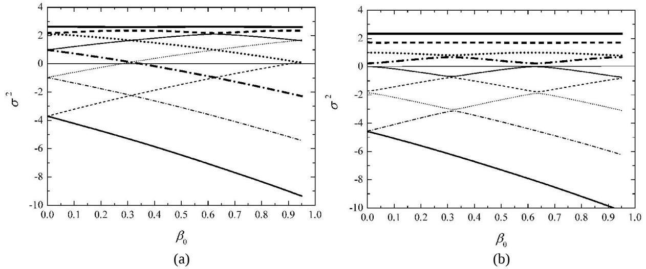
Figure 2. Dependence of eigenvalues of the matrix (11) on the parameter of tangential propagation of incident TE wave for (a) a planar sinusoidal and (b) a rectangular relief grating with the thickness h = 1.25\lambda , the spatial period \Lambda = 1.6\lambda and the index of refraction of a dielectric n_g = 1.6 .
