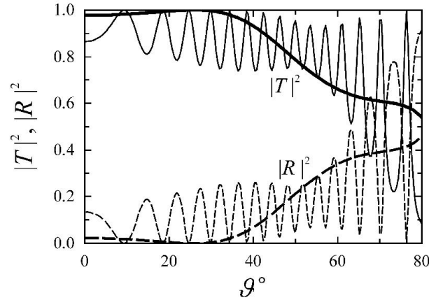
Figure 13. Intensities of transmitted (solid lines) and reflected (dashed curves) waves at the incidence of the TE polarized plane wave on a thin dielectric layer without (thick lines) and with (thin curves) a substrate of the thickness 20\lambda . The thickness of a layer h = 1.2\lambda , its real dielectric permittivity \varepsilon = 1.75 , permittivity of a substrate \varepsilon_s = 2.5 .
