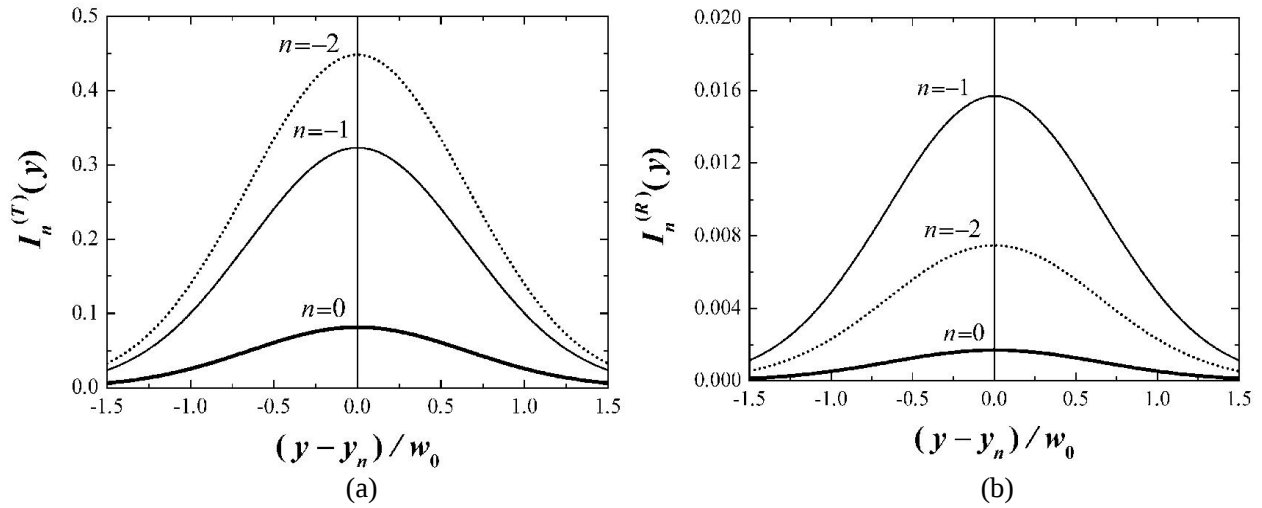
Figure 10. Transverse intensity structure of (a) transmitted I_n^{(T)}(y) and (b) reflected I_n^{(R)}(y) beams of various diffraction orders in the planes x = h + L and x = -L , respectively, computed relative to the middle of every beam y_n at the diffraction of the TE polarized beam with the parameter of tangential propagation \beta_0 = 0.64275 by a rectangular relief grating without a substrate.
