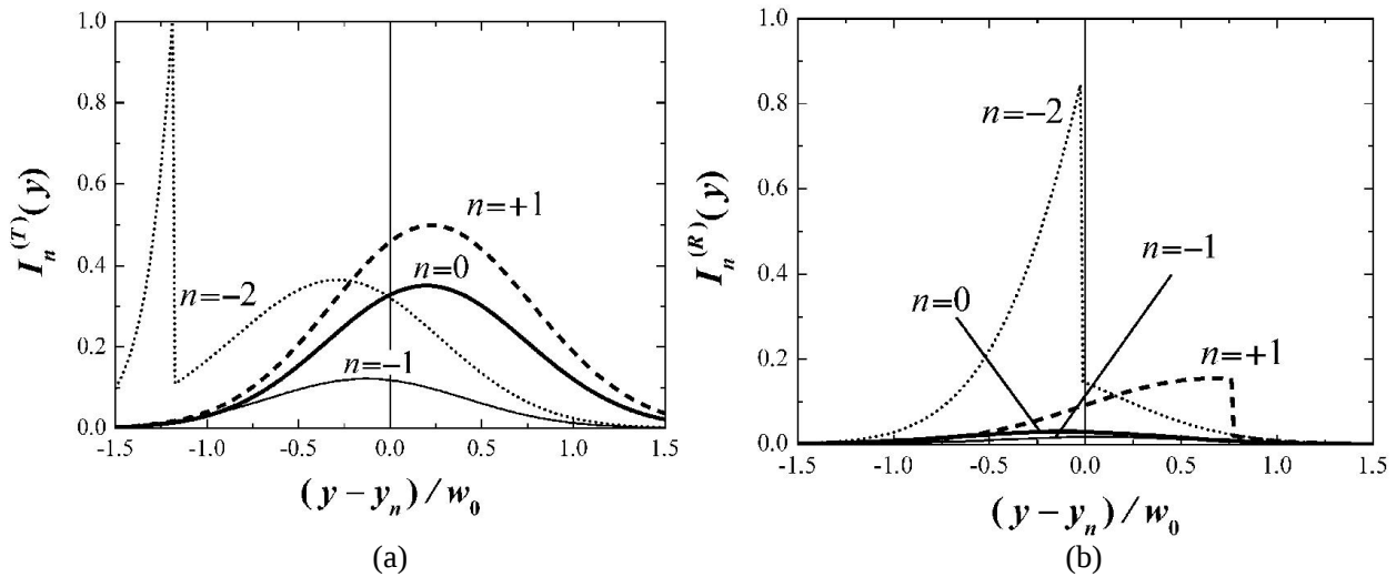
Figure 15. Transverse intensity structure of (a) transmitted I_n^{(T)}(y) and (b) reflected I_n^{(R)}(y) beams of various diffraction orders in the planes x = h + H + L and x = -L , respectively, computed relative to the middle of every beam y_n at the diffraction of the TE polarized beam with the parameter of tangential propagation \beta_0 = 0.320 by a rectangular relief grating located on a substrate with the thickness 10^3\lambda .
