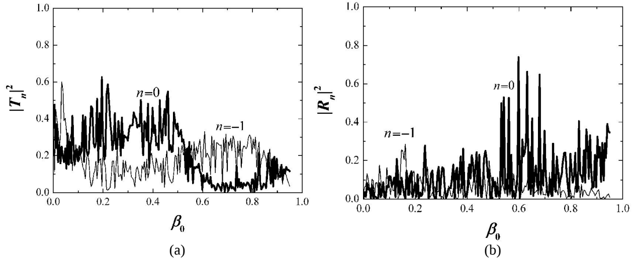
Figure 12. Intensities of the TE polarized (a) two transmitted |T_n|^2 and (b) two reflected |R_n|^2 radiation diffraction orders on the output of a rectangular relief grating located on a substrate of the thickness 10^3\lambda , in dependence of the parameter \beta_0 of incident plane wave tangential propagation.
