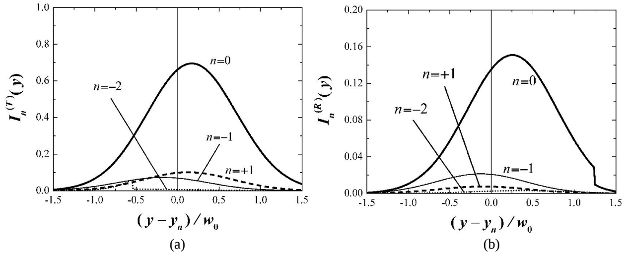
Figure 14. Transverse intensity structure of (a) transmitted I_n^{(T)}(y) and (b) reflected I_n^{(R)}(y) beams of various diffraction orders in the planes x = h + H + L and x = -L , respectively, computed relative to the middle of every beam y_n at the diffraction of the TE polarized beam with the parameter of tangential propagation \beta_0 = 0.320 by a planar sinusoidal grating located on a substrate with the thickness 10^3\lambda .
