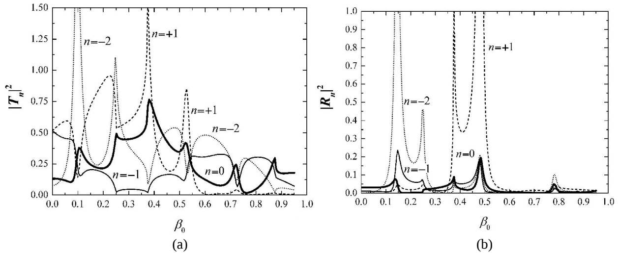
Figure 5. Intensities of the TE polarized (a) 4 transmitted |T_n|^2 and (b) 4 reflected |R_n|^2 radiation diffraction orders on the output of a rectangular relief grating without a substrate as functions of the parameter \beta_0 of incident wave tangential propagation.
