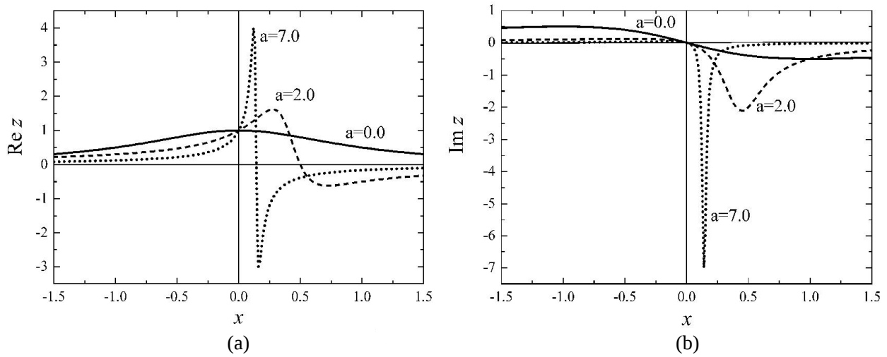
Figure 8. (a) Real and (b) imaginary parts of the inversely proportional function z = [1 + i(1 + ia)x]^{-1} at various values of the parameter a .
