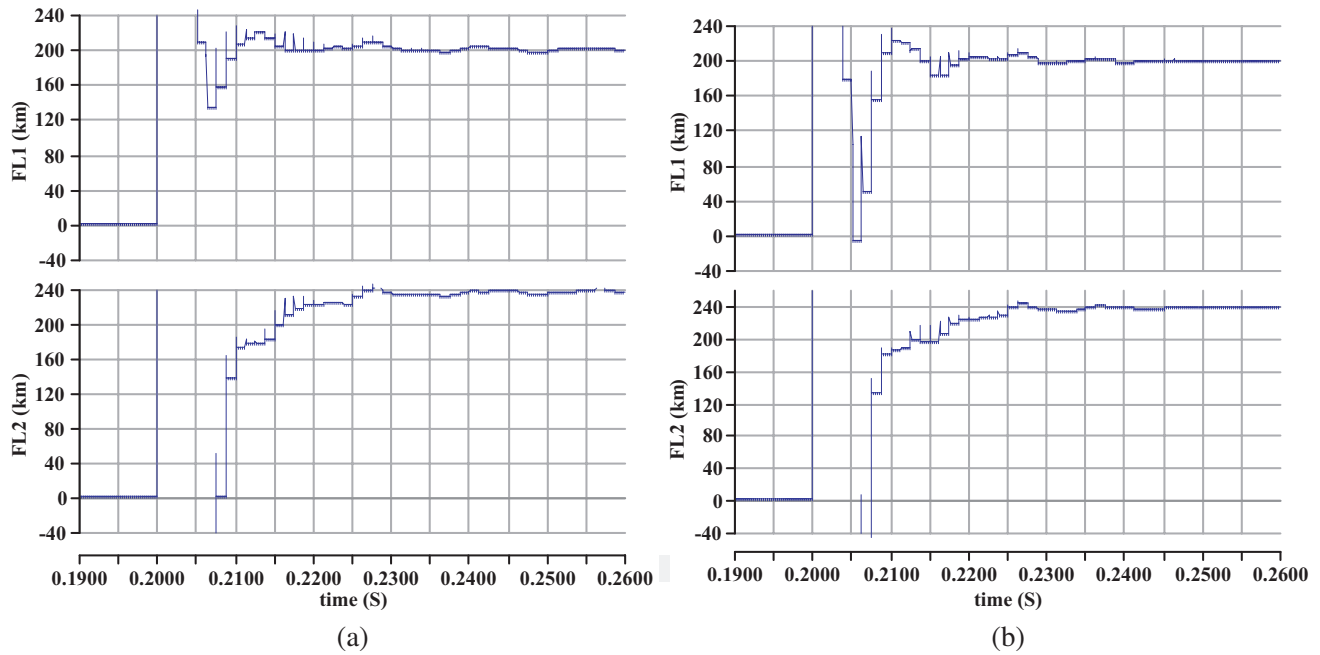
Figure 10. The partially enlarged view of the simulation results with fault resistance. (a) SPG with the resistance 200\ \Omega . (b) DPH with the resistance 50\ \Omega .
