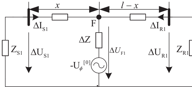
Figure 2. Positive sequence fault component diagram.
