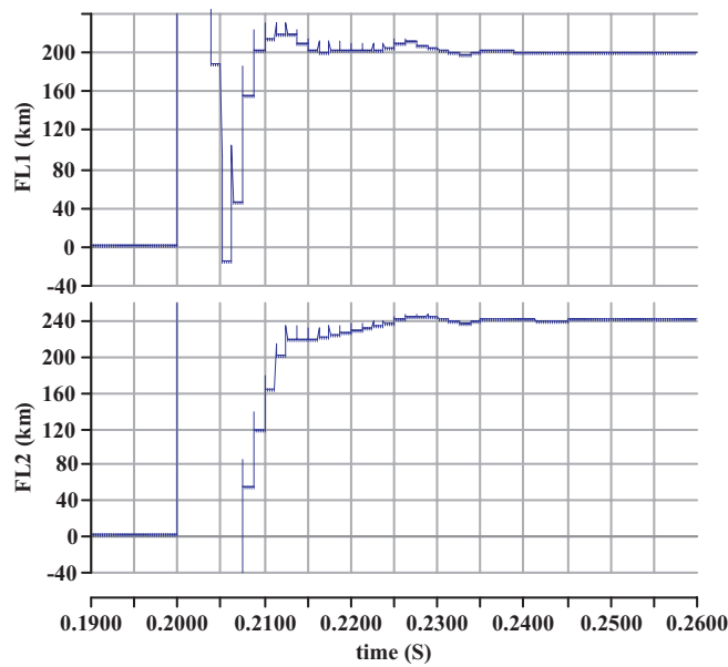
Figure 11. The partially enlarged view of TPH with the resistance 50\ \Omega .
