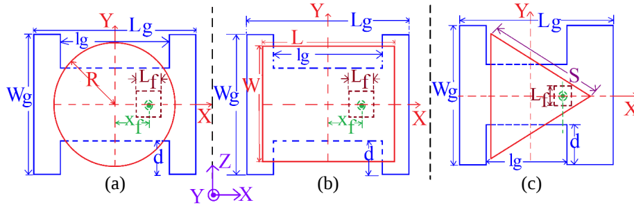
Figure 7. (a) CMSA, (b) SMSA, and (c) ETMSA backed by H-shape ground plane.
