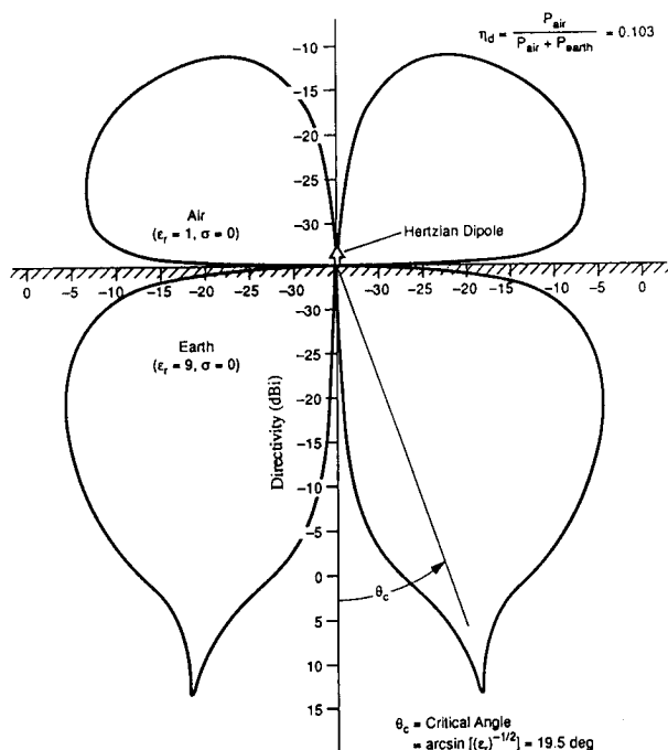
Figure 3.3 Directivity (in any Azimuthal plane) of a vertically polarized Hertzian dipole at zero height above dielectric Earth, \epsilon_r = 9 .
