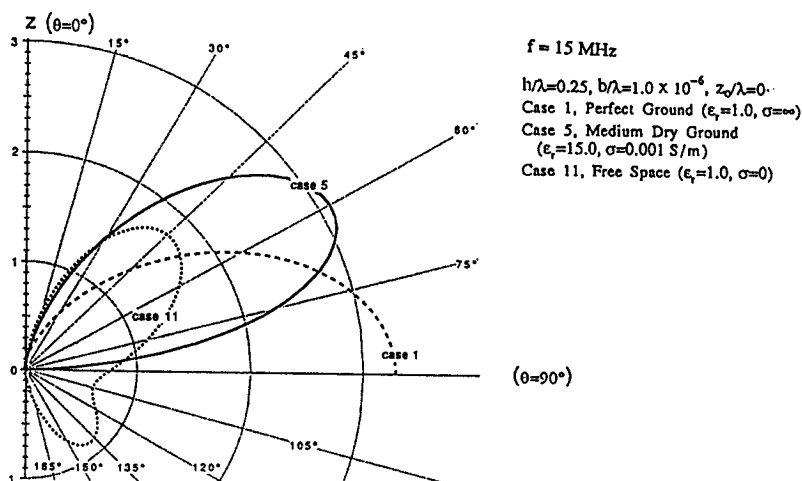
Figure 2.3 Numeric directivity polar plot, 2\pi a/\lambda = 3.0 . ( f=15 \text{ MHz} , h/\lambda = 0.25, b/\lambda = 1.0 \times 10^{-6}, Z_0/\lambda = 0 . Case 1: Perfect Ground ( \epsilon_0 = 1.0, \delta = \infty ), Case 5: Medium Dry Ground ( \epsilon_0 = 15.0, \delta = 0.001 \text{ s/m} ), Case 11: Free Space ( \epsilon_0 = 1.0, \delta = 0 ).)
