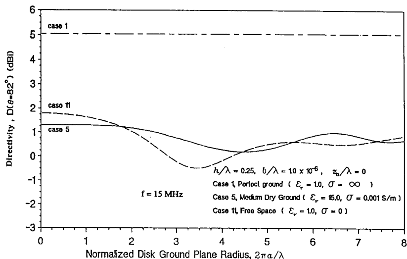
Figure 2.9 Directivity at eight degrees above the horizon
