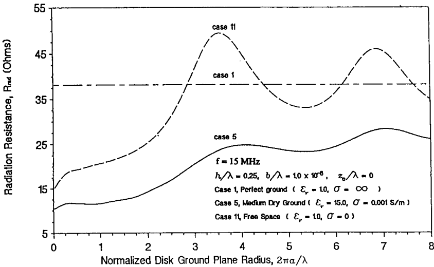
Figure 3.6 Radiation resistance of a quarter-wave monopole element on a disk ground plane resting on medium dry ground
