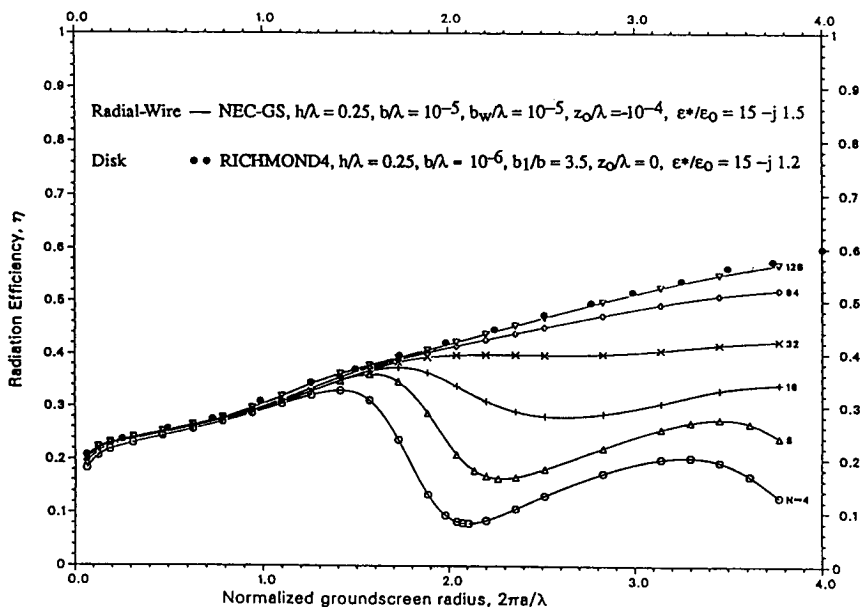
Figure 3.5 Radiation efficiency of a quarter-wave monopole element with radial-wire and disk ground planes on or just above medium dry Earth.
