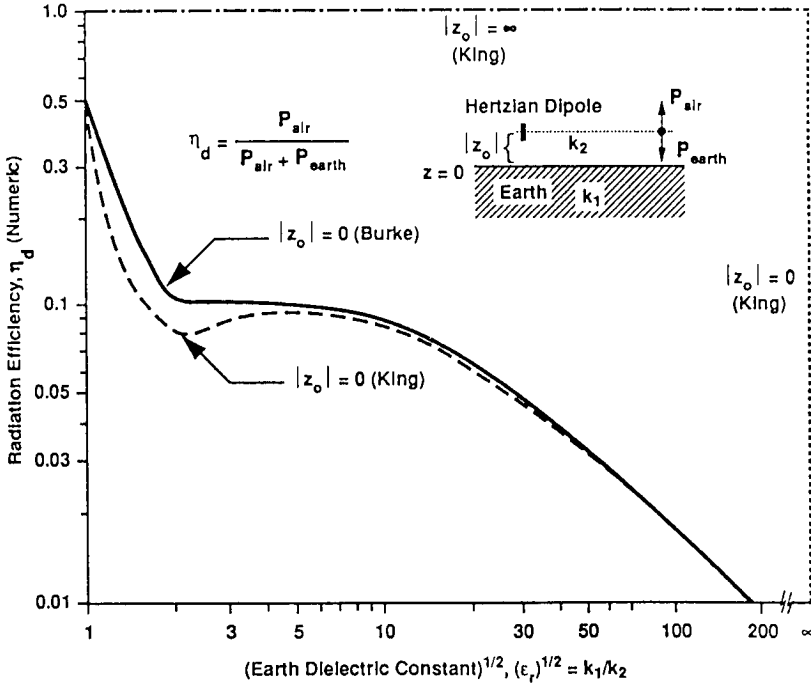
Figure 3.1 Radiation efficiency of vertically polarized Hertzian dipole above dielectric Earth, |z_0|/\lambda = 0 and |z_0|/\lambda = \infty .
