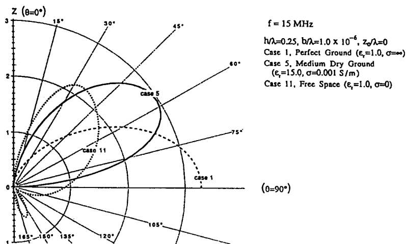
Figure 2.5 Numeric directivity polar plot, 2\pi a/\lambda = 5.0 . ( f = 15 \text{ MHz} , h/\lambda = 0.25, b/\lambda = 1.0 \times 10^{-6}, Z_0/\lambda = 0 . Case 1: Perfect Ground ( \epsilon_0 = 1.0, \delta = \infty ), Case 5: Medium Dry Ground ( \epsilon_0 = 15.0, \delta = 0.001 \text{ s/m} ), Case 11: Free Space ( \epsilon_0 = 1.0, \delta = 0 ).)
