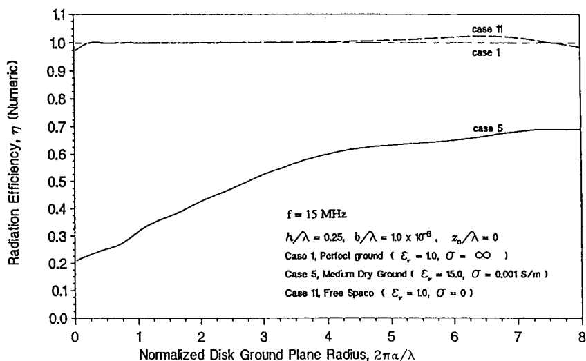
Figure 3.4 Radiation efficiency of a quarter-wave element on a disk ground plane resting on medium dry ground.
