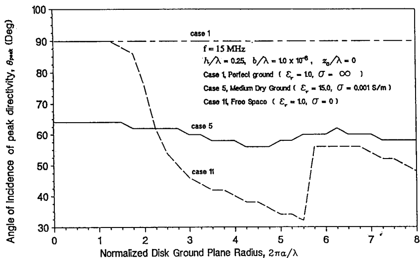
Figure 2.8 Angle of incidence of peak directivity
