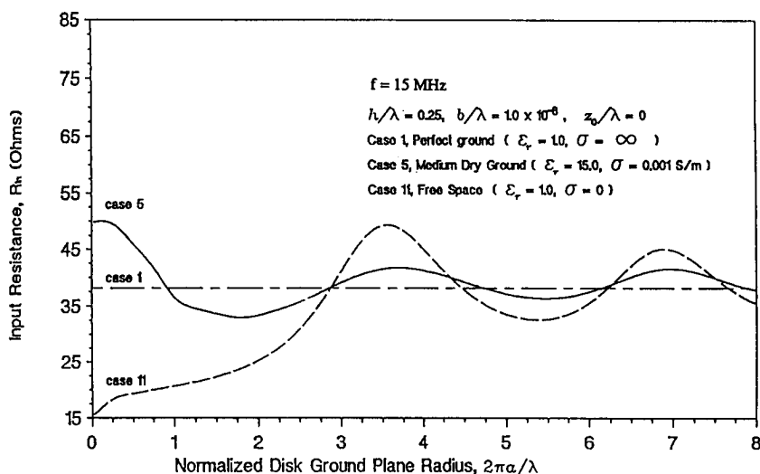
Figure 3.7 Input resistance of a quarter-wave monopole element on a disk ground plane resting on medium dry ground
