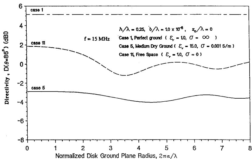
Figure 2.11 Directivity at four degrees above the horizon
