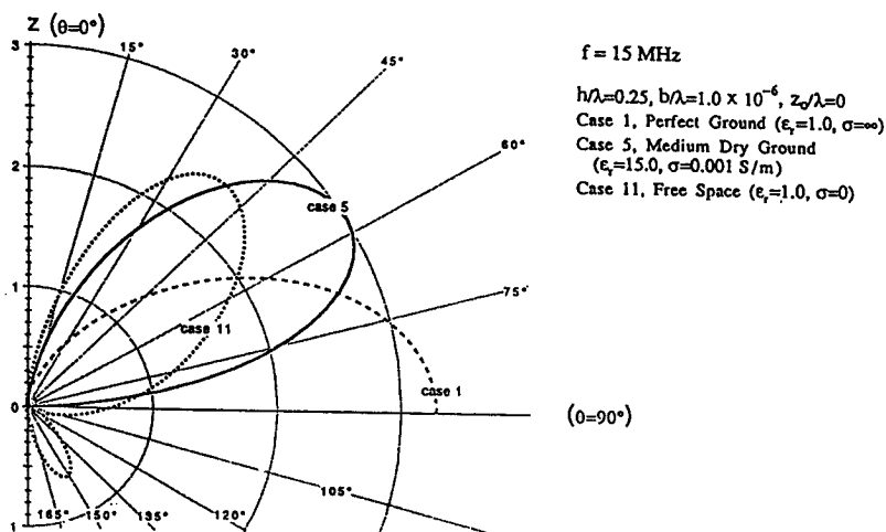
Figure 2.4 Numeric directivity polar plot, 2\pi a/\lambda = 4.0 . ( f=15 \text{ MHz} , h/\lambda = 0.25, b/\lambda = 1.0 \times 10^{-6}, Z_0/\lambda = 0 . Case 1: Perfect Ground ( \epsilon_0 = 1.0, \delta = \infty ), Case 5: Medium Dry Ground ( \epsilon_0 = 15.0, \delta = 0.001 \text{ s/m} ), Case 11: Free Space ( \epsilon_0 = 1.0, \delta = 0 ).)
