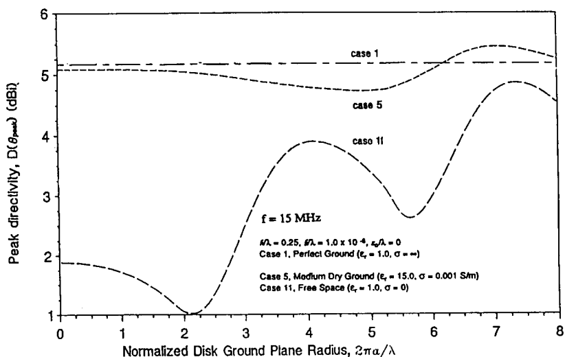
Figure 2.7 Peak directivity
