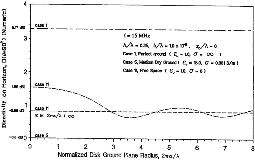
Figure 2.12 Directivity at two degrees above the horizon
