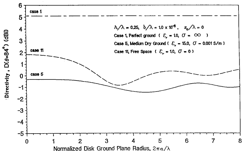
Figure 2.10 Directivity at six degrees above the horizon
