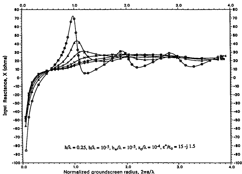
Figure 3.10 Input reactance of a quarter-wave monopole element on a radial-wire groundscreen; z_0/\lambda = 10.4 , \epsilon^*/\epsilon_0 = 15 - j1.5
