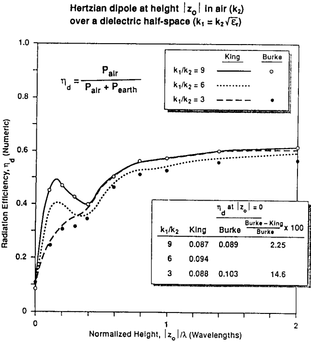
Figure 3.2 Radiation efficiency of vertically polarized Hertzian dipole above dielectric Earth, 0 \leq |z_0|/\lambda \leq 2 .
