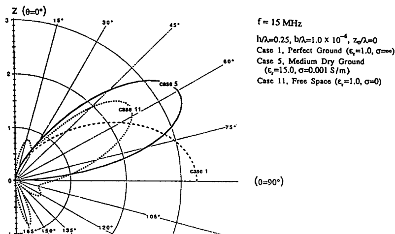
Figure 2.6 Numeric directivity polar plot, 2\pi a/\lambda = 6.5 . ( f = 15 \text{ MHz} , h/\lambda = 0.25, b/\lambda = 1.0 \times 10^{-6}, Z_0/\lambda = 0 . Case 1: Perfect Ground ( \epsilon_0 = 1.0, \delta = \infty ), Case 5: Medium Dry Ground ( \epsilon_0 = 15.0, \delta = 0.001 \text{ s/m} ), Case 11: Free Space ( \epsilon_0 = 1.0, \delta = 0 ).)
