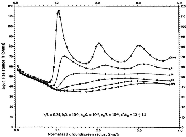
Figure 3.9 Input resistance of a quarter-wave monopole element on a radial-wire groundscreen; z_0/\lambda = 10.4, \epsilon^*/\epsilon_0 = 15 - j1.5
