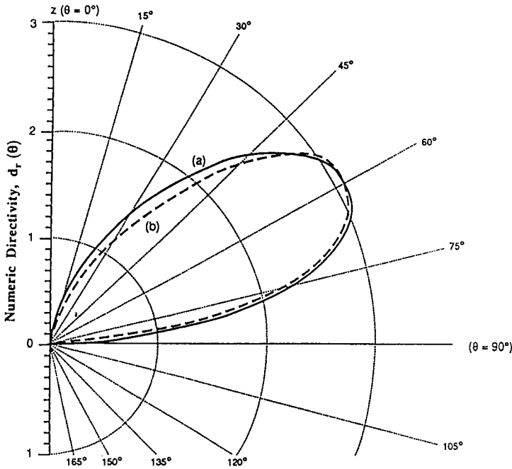
Figure 2.15 Numeric directivity of a quarter-wave element on a disk ground plane resting on medium dry ground, 2\pi a/\lambda = 3.0 . (a) Richmond's method-of-moments; (b) 10 \cos \theta \sin^3 \theta .
