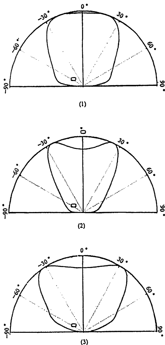
Figure 4. The radiation pattern of dipole antenna in a bi-isotropic two-layer geometry. H_1 = 0.03\text{m} , H_3 = 0.01\text{m} , H_0/\lambda = 0.3333 , \phi = 0, 90^\circ , \epsilon_2 = 2\epsilon_3 = 2.5\epsilon_0 (1) \epsilon_4 = 5.0\epsilon_0 , \xi_{e2} = \xi_{e3} = 2\xi_{m2}^* = 2\xi_{m3}^* = i3.0 \times 10^{-11} , \xi_{e4} = 2\xi_{m4}^* = i3.0 \times 10^{-10} . (2) \epsilon_4 = 5.0\epsilon_0 , \xi_{e2} = \xi_{e3} = 0.1\xi_{m2}^* = 0.1\xi_{m3}^* = i3.0 \times 10^{-11} , \xi_{e4} = 0.1\xi_{m4}^* = i3.0 \times 10^{-10} . (3) \epsilon_4 = \epsilon_0 , \xi_{e2} = \xi_{m2}^* = i3.0 \times 10^{-11} , \xi_{e4} = \xi_{m4}^* = 0 .
