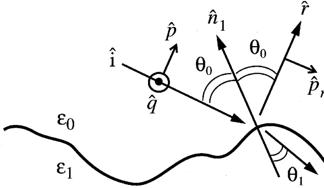
Figure 4. Reflection coefficients.
