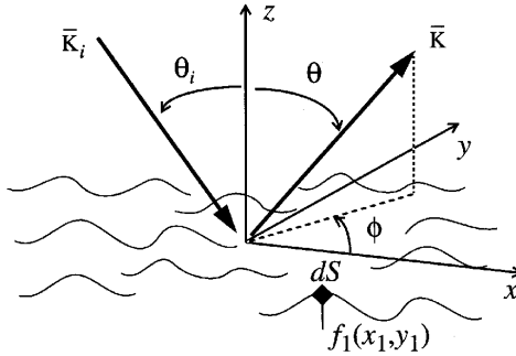
Figure 2. Rough surface is given by z = f_1(x_1, y_1) , and the surface element dS is at \bar{r}_1 = x_1\hat{x} + y_1\hat{y} + f_1(x_1, y_1)\hat{z} . \bar{K}_i = k\hat{i} and \bar{K} = k\hat{o} .
