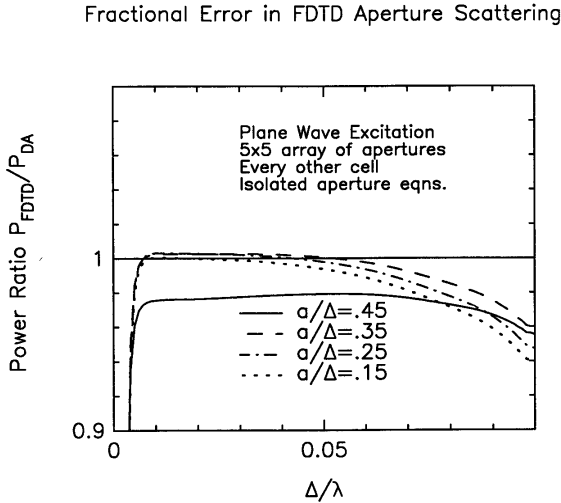
Figure 5. Transmitted power through 5 \times 5 array of circular apertures. Aperture in every other cell. Isolated aperture correction.
