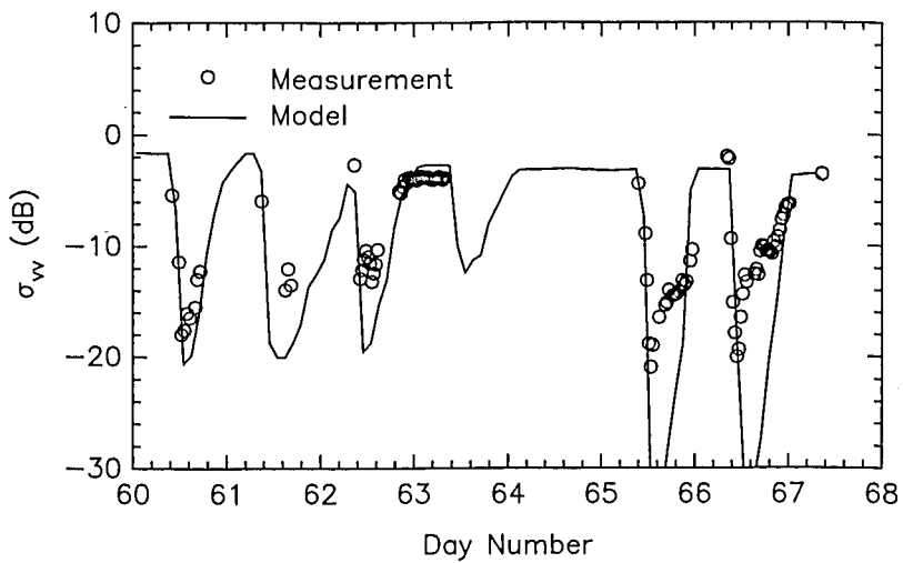
Figure 7. Temporal variations of backscatter in vv polarization at 35 GHz and 60° incident angle. Circles are measured data from Reference [16] and solid curve is DMRT simulation with snow parameters provided by SNTHERM model.
