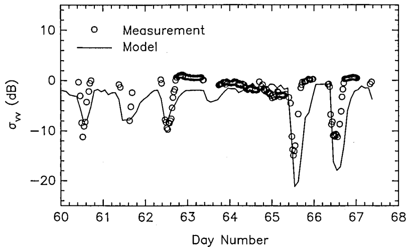
Figure 8. Temporal variations of backscatter in vv polarization at 95 GHz and 60° incident angle. Circles are measured data from Reference [16] and solid curve is DMRT simulation with snow parameters provided by SNTHERM model.
