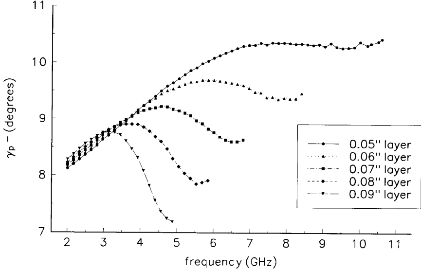
Figure 14. Phase front angles inside the layers.
