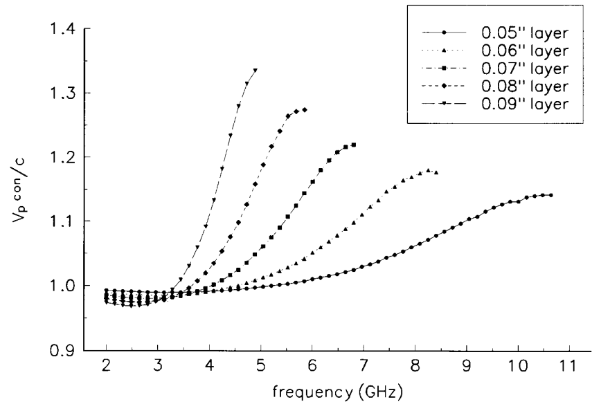
Figure 19. Conventional phase velocity.
