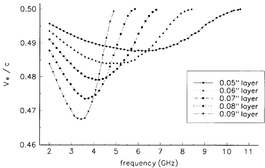
Figure 21. Energy velocity outside the layers.
