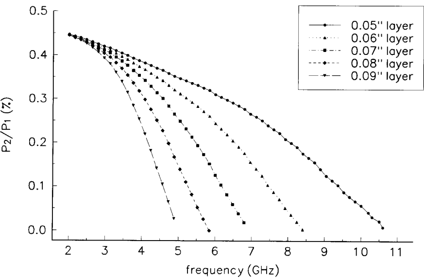
Figure 34. P_2/P_1 ratio.
