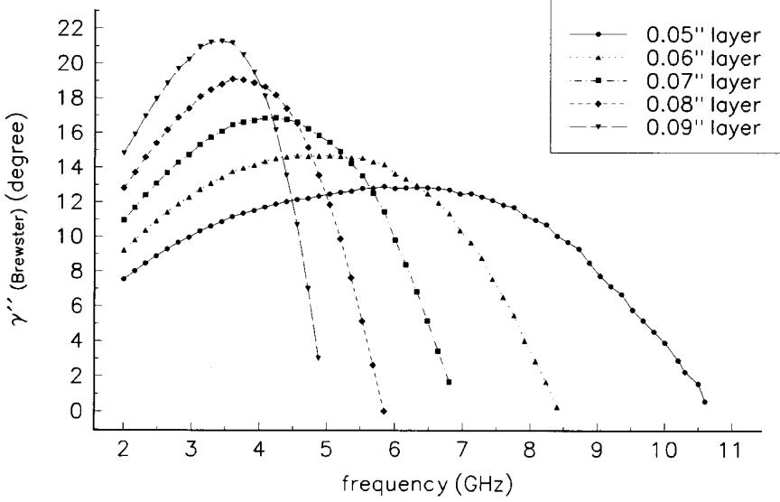
Figure 13. Brewster angle (Imaginary part).
