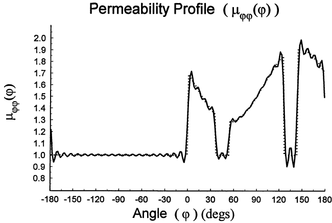
Figure 13. Plots of the relative permeability function \mu_{\phi\phi}(\rho, \phi) (exact ( dotted line ) and Fourier series representation ( solid line )) for the same case as described in Fig. 10 are shown.
