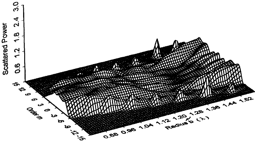
Figure 8. The scattered order power that occurs when a plane wave impinges on a uniform dielectric shell (see Fig. 1, \varepsilon_1 = 1.5 , \varepsilon_2 = 2.5 , \varepsilon_3 = 1. , \mu = 1. ) rather than an anisotropic half shell is shown.
