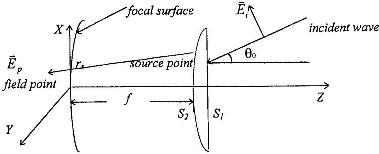
Figure 1. Geometry of symmetric focusing lens.
