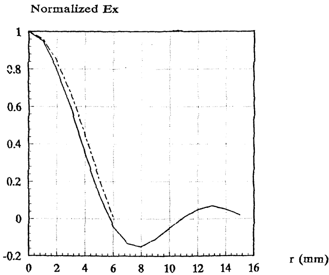
Figure 3. The fields comparison dash line-field in the aperture of horn; solid line-field in the axial region of focal plane.
