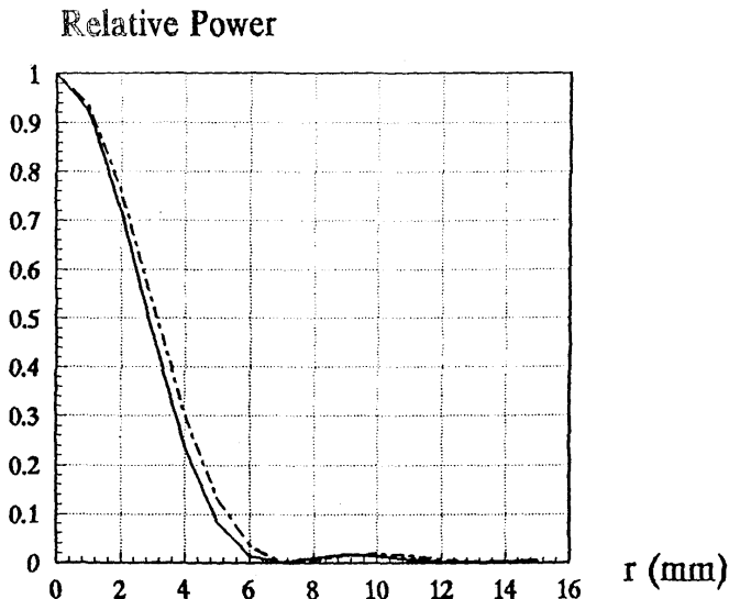
2c. Focal length f = 350 mm, f/D = 1.75 .
