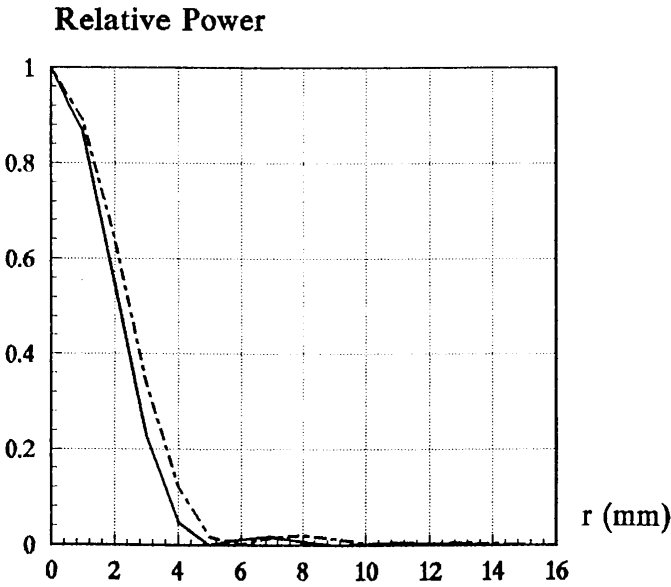
2b. Focal length f = 260 mm, f/D = 1.3 .
