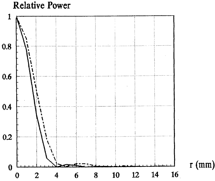
2a. Focal length f = 200 mm, f/D = 1.0 .
