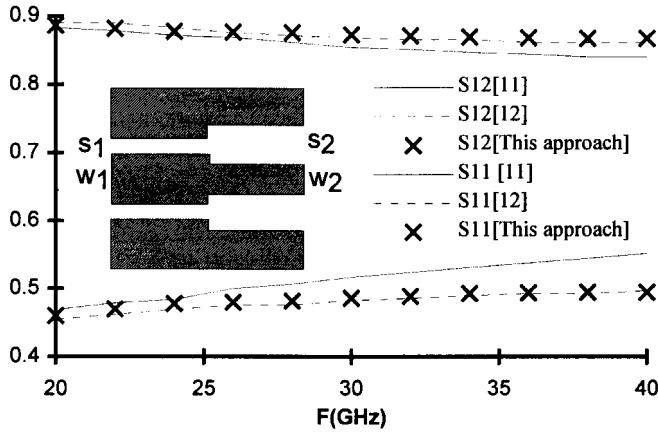
Figure 6. S -parameters of a simple step discontinuity in a coplanar wave guide; Dimensions: s_1 = 0.1 mm, s_2 = 0.4 mm, w_1 = 0.4 mm, w_2 = 0.1 mm, dielectric constant \varepsilon = 9.6 and thickness h = 0.254 mm.
