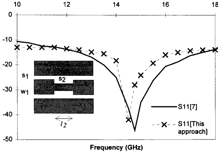
Figure 5. S_{11} -parameter of a double step discontinuity in a coplanar circuit; Dimensions: s_1 = 0.2 mm, w_1 = 0.5 mm, s_2 = 0.35 mm, l_2 = 4.36 mm, h = 0.635 mm, \varepsilon_r = 9.9 , housing WR28.
