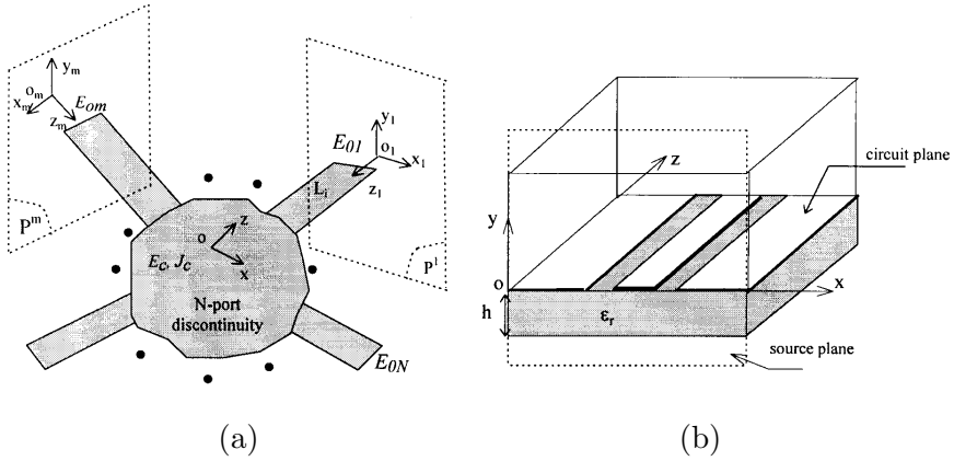
Figure 1. (a) Schematic of a multiport discontinuity. (b) transition source-line (case of a CPW)
