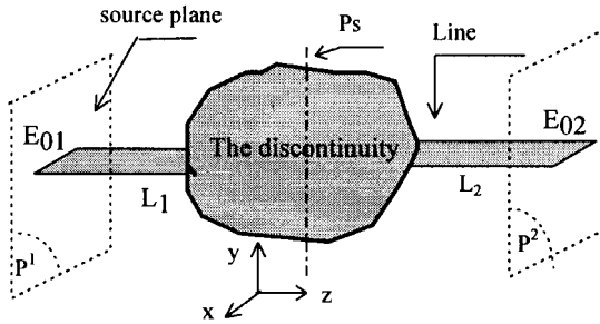
Figure 4. Schematic of 2-port discontinuity.
