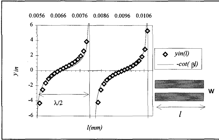
Figure 3. The input admittance y_{in} of a short circuited fin line as function of its length l ; Dimensions: gap w = 0.3 mm, substrate thickness h = 0.11 mm, \epsilon_r = 3.75 , Frequency = 80 GHz.
