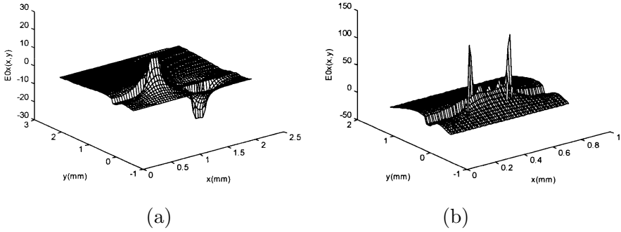
Figure 2. x -component of voltage sources. (a) Coplanar wave guide ( w = 0.9 mm, s = 0.5 mm, substrate thickness h = 0.635 mm, \varepsilon_r = 9.9 , housing WR28, F = 15 GHz) (b) Finline (gap w = 0.3 mm, substrate thickness h = 0.11 mm, \varepsilon_r = 3.75 , F = 80 GHz).
