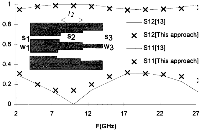
Figure 7. S -parameters of a cascaded step discontinuity in a coplanar wave guide: \lambda/4 transformer; Dimensions: \epsilon_r = 12.9 , thickness = 200\mu\text{m} , wave guide 35 ohm ( w = 20\mu\text{m} , s = 5\mu\text{m} ), wave guide 50 ohm ( w = 15\mu\text{m} , s = 10\mu\text{m} , l = 3.104\text{ mm} ), wave guide 70 ohm ( w = 8\mu\text{m} , s = 17\mu\text{m} ).
