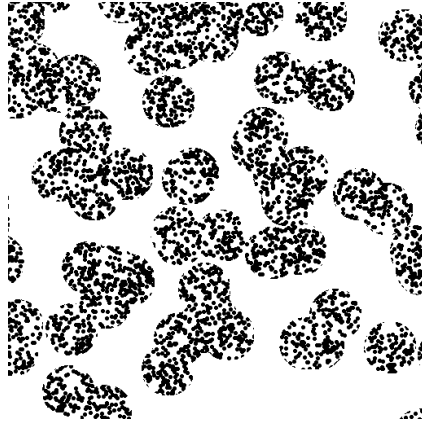
Figure 3. Simulation of a two scale model obtained in 2D by the intersection of two Boolean models of discs ( p_1 = p_2 = 0.5 ; p = 0.25 ).
