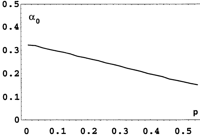
Figure 5. The dependence of the coefficient \alpha_0 in Eq. (41) for a cubic lattice of inclusions on their volume concentration p .
