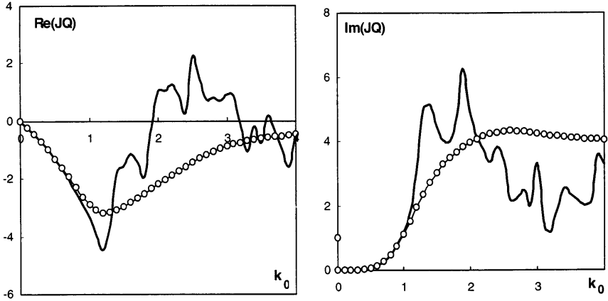
Figure 1. The dependences of the real and imaginary parts of the functional JQ on k_0 . Solid lines correspond to the exact solution of the diffraction problem (Mie's solution) for an inclusion of a unit radius ( \varepsilon_0 = 1 , \varepsilon = 5 ), the lines with dots correspond to the plane wave approximation.
