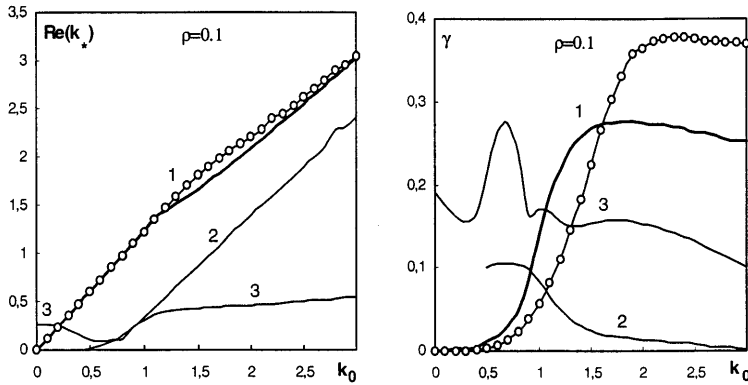
Figure 9. The disperse curves and attenuation factors for the mean wave field in the composite with the model correlation function (57) and \rho = 0.1 ( \varepsilon_0 = 1 ; \varepsilon = 5 , p = 0.2 ). Lines with dots are one scale Boolean model for p = 0.2 .
