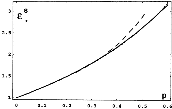
Figure 6. The dependence of the effective static dielectric permittivity \epsilon_*^s of the composite with a cubic lattice of spherical inclusions on their volume concentration p ( \epsilon = 10, \epsilon_0 = 1 ). Point line is the same dependence for isotropic distribution of inclusions (Eq. (37)); dashed line is the exact values of the effective permittivity obtained in [16].
