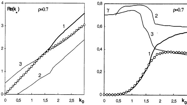
Figure 11. The same graphs as in Fig. 9, 10 for \rho = 0.7 .
