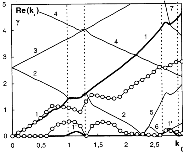
Figure 7. The dispersion curves (dependences \text{Re}[k_*(k_0)] ) and attenuation factors ( \gamma = \text{Im}[k_*(k_0)] ) of the mean wave field in the composite with a regular cubic lattice of spherical inclusions of a unit radius ( \varepsilon_0 = 1 ; \varepsilon = 5 , p = 0.3 ).
