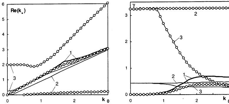
Figure 8. The dispersion curves and attenuation factors for the one scale (lines with dots) and two scale (solid lines) Boolean random sets of inclusions ( \varepsilon_0 = 1 ; \varepsilon = 5 , p = 0.2 ).
