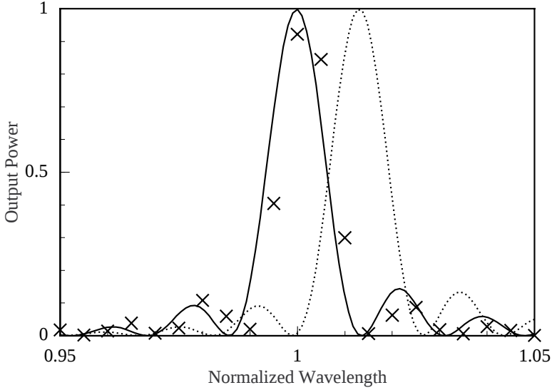
Figure 2. Comparison of the wavelength response of the output power in waveguide b at the coupling length l = 1.66 mm as the function of normalized wavelength \lambda/\lambda_0 , where d_5 - d_4 = 0.35 \mu\text{m} , d_4 - d_3 = 0.6 \mu\text{m} , d_3 - d_2 = 0.05 \mu\text{m} , d_2 - d_1 = 0.2 \mu\text{m} , n_a = n_b = 3.4 , n_s = 3.2 , n_c^2 = (n_b^2 + n_s^2)/2 , n_d^2 = (n_b^2 - n_s^2)/2 , p = 21.42 \mu\text{m} , and the center wavelength \lambda_0 = 0.83 \mu\text{m} . The solid and dotted curves are obtained by the present formulation and the improved coupled-mode theory, respectively, and the crosses are the numerical results of the Fourier series expansion method [12].
