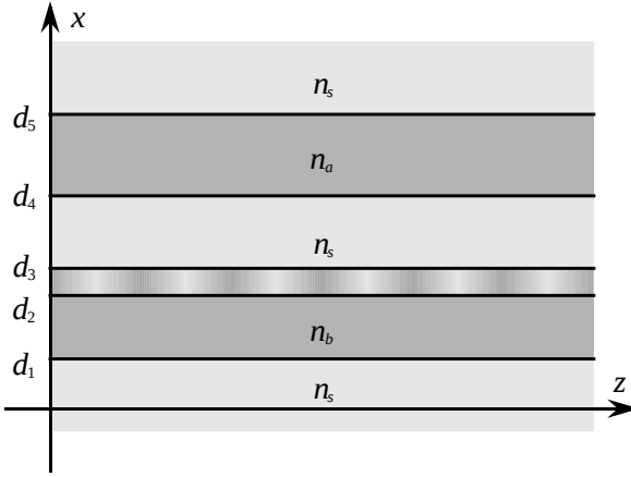
Figure 1. Geometry of the grating-assisted directional coupler.
