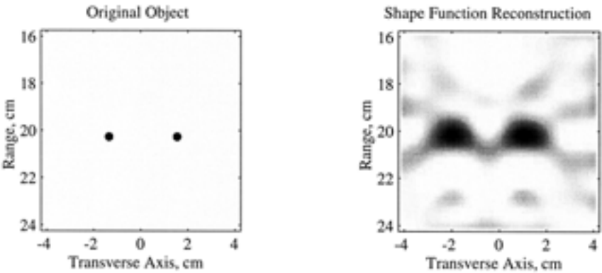
Figure 11. Original object and shape function reconstruction of two metallic cylinders of diameter 4.5 mm aligned horizontally with separation 3.2 cm .
