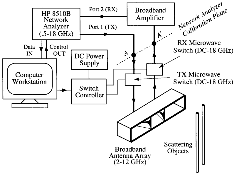
Figure 4. Block diagram of prototype step-frequency radar (SFR) broadband inverse scattering measurement system.
