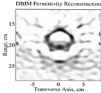
Figure 14. Reconstruction of microwave data from a hollow PVC pipe of diameter 4.8 cm in air.
