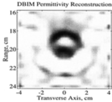
Figure 13. Reconstruction of microwave data from a hollow PVC pipe of diameter 2.7 cm in air.
