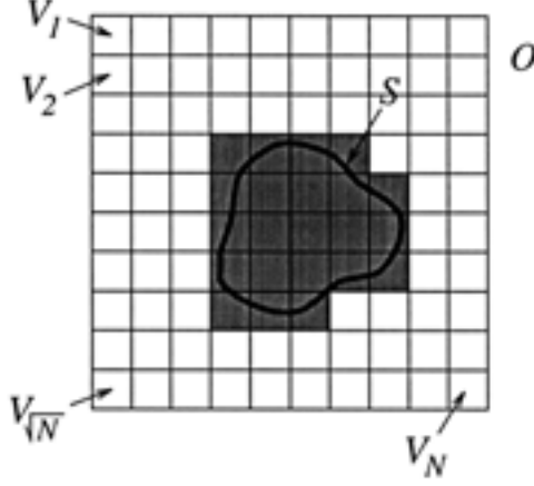
Figure 2. Discretization of scattering object volume \mathcal{O} into N subvolumes V_i , i = 1, \dots, N . Surface S indicates the metallic scatterer and the shaded region is where \gamma_i = 1 .
