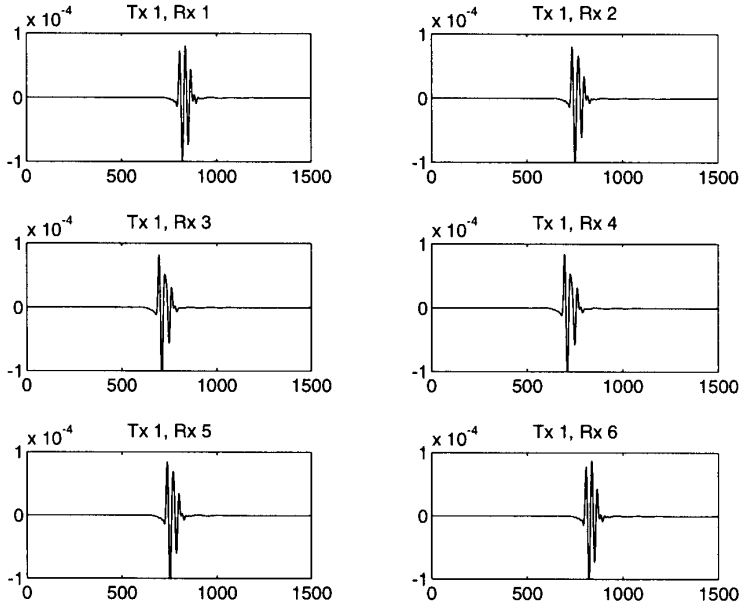
Figure 10. Scattered field computed using finite-difference time-domain for two metallic cylinders aligned vertically. Cylinders each have diameter of 4.5 mm and are separated by 3.2 cm .
