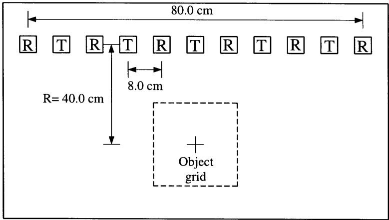
Figure 6. Arrangement of transmitters (T), receivers (R) and object grid for new switched antenna array.
