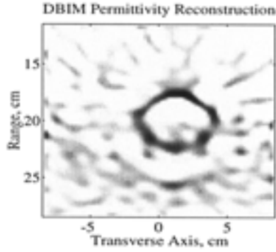
Figure 15. DBIM permittivity reconstruction of an empty glass graduated cylinder of diameter 5.25 cm located in air.
