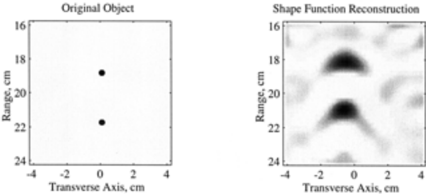
Figure 12. Original object and shape function reconstruction of two metallic cylinders of diameter 4.5 mm aligned vertically with separation 3.2 cm .
