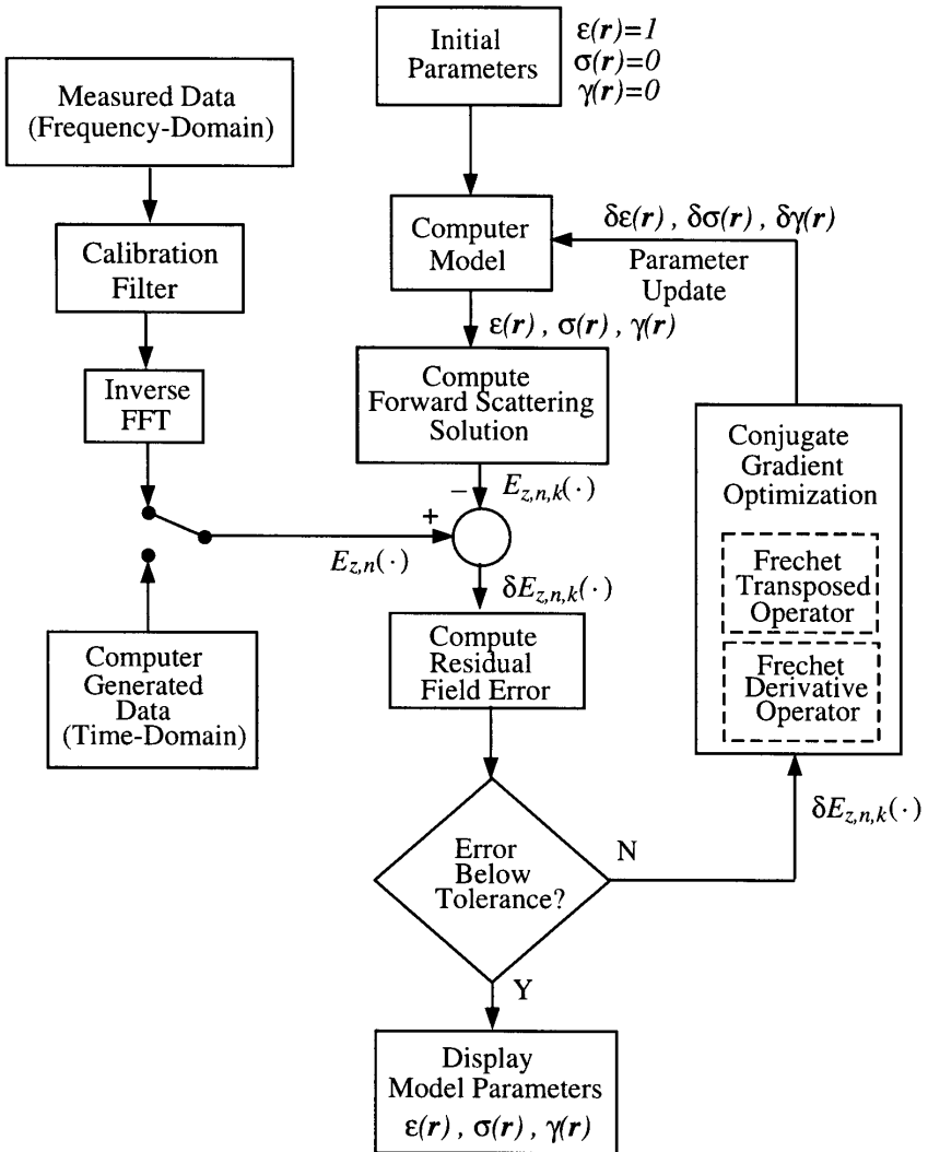
Figure 3. Block diagram of processing of measured and computer simulated scattering data.
