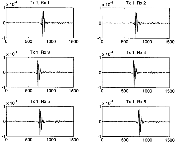
Figure 9. Calibrated time-domain scattering data for two metallic cylinders aligned vertically, obtained from the SFR measurements. Cylinders each have diameter of 4.5 mm and are separated by 3.2 cm. Data is shown for the first transmitter only and all six receivers.
