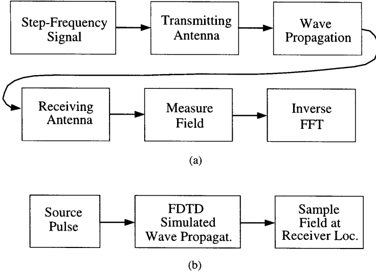
Figure 8. (a) Step-frequency radar measurement model and (b) FDTD computer model of scattering experiment.
